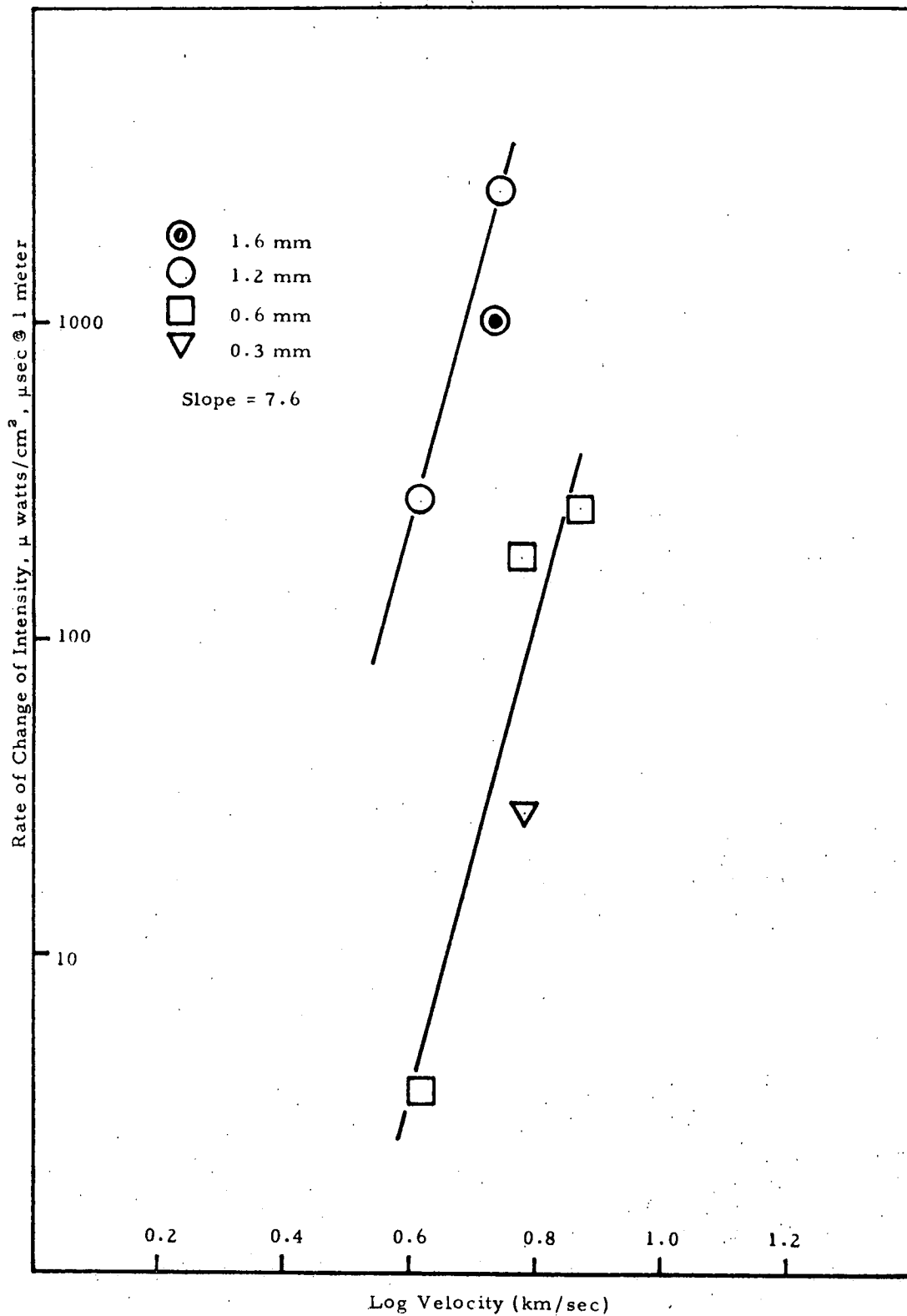
Figure 33. Spike Rate of Change of Intensity at 5085Å o for Bruderheim Projectiles Impacting Cadmium
