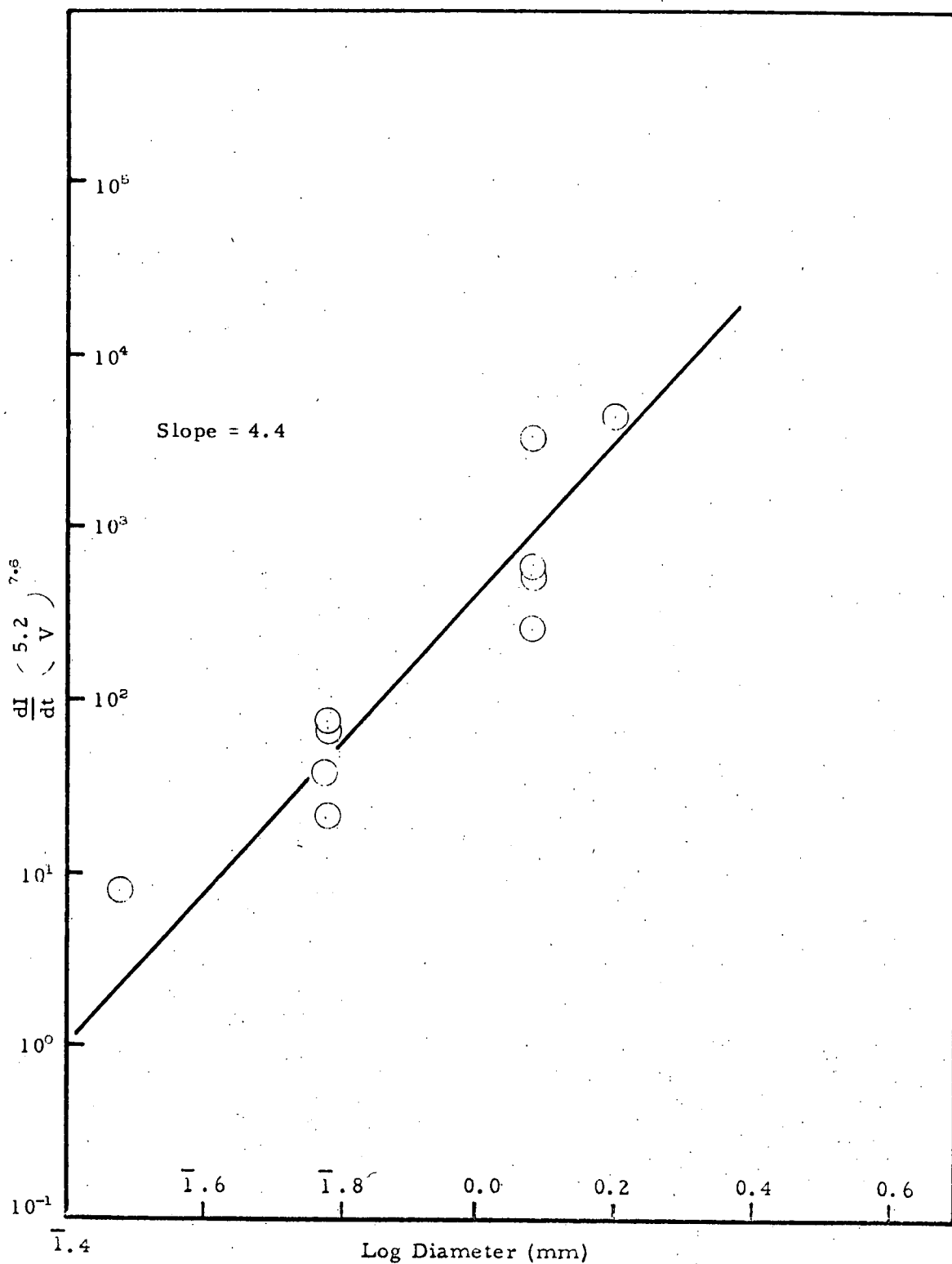
Figure 46. Dependence of dI/dt on Projectile Diameter for Bruderheim at 3610 Å
