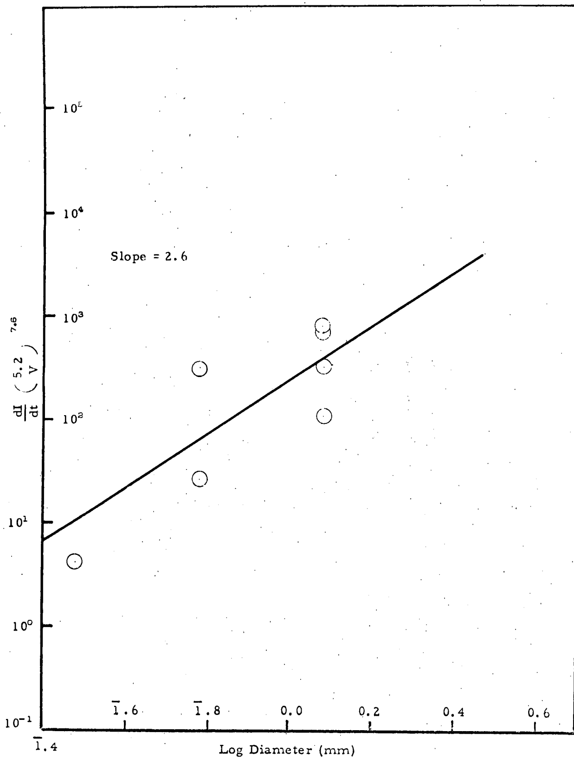
Figure 48. Dependence of dI/dt on Projectile Diameter for Bruderheim at 4900Å
