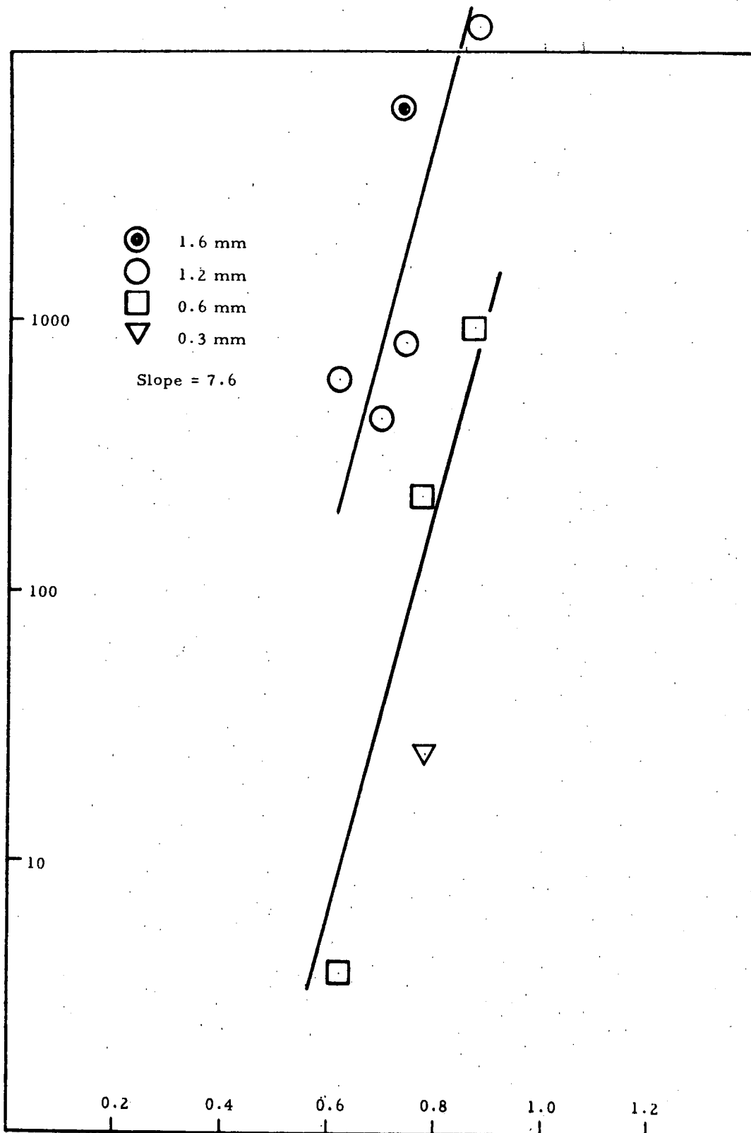
Figure 34. Spike Rate of Change of Intensity at 3610Å o for Bruderheim Projectiles Impacting Cadmium
