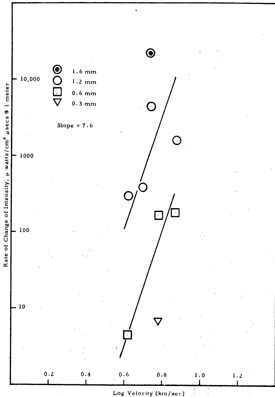
Figure 32. Spike Rate of Change of Intensity at 3261Å for Bruderheim Projectiles Impacting Cadmium
