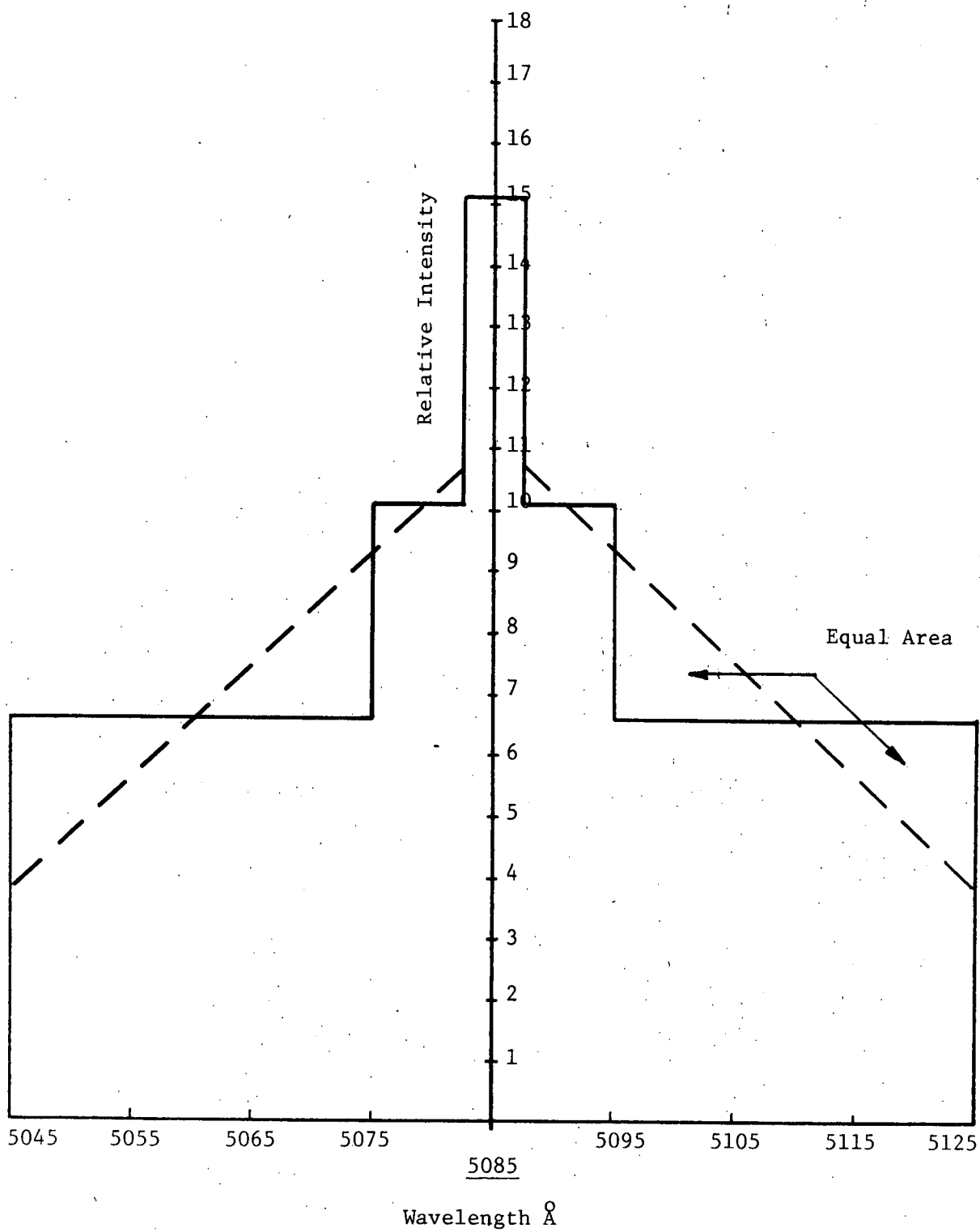
Figure 2. Spectral Distribution Around 5085 0 Å Line
