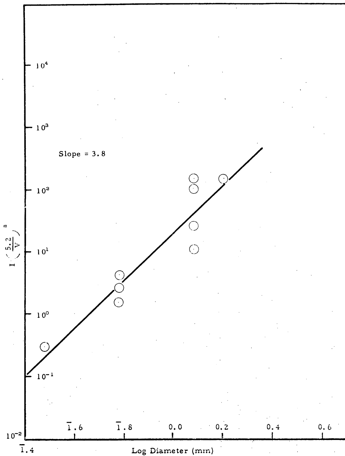
Figure 47. Dependence of Intensity on Projectile Diameter for Bruderheim at 3610 Å
