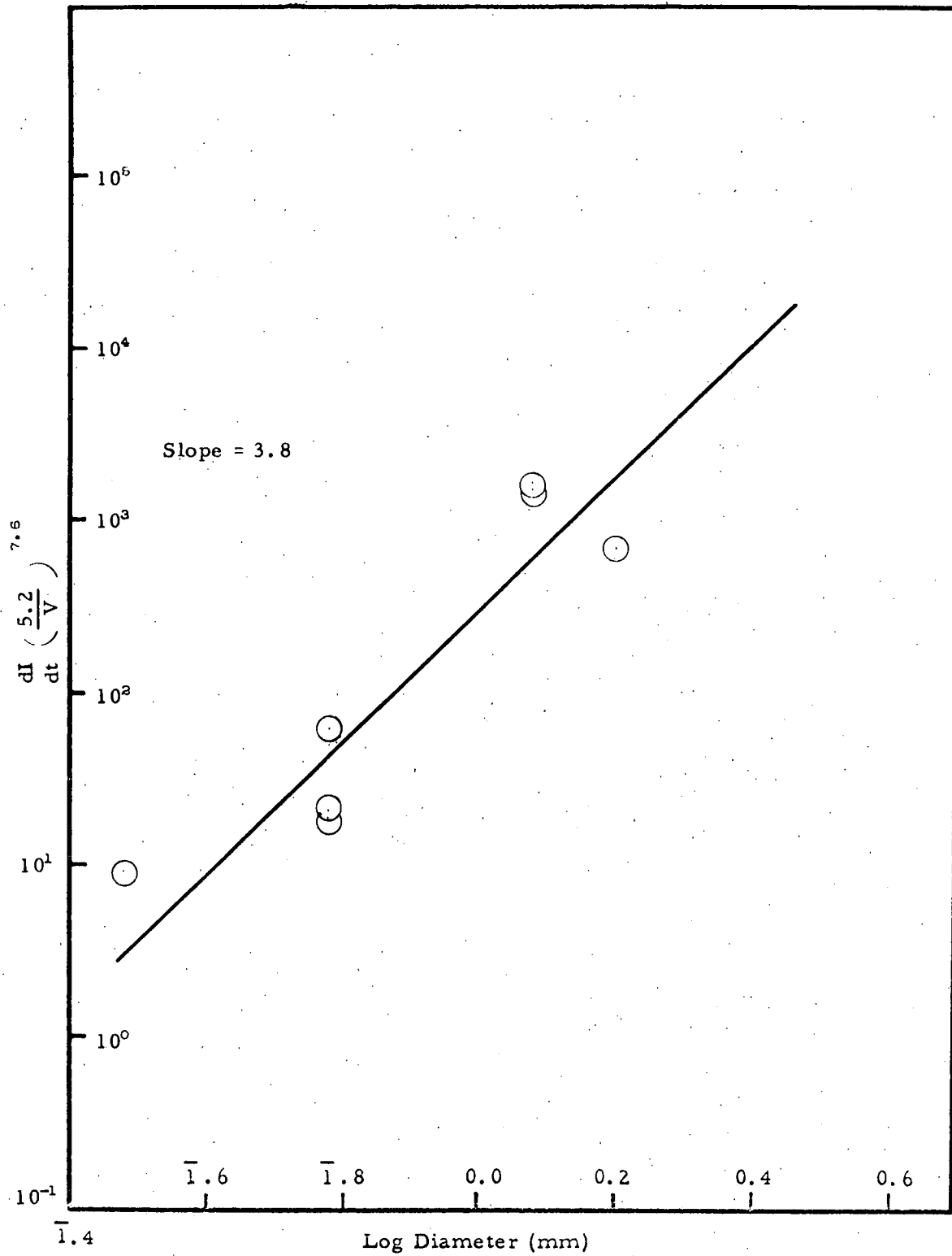
Figure 44. Dependence of dI/dt on Projectile Diameter for Bruderheim at 5085Å
