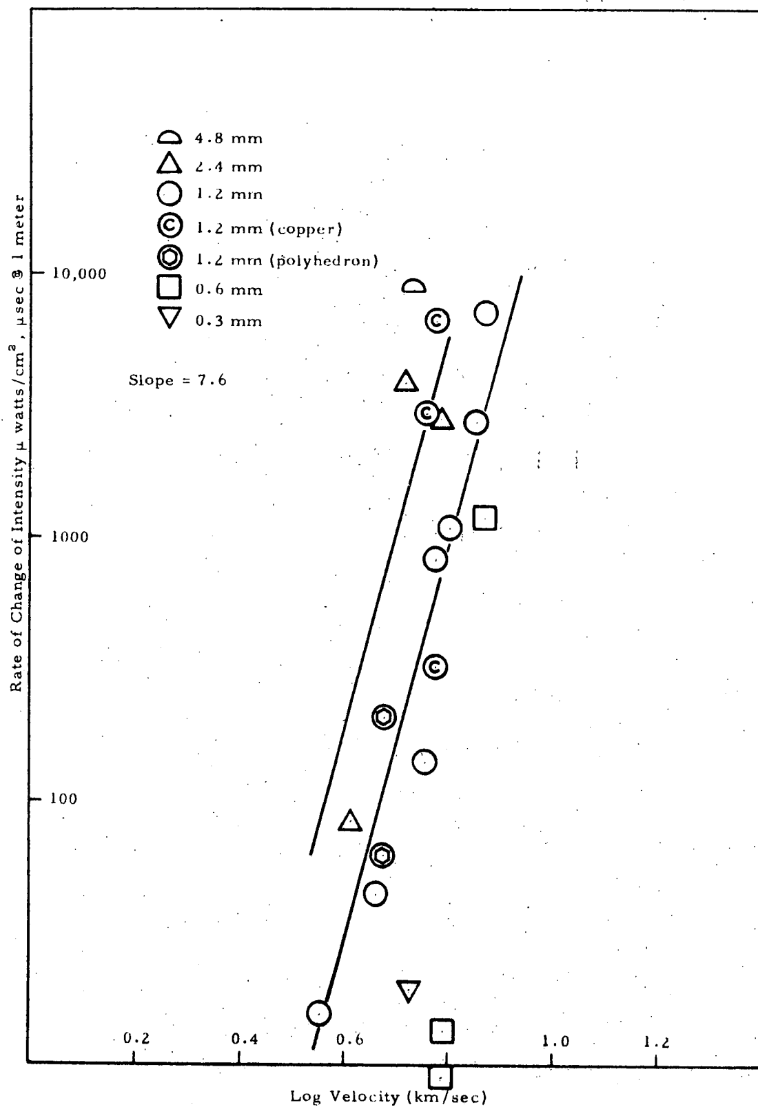
Figure 28. Spike Rate of Change of Intensity at 3261\text{\AA} for CanDi and Copper Projectiles Impacting Cadmium
