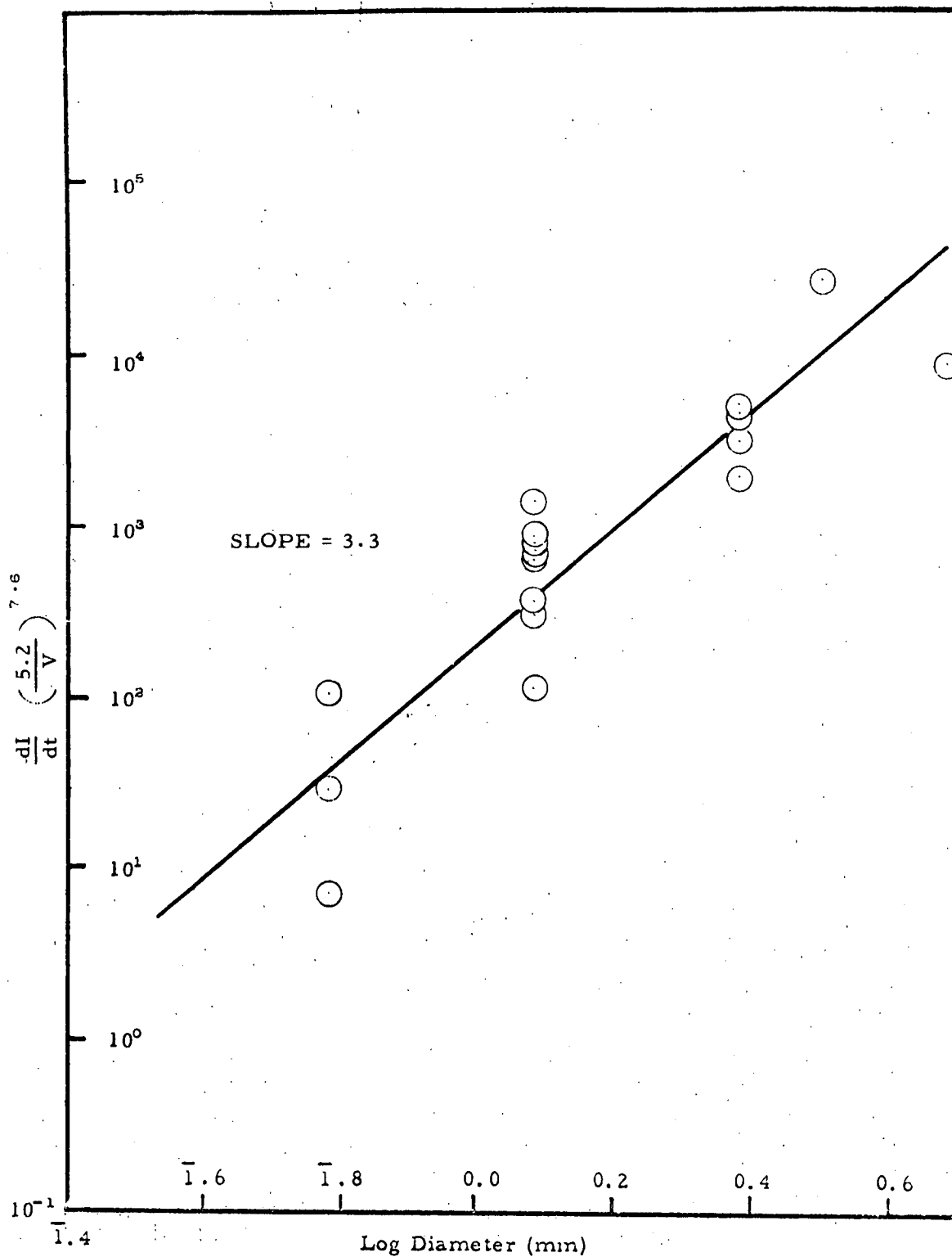
Figure 41. Dependence of dI/dt on Projectile Diameter for Canyon Diablo at 3610Å
