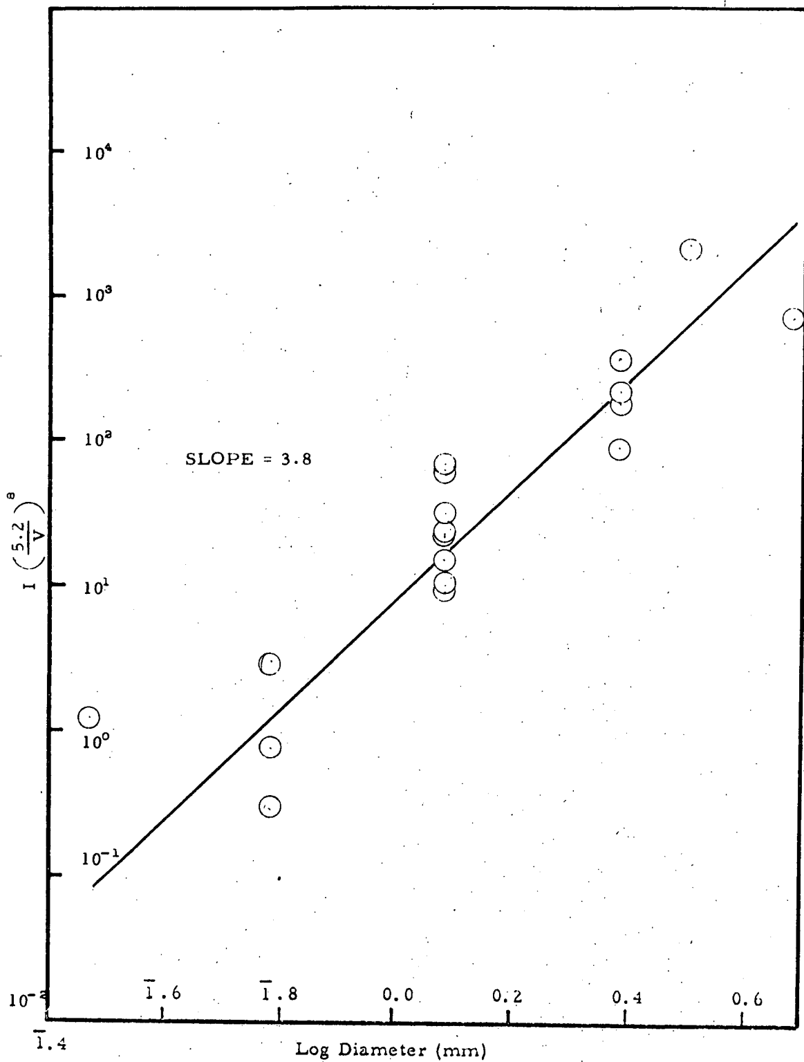
Figure 37. Dependence of Intensity on Projectile Diameter for Canyon Diablo at 3610 Å
