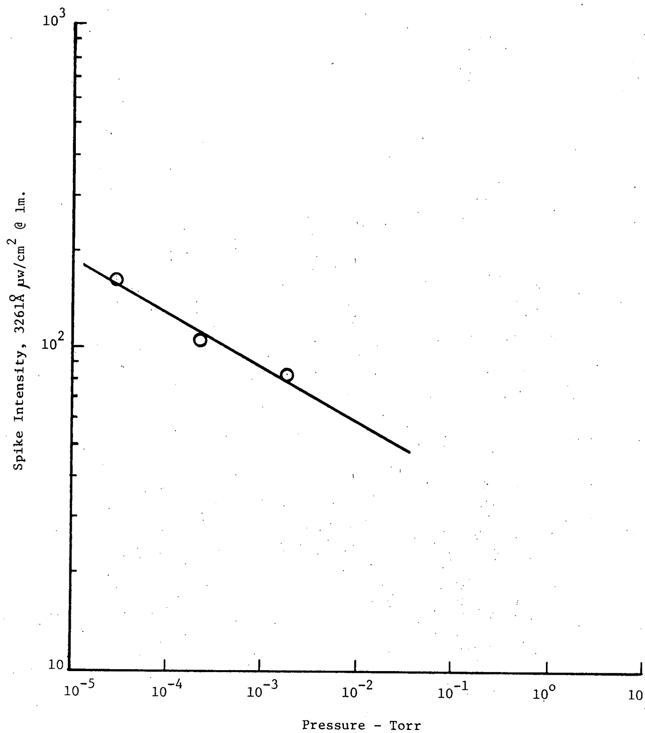
Figure 18. Pressure Dependence of Spike Intensity, 3261 Å
