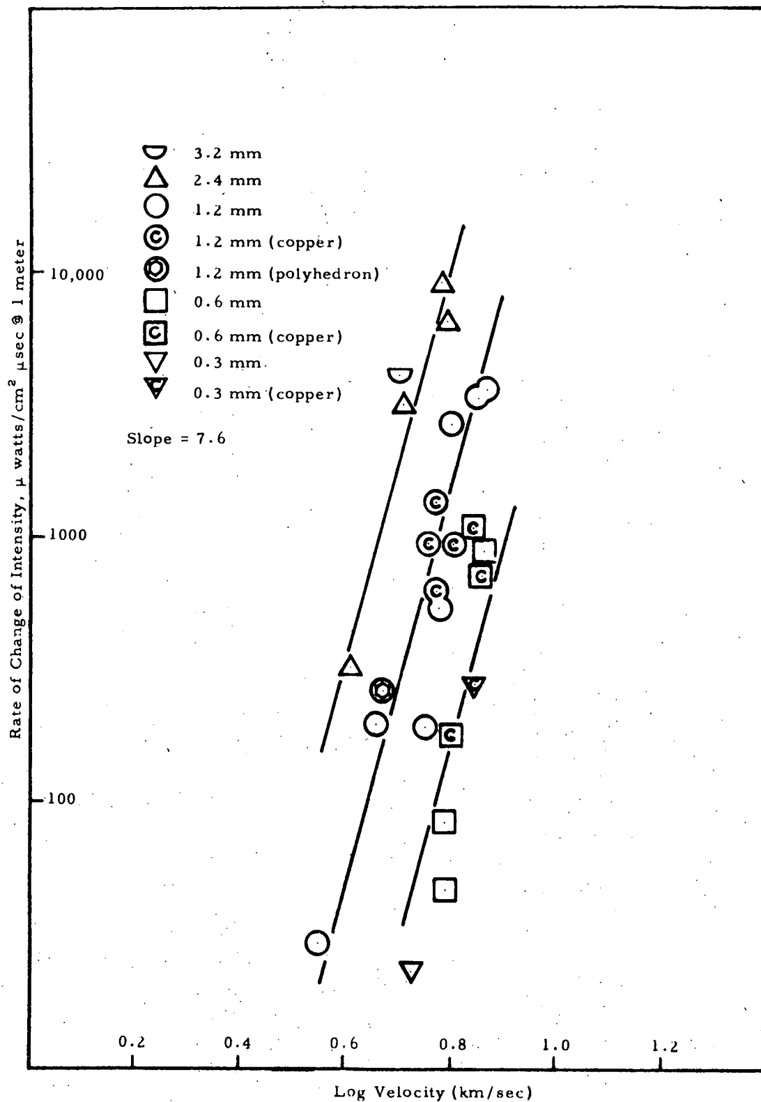
Figure 29. Spike Rate of Change of Intensity at 5085Å 0 for CanDi and Copper Projectiles Impacting Cadmium
