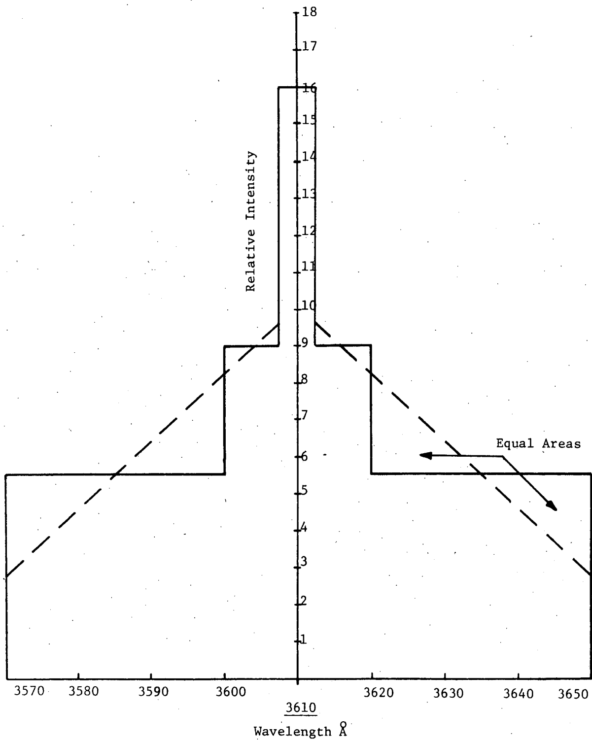
Figure 1. Spectral Distribution Around 3610 0 Å Line
