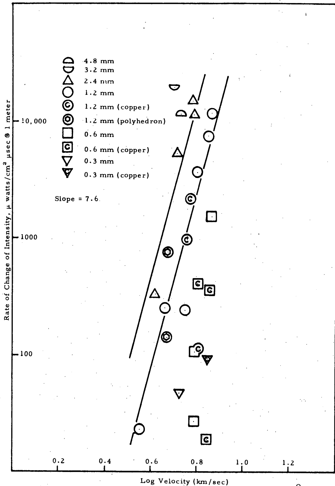
Figure 30. Spike Rate of Change of Intensity at 3610Å o for CanDi and Copper Projectiles Impacting Cadmium
