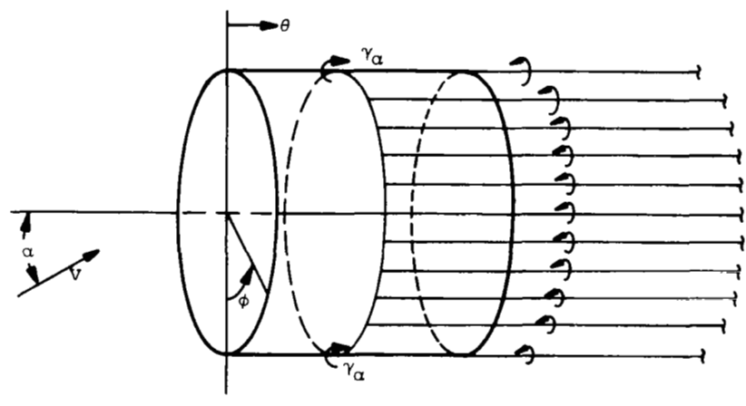
(b) Duct at angle of attack.
