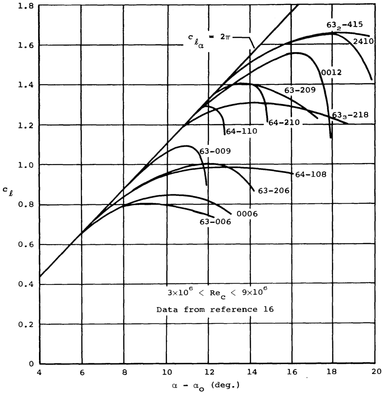
(a) Section data.
