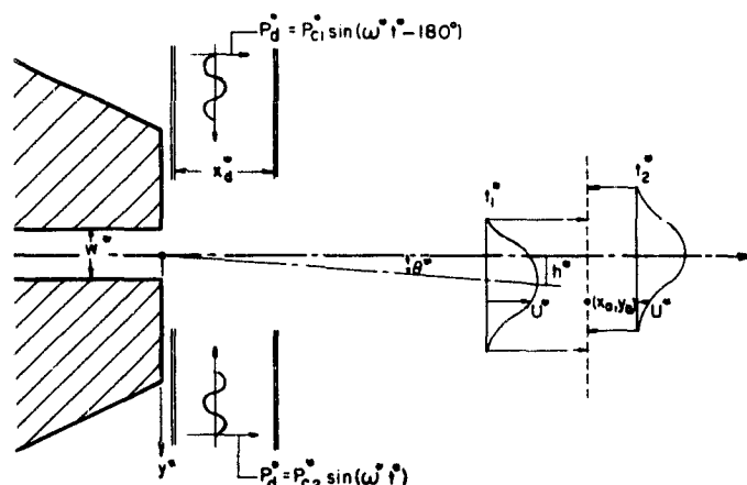
Fig. 14 Representation of Perturbed Mean Velocity Profiles
