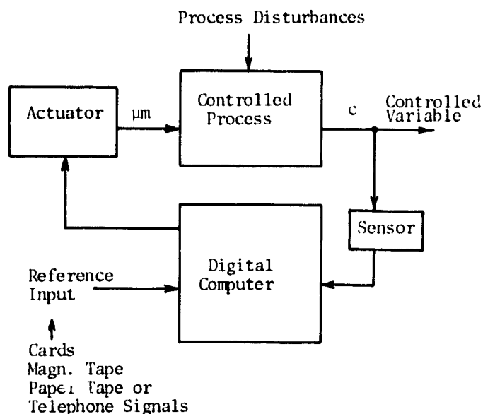
Fig. 30 Block Diagram for the Proposed Control Method
