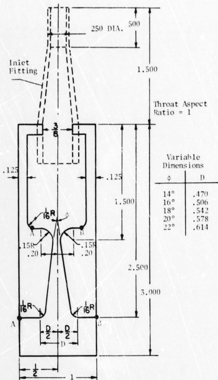
Fig. 2 Dimensions of the Small Diffuser Test Models
