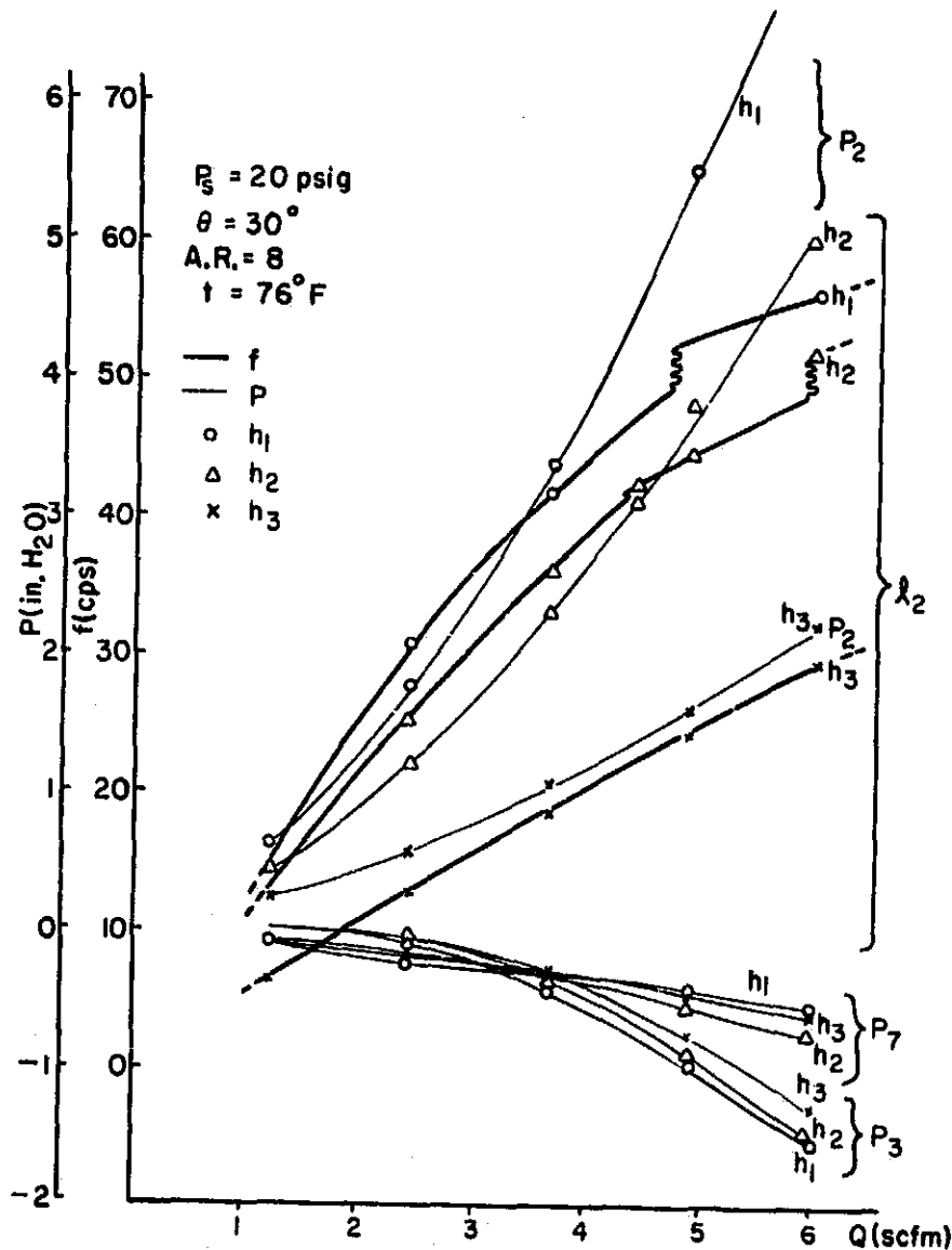
Fig. 12a Influence of Vane Height -- Case I, \lambda_1
