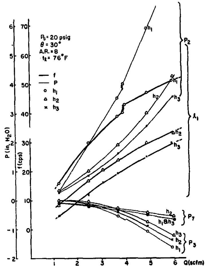
Fig. 12c Influence of Vane Height -- Case I, l_3
