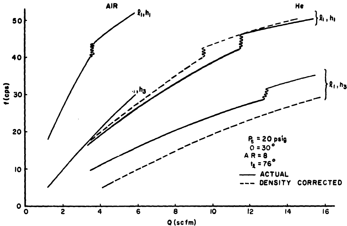
Fig. 13a Influence of Gas Density -- Case I, Q
