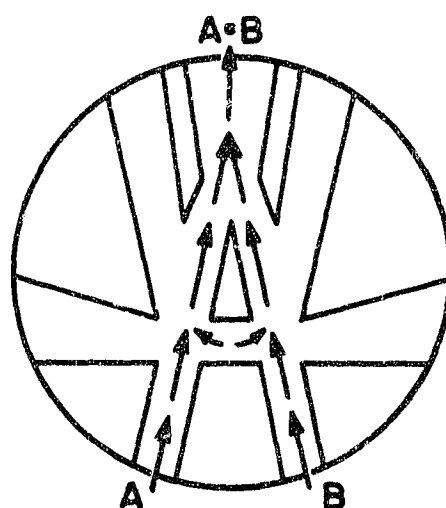
Figure 6. Fluoric AND unit operation.
