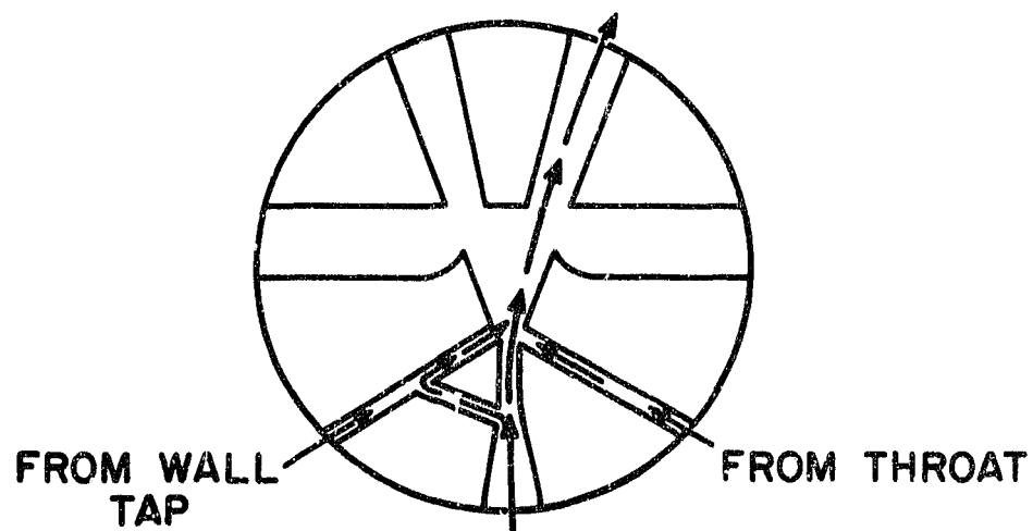
(C) INPUT PRESSURE GREATER THAN REFERENCE
