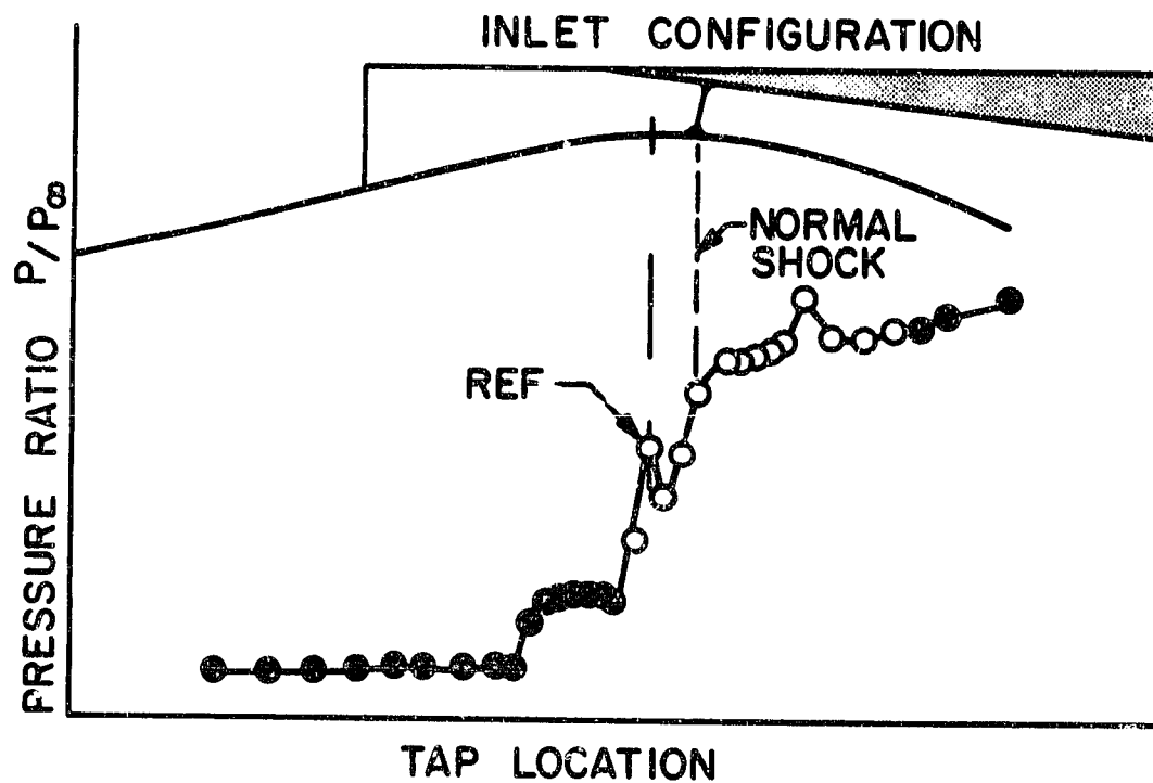
Figure 13. Wall pressure distribution, showing computed normal shock position for M_\infty = 2.5 . (Pressure distribution taken from NASA report TND-4557, fig. 23, "Investigation of a Nearly Isentropic Mixed Compression Axisymmetric Inlet System at Mach Numbers 0.6 to 3.2," by Smeltzer, Donald B., et al. )
