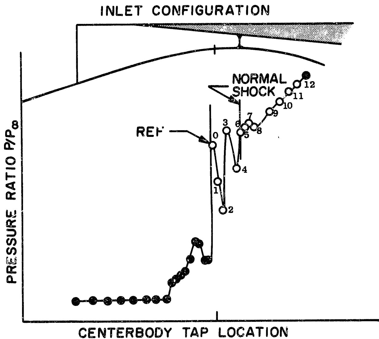
Figure 11. Wall pressure distribution, showing computed normal shock position for M_\infty = 3.0 . (Pressure distribution taken from NASA report TND-4557, fig. 20, "Investigation of a Nearly Isentropic Mixed Compression Axisymmetric Inlet System at Mach Numbers 0.6 to 3.2," by Smeltzer, Donald B., et al. )
