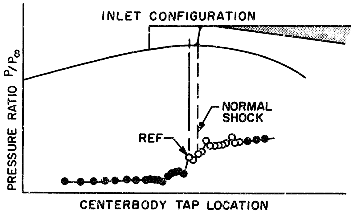
Figure 12. Wall pressure distribution, showing computed shock position for M_\infty = 2.25 . (Pressure distribution taken from fig. 25, "Investigation of a Nearly Isentropic Mixed Compression Axisymmetric Inlet System at Mach Numbers 0.6 to 3.2," by Smeltzer, Donald B., et al. )
