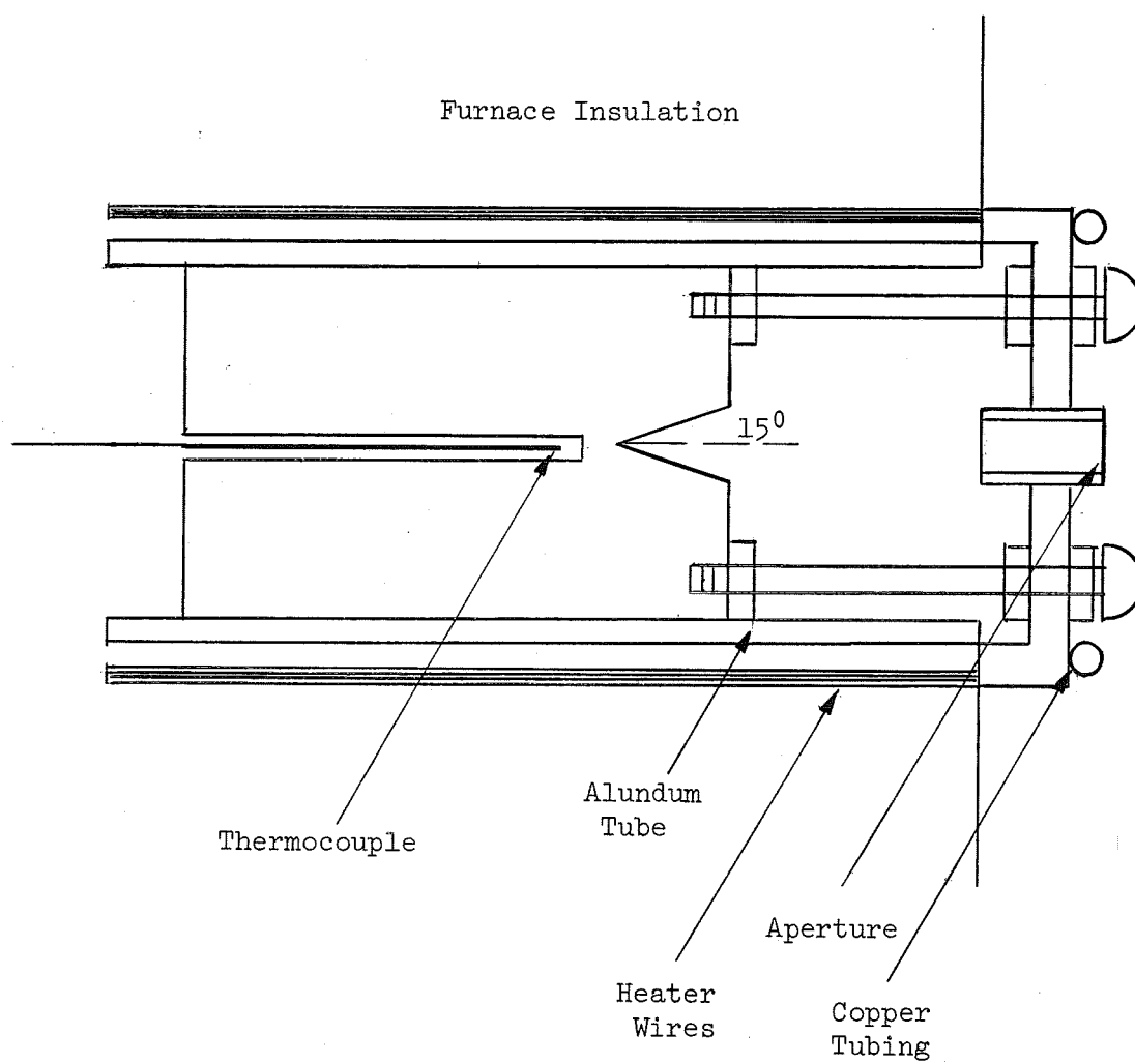
Figure 3.4 A Cut-Away View of the Black Body Source
