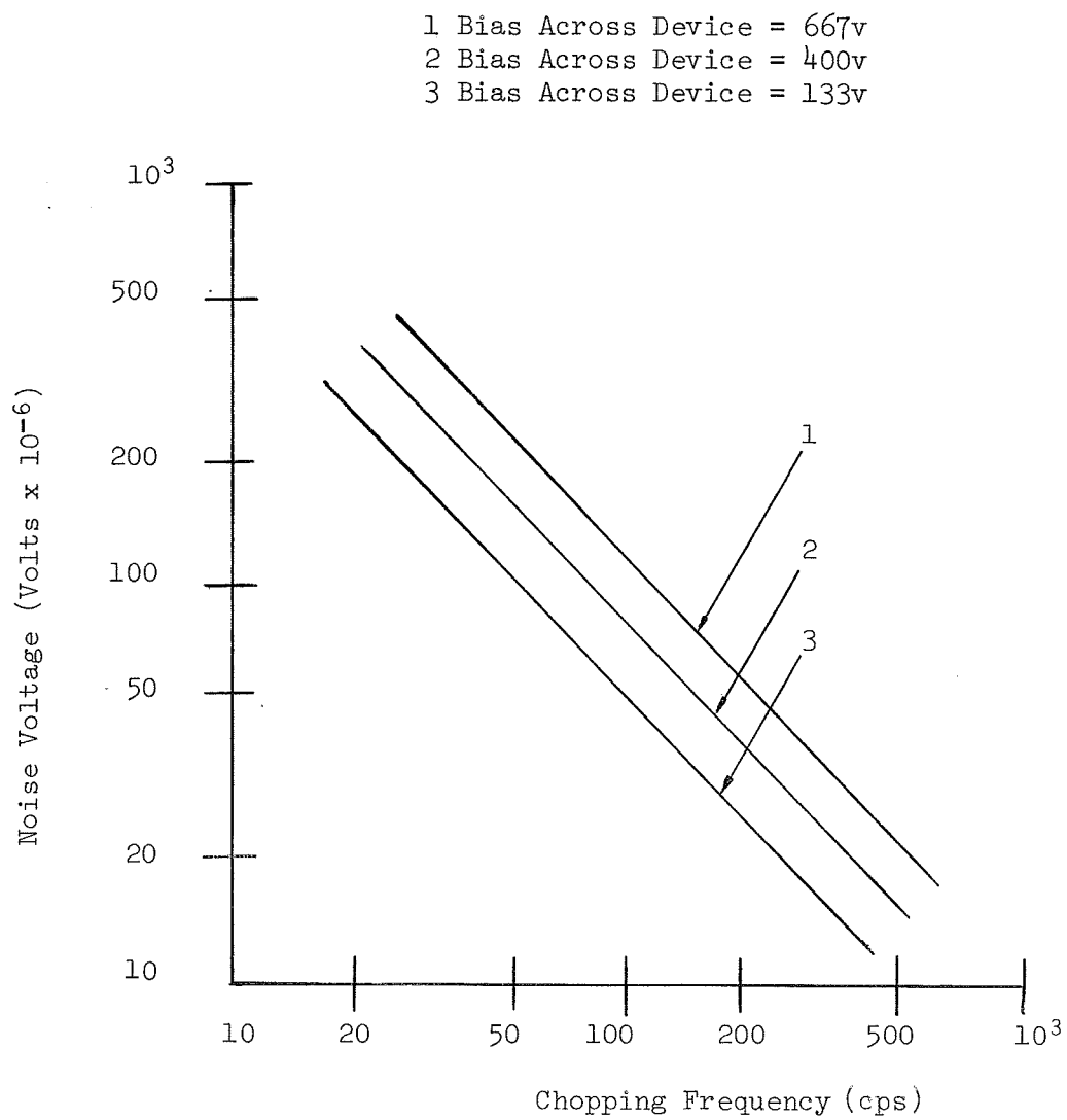
Figure 4.11 A Typical Noise Root Power Spectrum (Device S-12-N.4)
