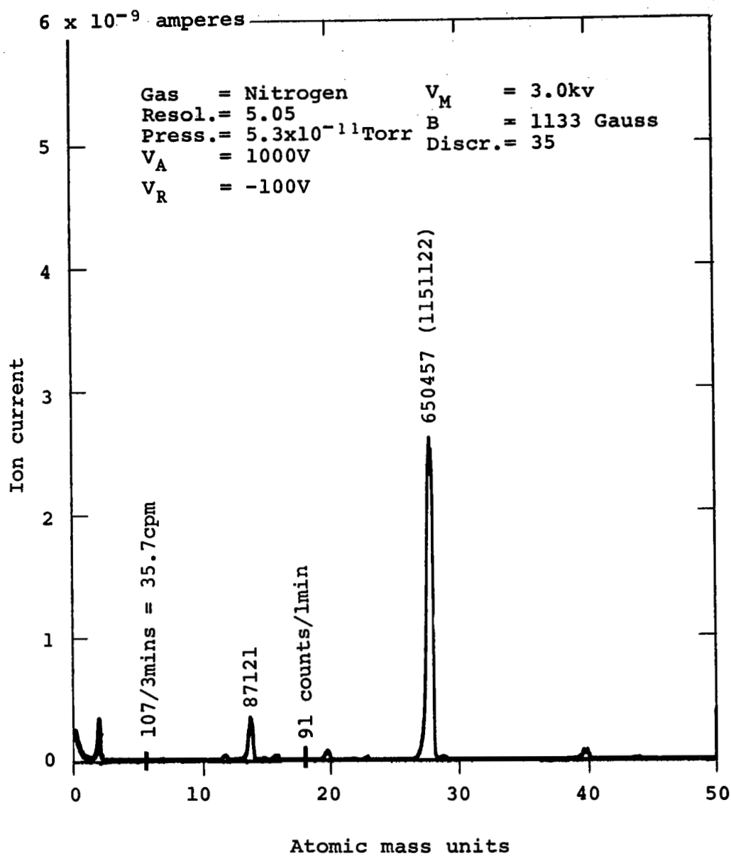
Figure 30.- Spectrum of "Single" species - nitrogen
