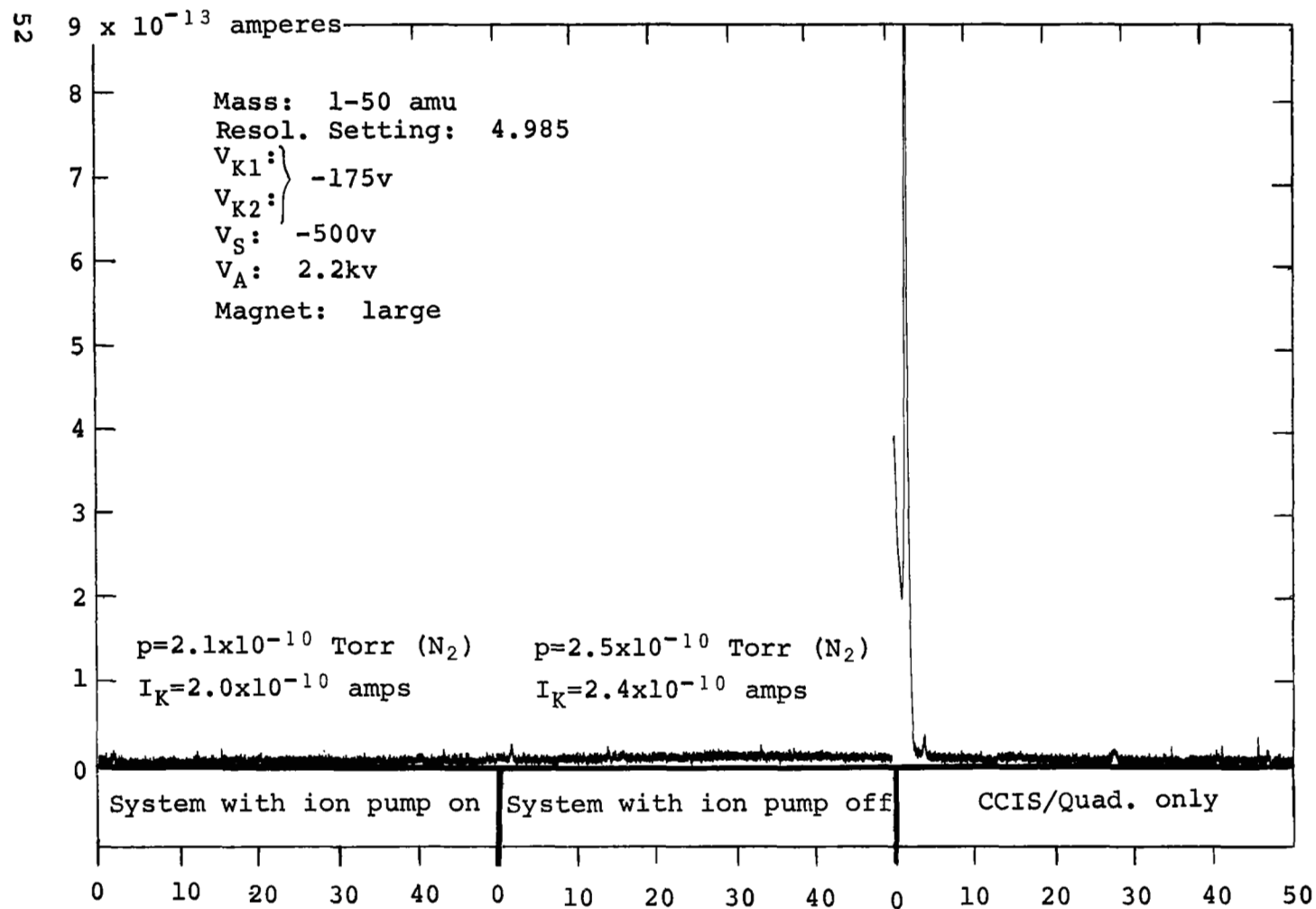
Figure 12.- Background spectra from CCIS/Quadrupole
