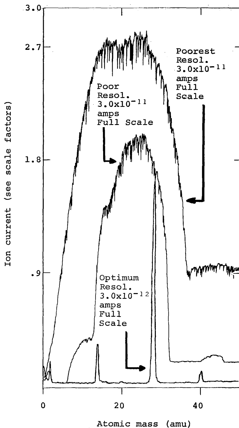
Figure 15.- Sensitivity vs. resolution- low mass range
