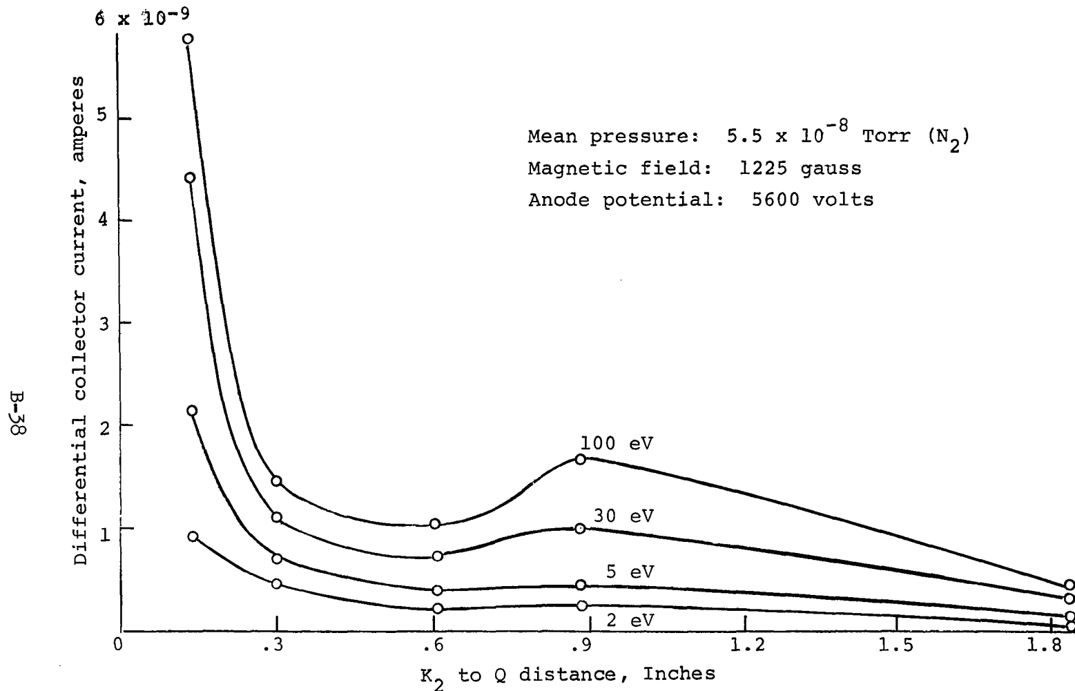
Figure B-12.- Differential collector current vs. distance for selected energy intervals, for V_{K1} = zero volts
