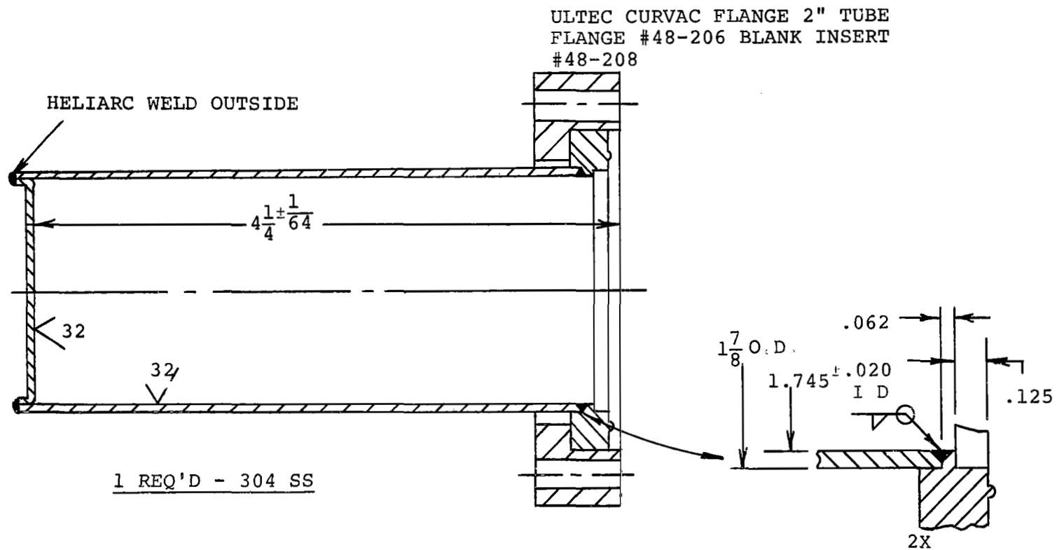
Fig. 51 CCIS Housing
