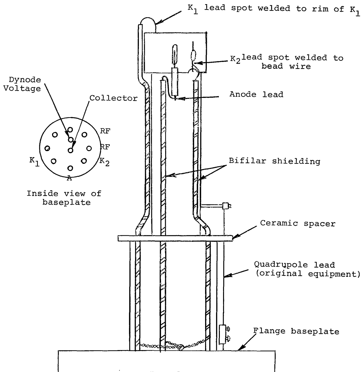
Figure 38 - Lead Assembly
