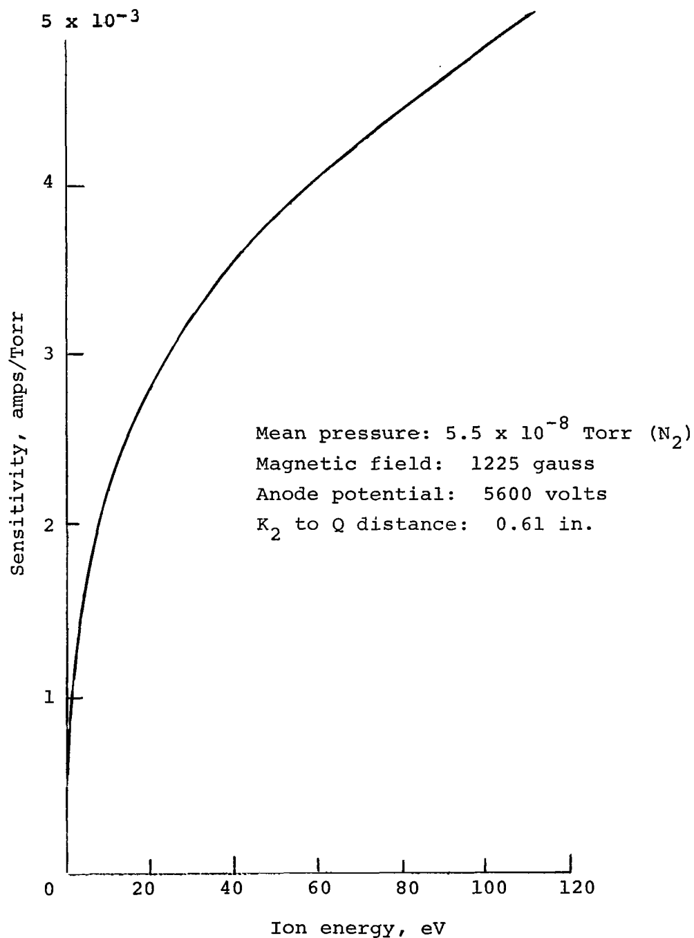
Figure B-10.— Sensitivity vs integral ion energy at 0.61 inches, for V_{K1} at +40 volts
