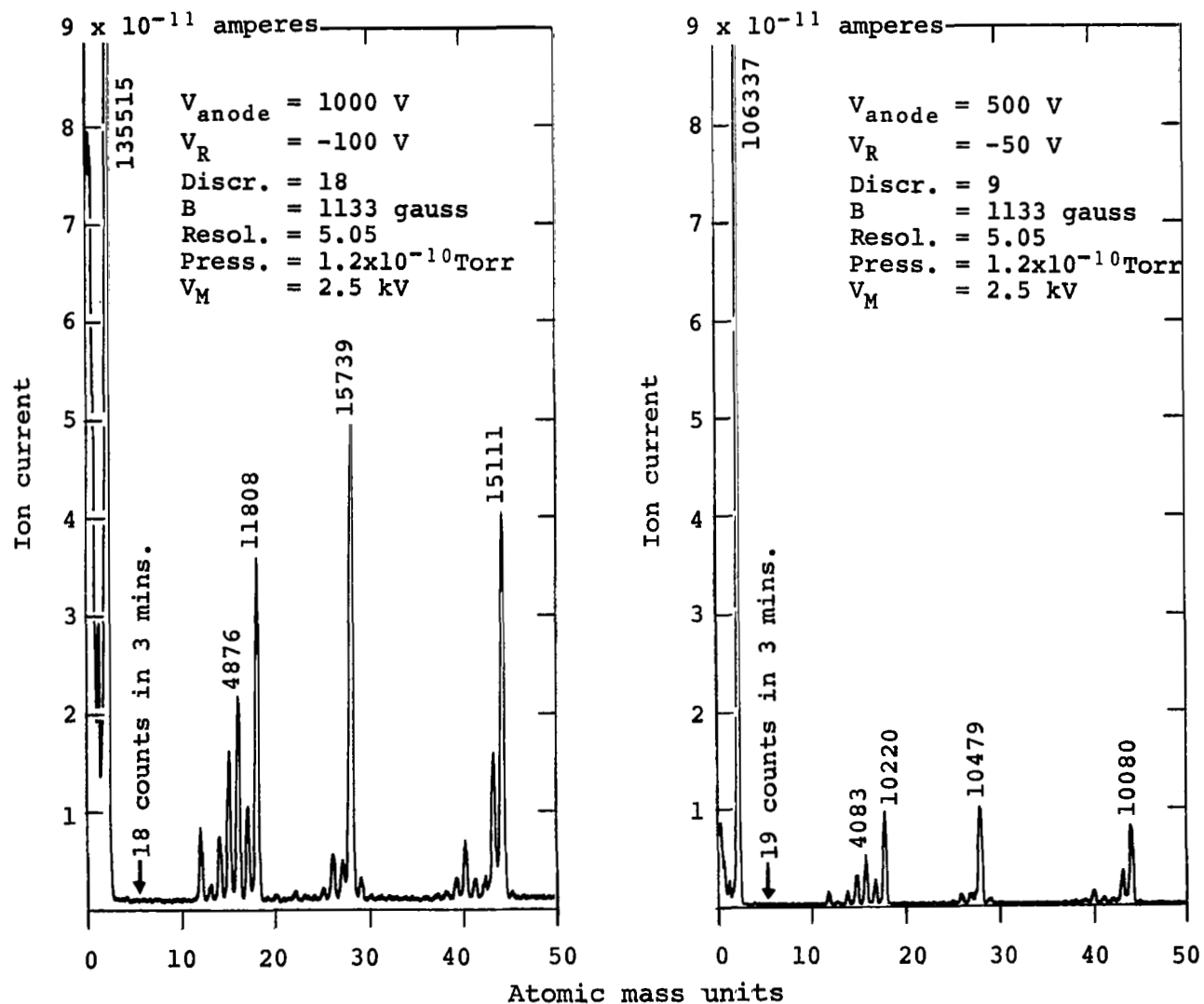
Figure 26.- Background spectra for two anode voltages (at same noise level)
