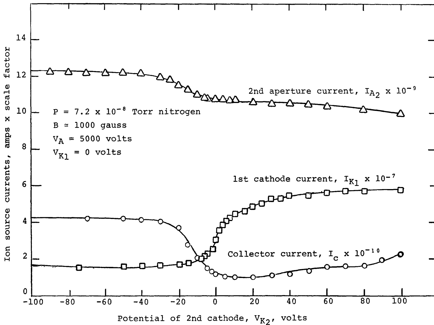
Figure A-7. - Ion extraction data - Method I - V_{K2} negative
