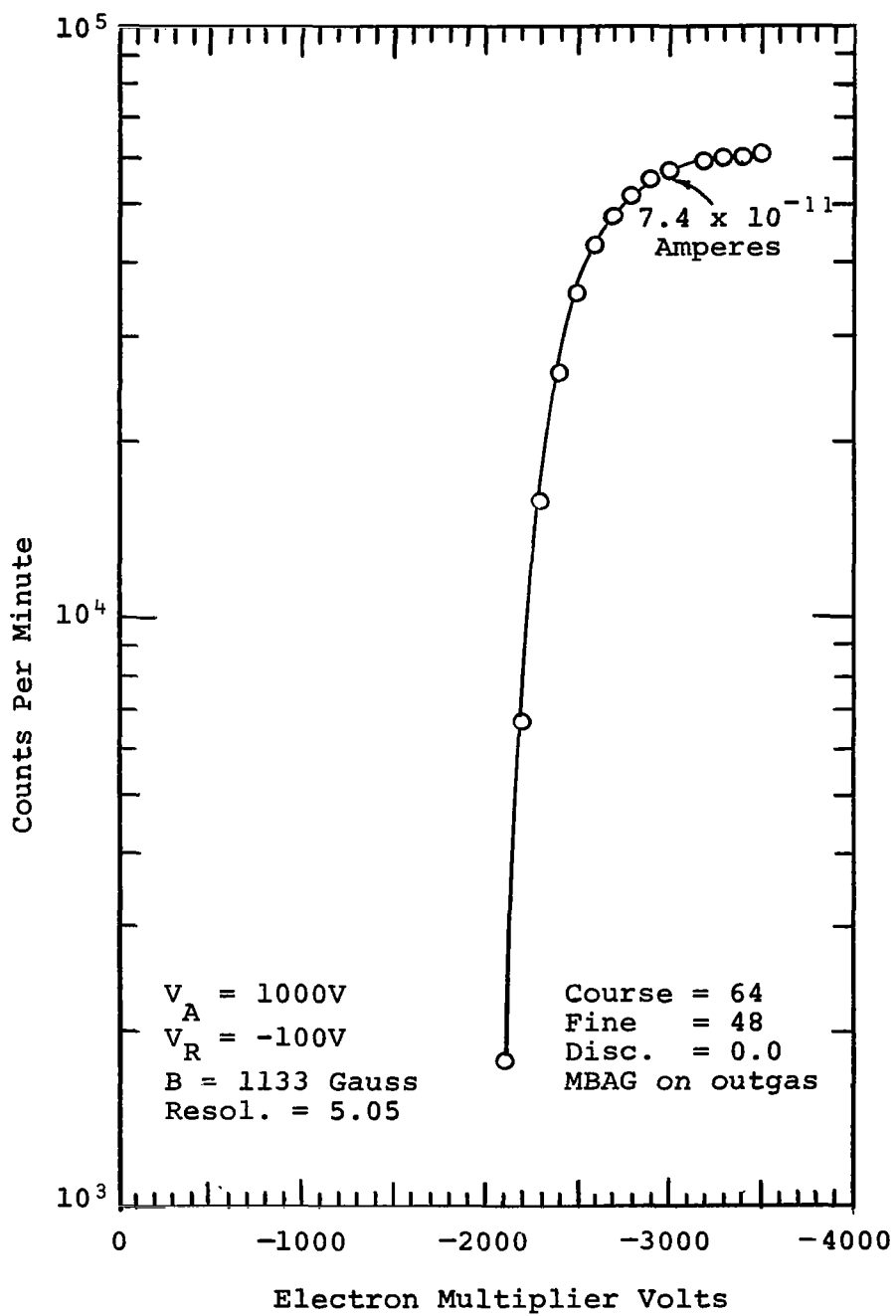
Fig. 32 Mass 28 Counting Rate vs. Multiplier Voltage
