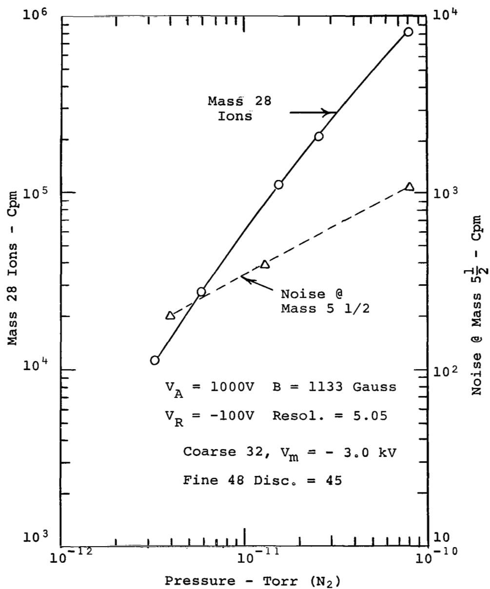
Fig. 29 Signal & Noise vs. Pressure.
