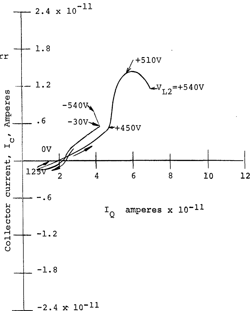
Figure B-17.- Effect of lens potential variations on I_C and I_Q at position 2 for V_{K1} = zero volts
