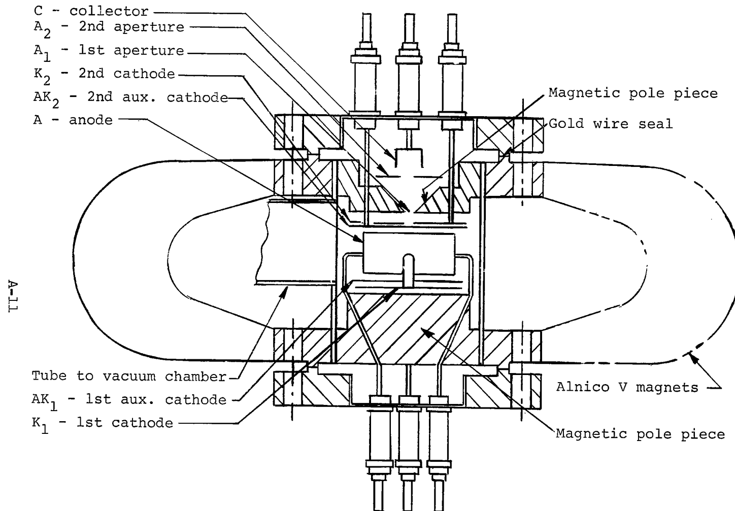
Figure A-1.- Normal Magnetron Cold Cathode Ion Source
