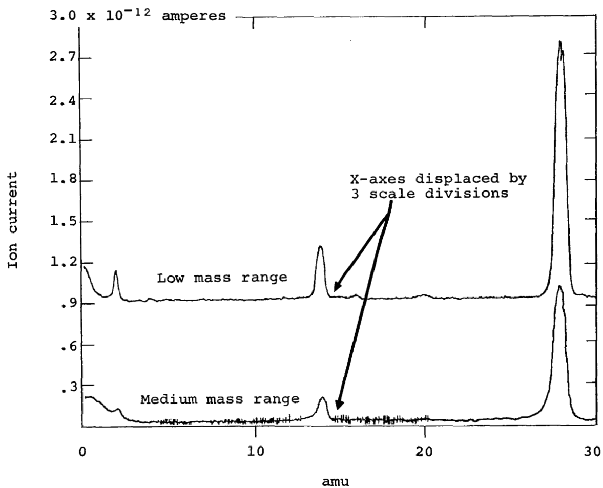
Figure 10.- Performance of CCIS/Quadrupole spectrometer on two mass ranges
