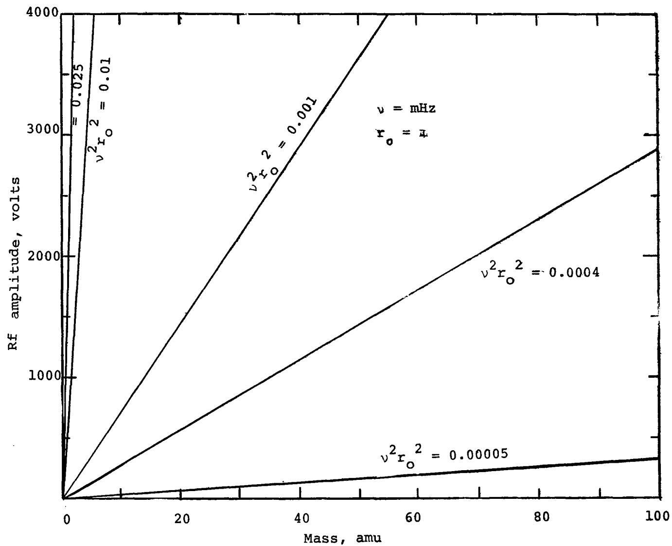
Figure A-13.- Rf amplitude vs. mass of ion
