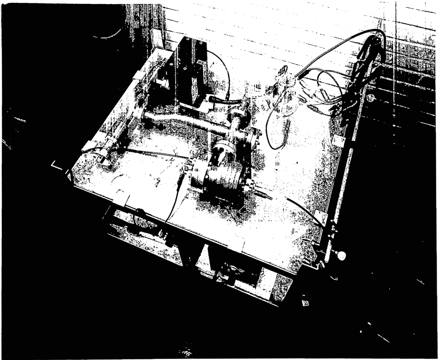
Figure B-6 View of the Upper Manifold Portion of the Vacuum System
