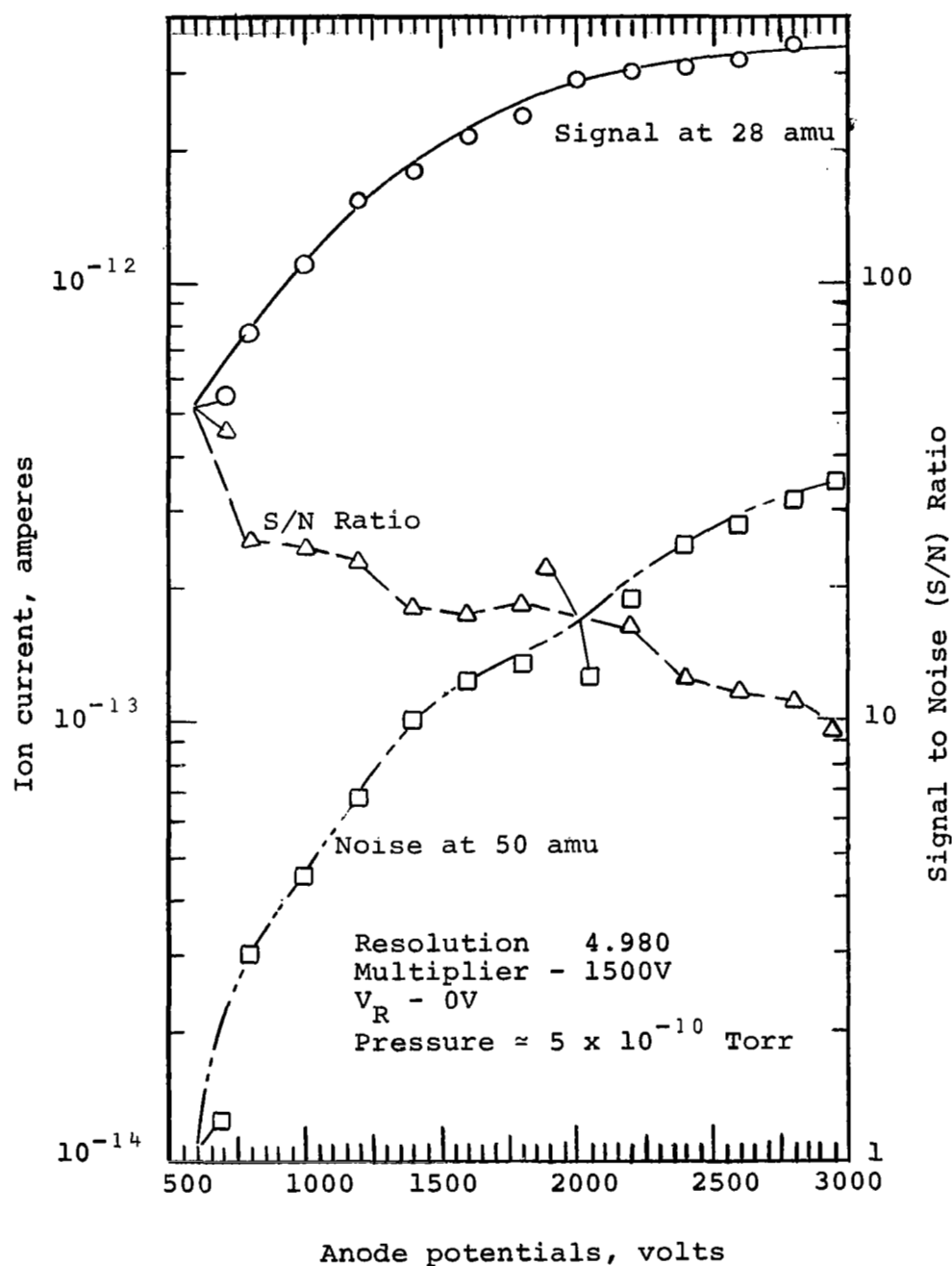
Fig. 18 - DC S/N Ratio vs. Anode Voltage
