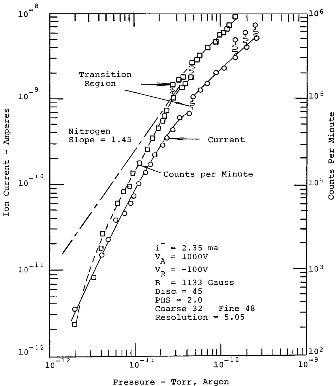
Fig. 34 Dc & Counting Rate Calibration for Argon
