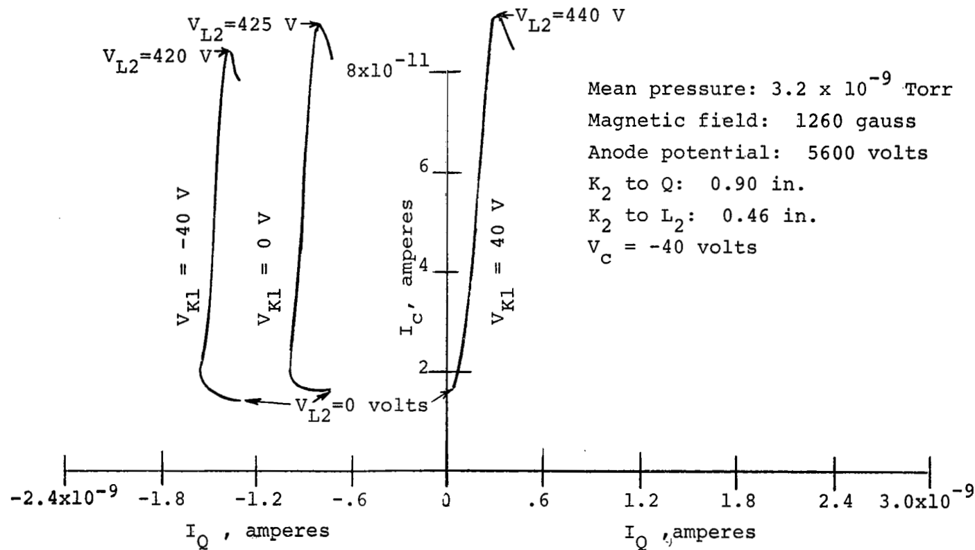
Figure B-18.- Effect of lens potential variations on I_c and I_Q at position 3, for V_{K1} = +40, \text{ Zero and } -40 volts
