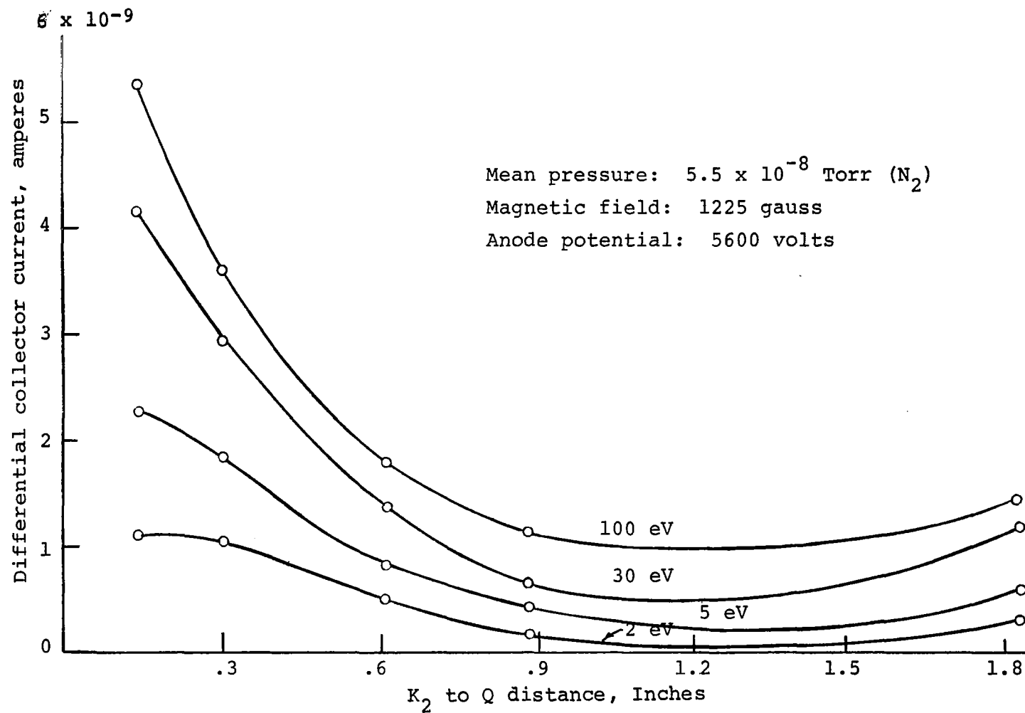
Figure B-13.- Differential collector current vs. distance for selected energy intervals, for V_{K1} = -40 volts
