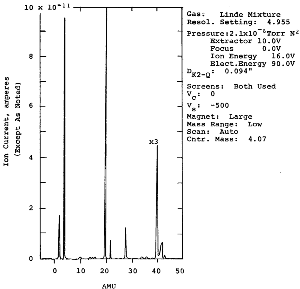
Fig. 1 Low Mass Range Spectrum Taken with the Hot Filament Spectrometer.
