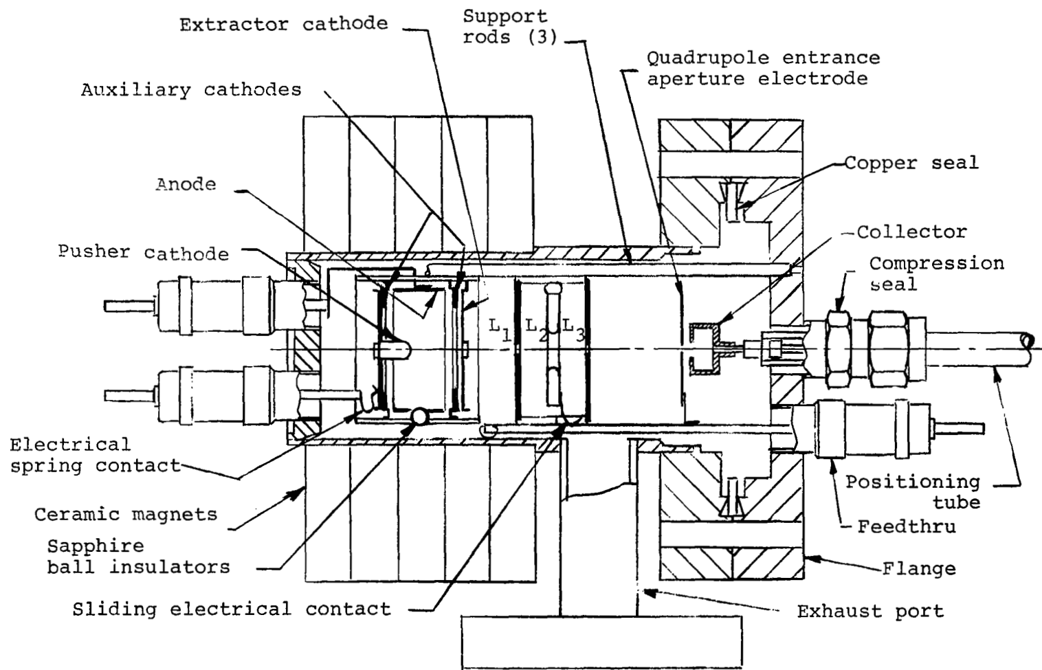
Figure B-2.- Cold cathode ion source
