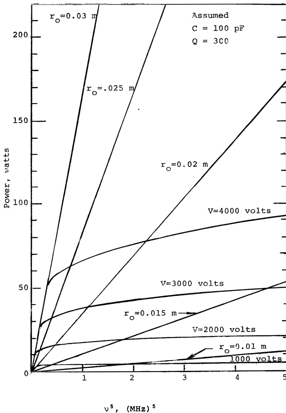
Figure A-14.- Maximum power Required for mass 100 a.m.u. ions vs. fifth power of frequency
