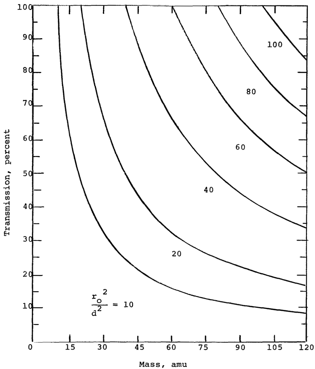
Figure A-17.- Transmission of mass filter vs. mass of ion
