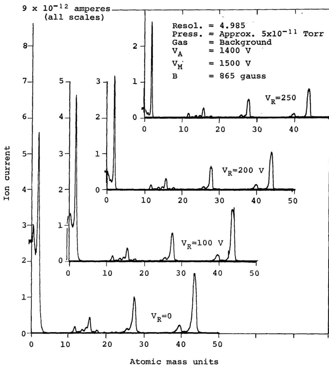
Figure 20.- DC signal and noise vs. retarding potential with tubular cathode stub
