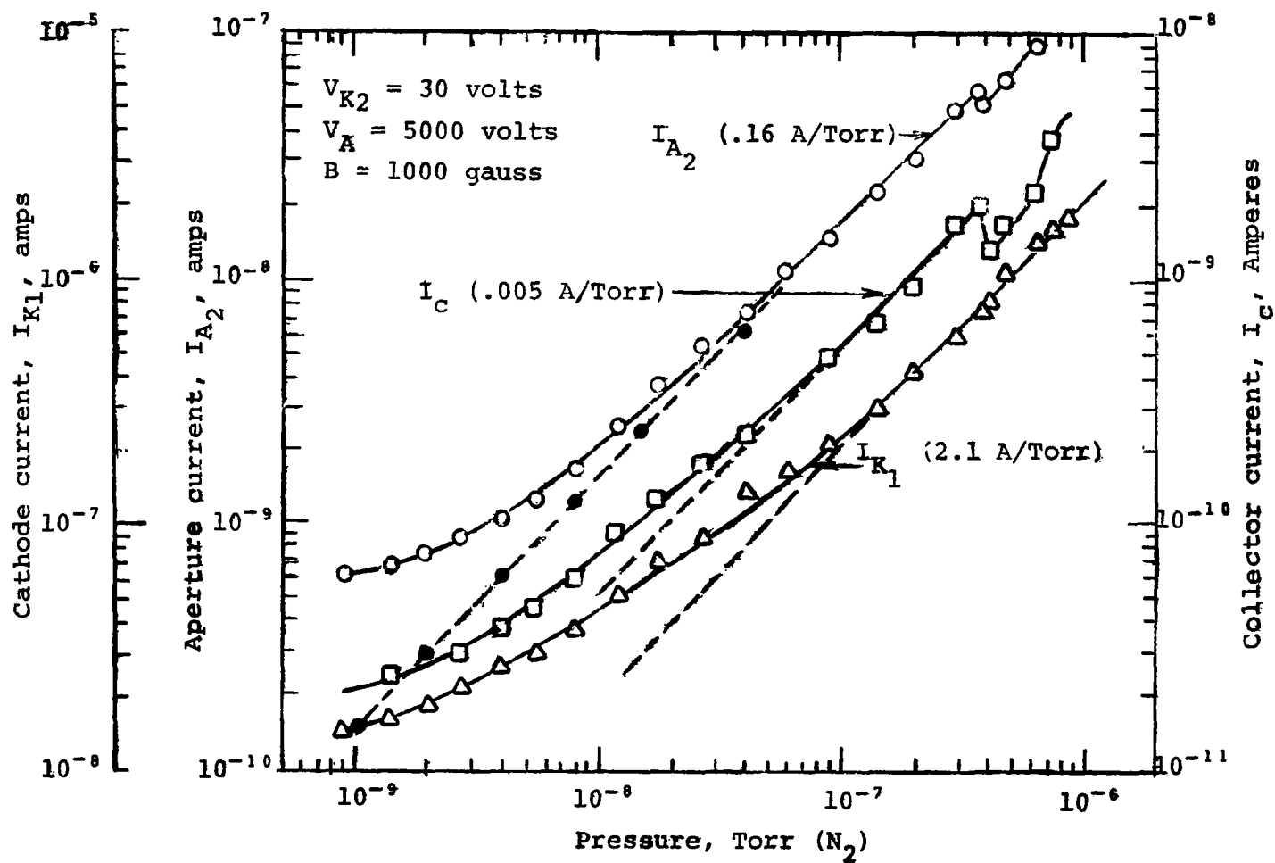
Figure A-11.- Ion currents vs. pressure
