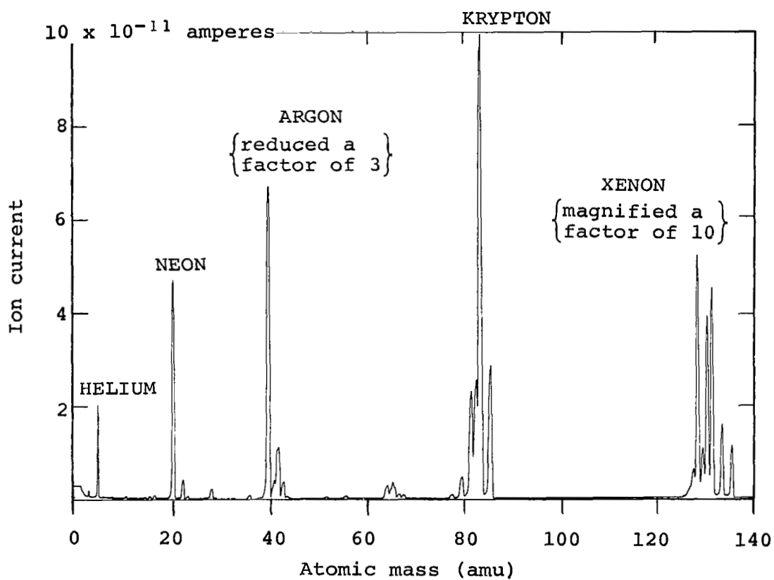
Figure 13.- Performance of CCIS/Quadrupole on medium mass range for inert gas mixture
