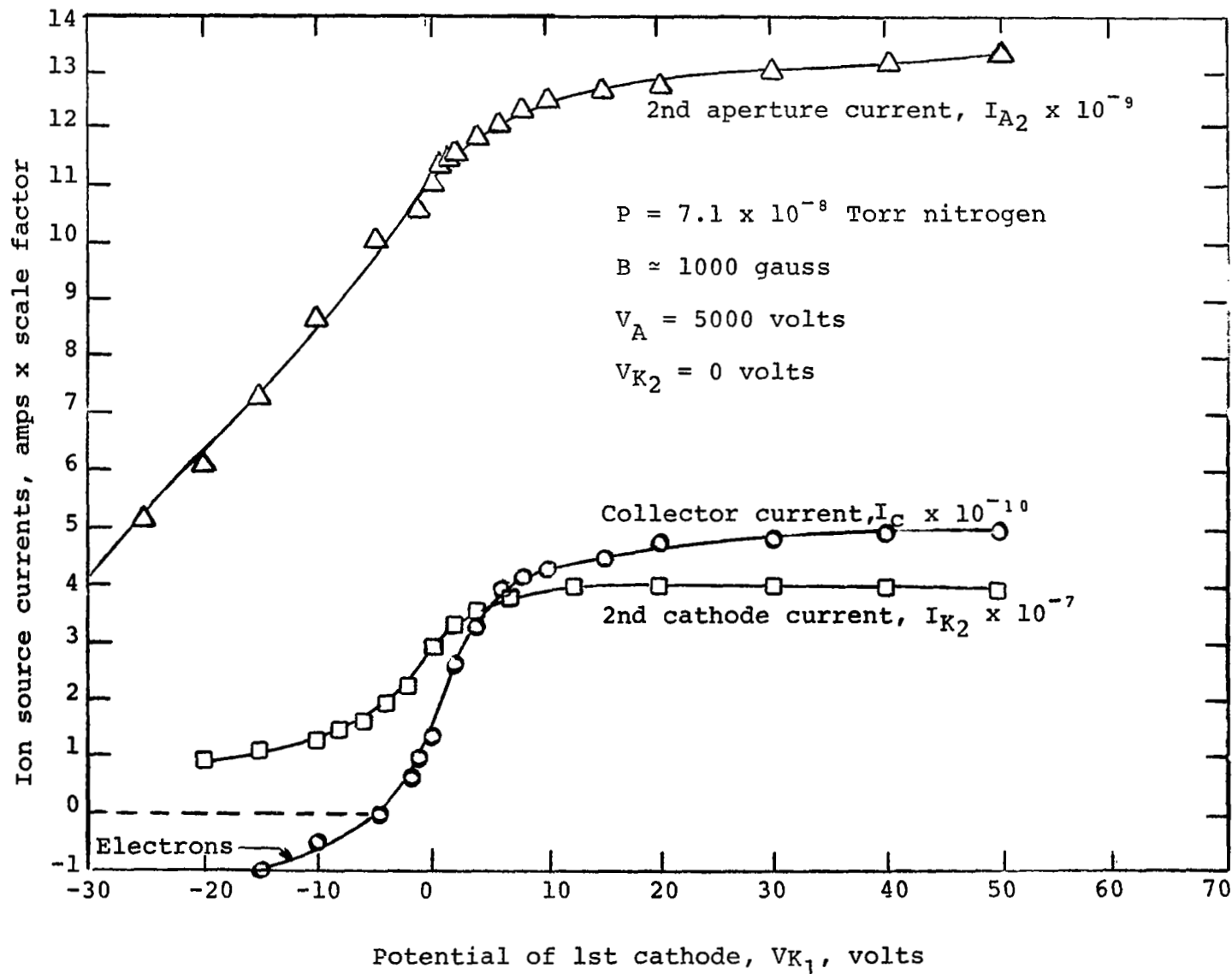
Figure A-8.-Ion extraction data - Method II - V_{K1} positive
