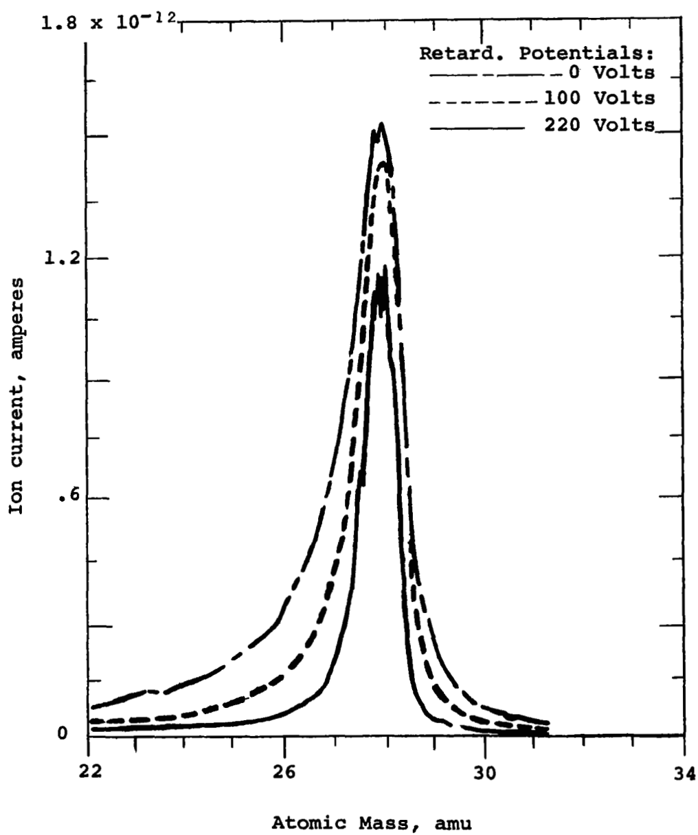
Figure 9.- Effect of retarding potential on resolution and sensitivity of nitrogen peak
