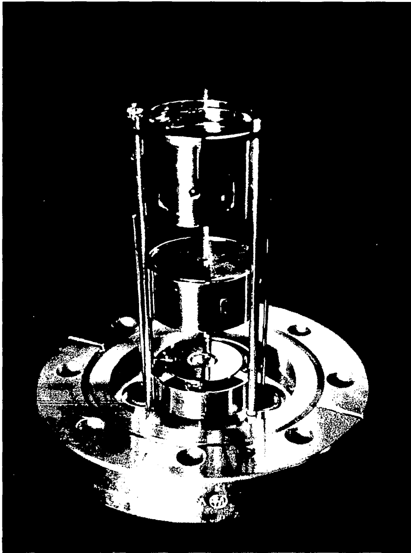
Figure B-3 View of Internal Components of Cold Cathode Ion Source. From Top to Bottom Magnetron, Lens and Probe
