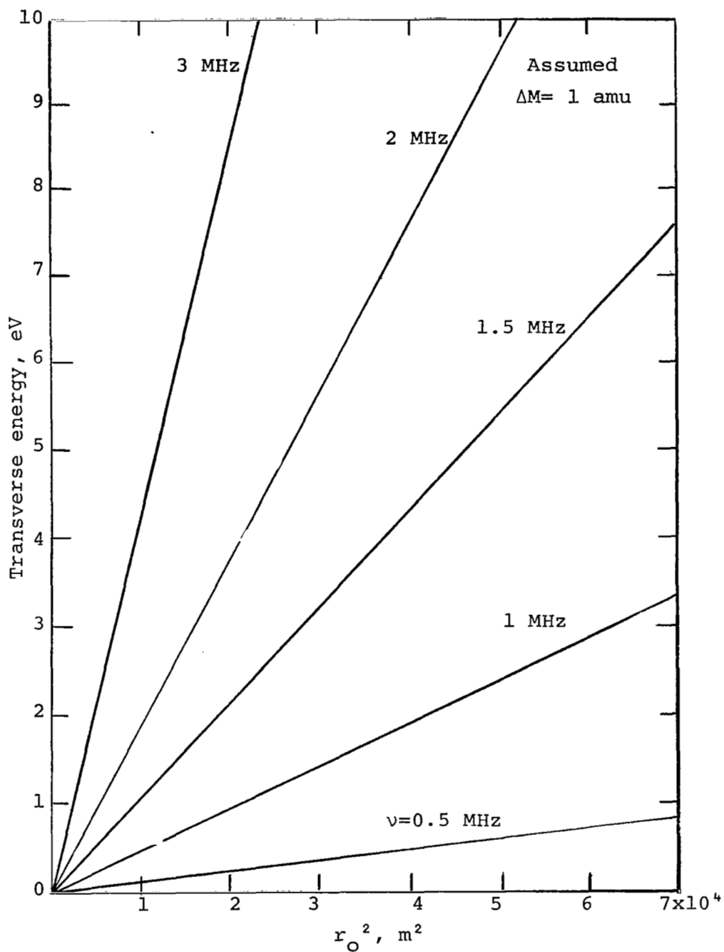
Figure A-15.— Maximum transverse voltage for unity transmission vs. field radius squared
