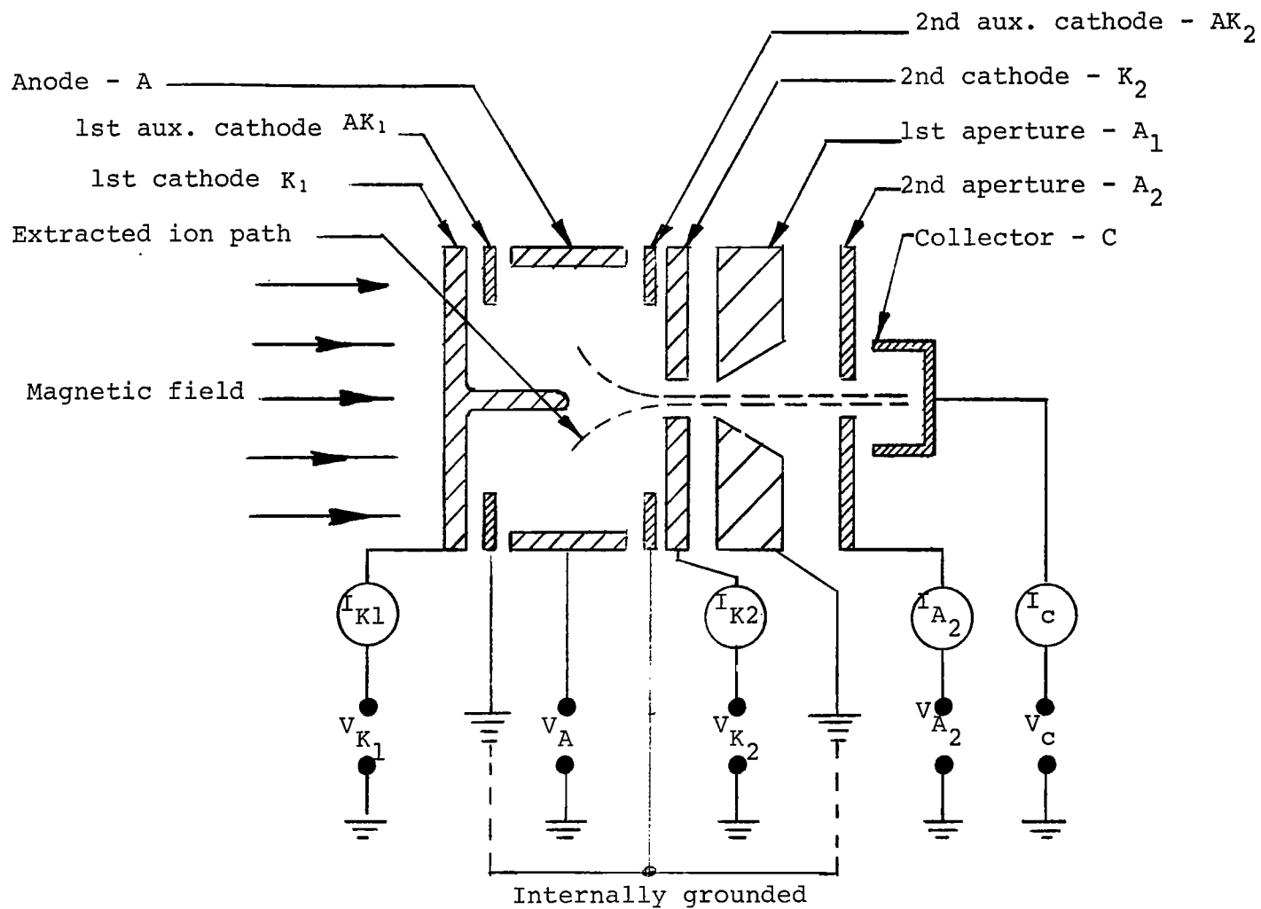
Figure A-4.- Cold cathode ion source schematic
