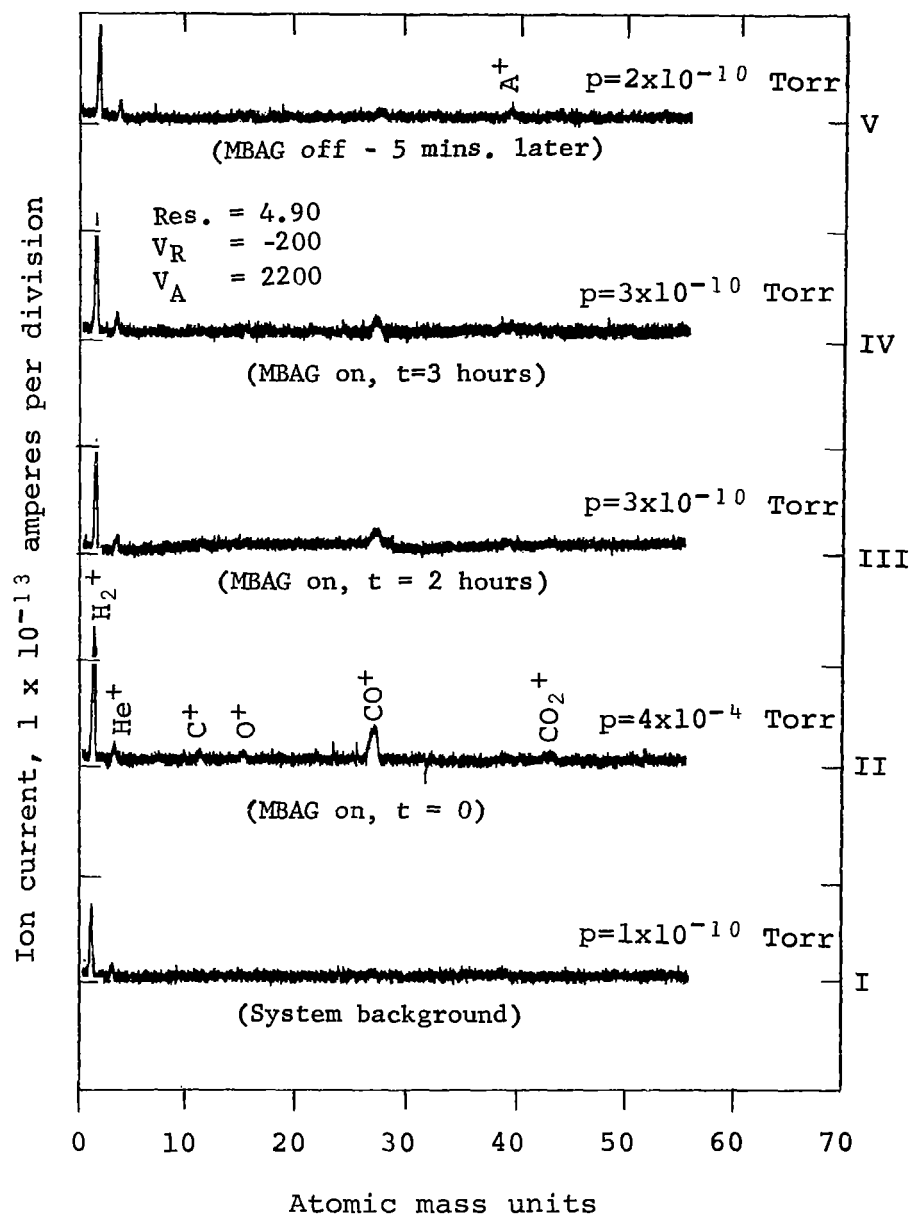
Figure 11.- Background spectra produced by Bayard-Alpert Gauge
