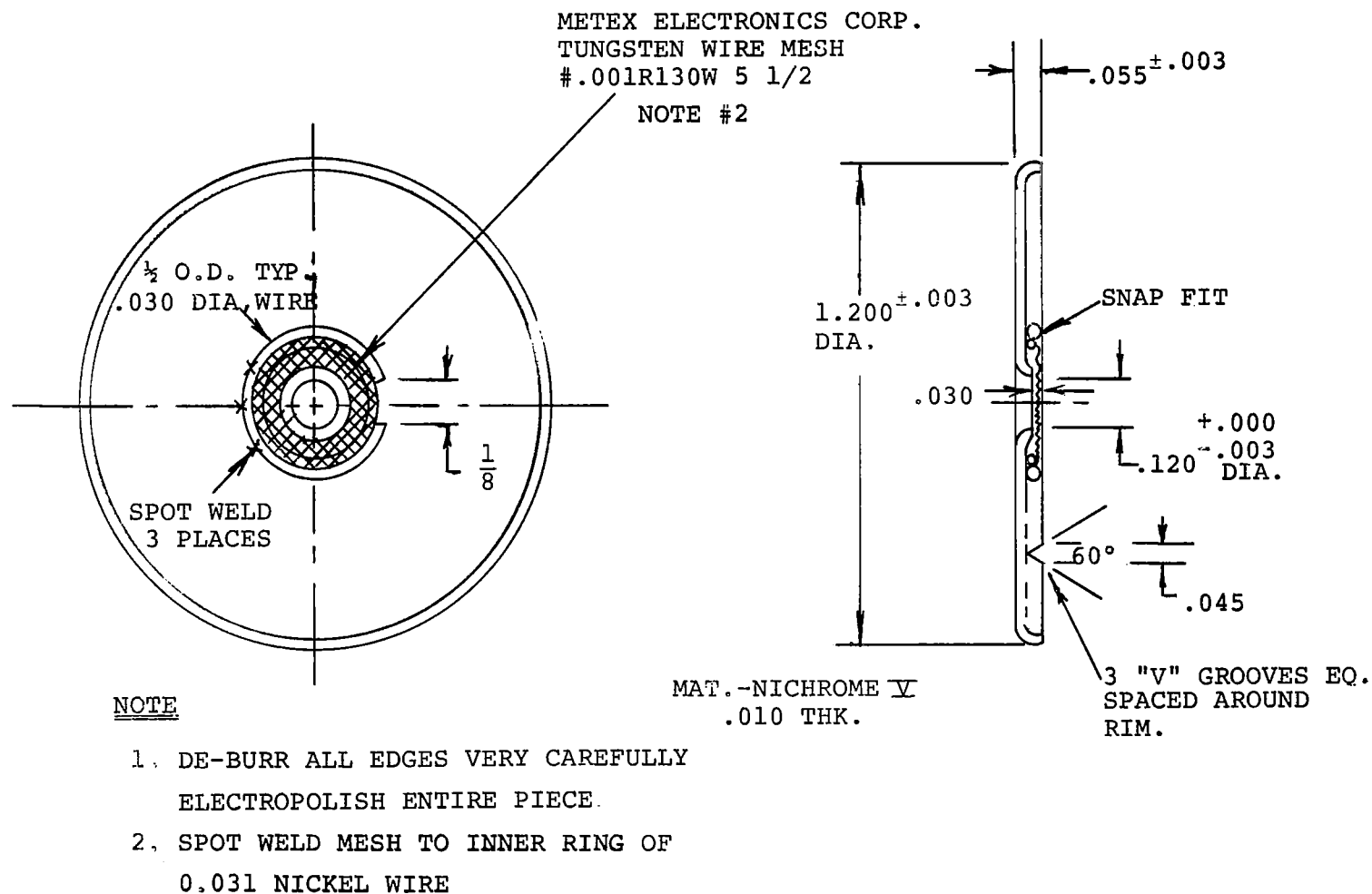
Fig. 50 Cathode End Plate
