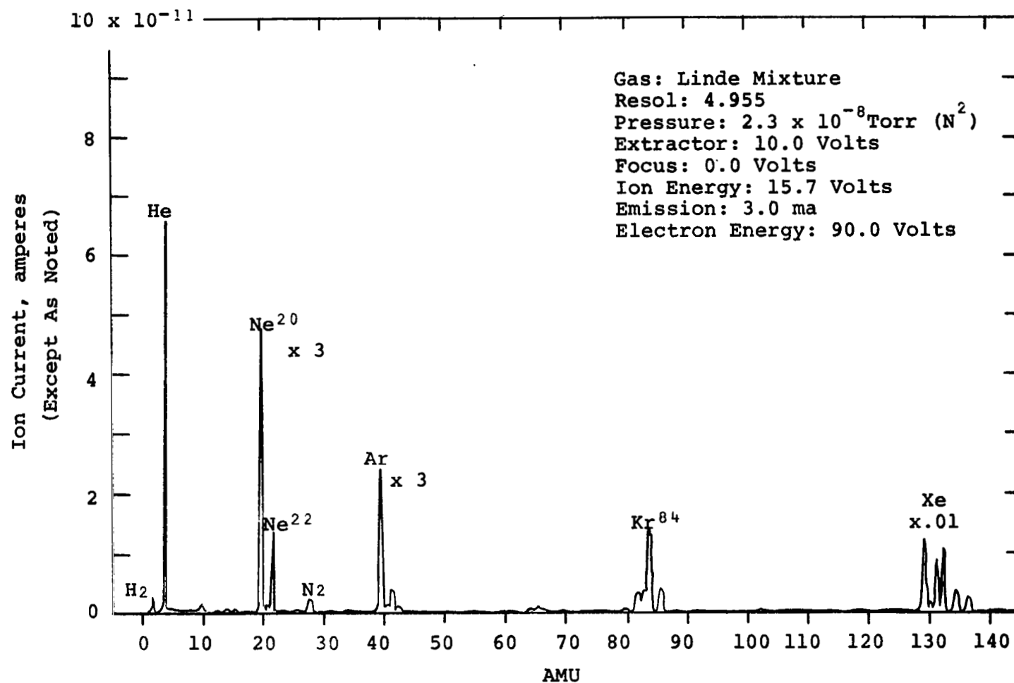
Fig. 2 Medium Mass Range Spectrum Taken with the Hot Filament Spectrometer.
