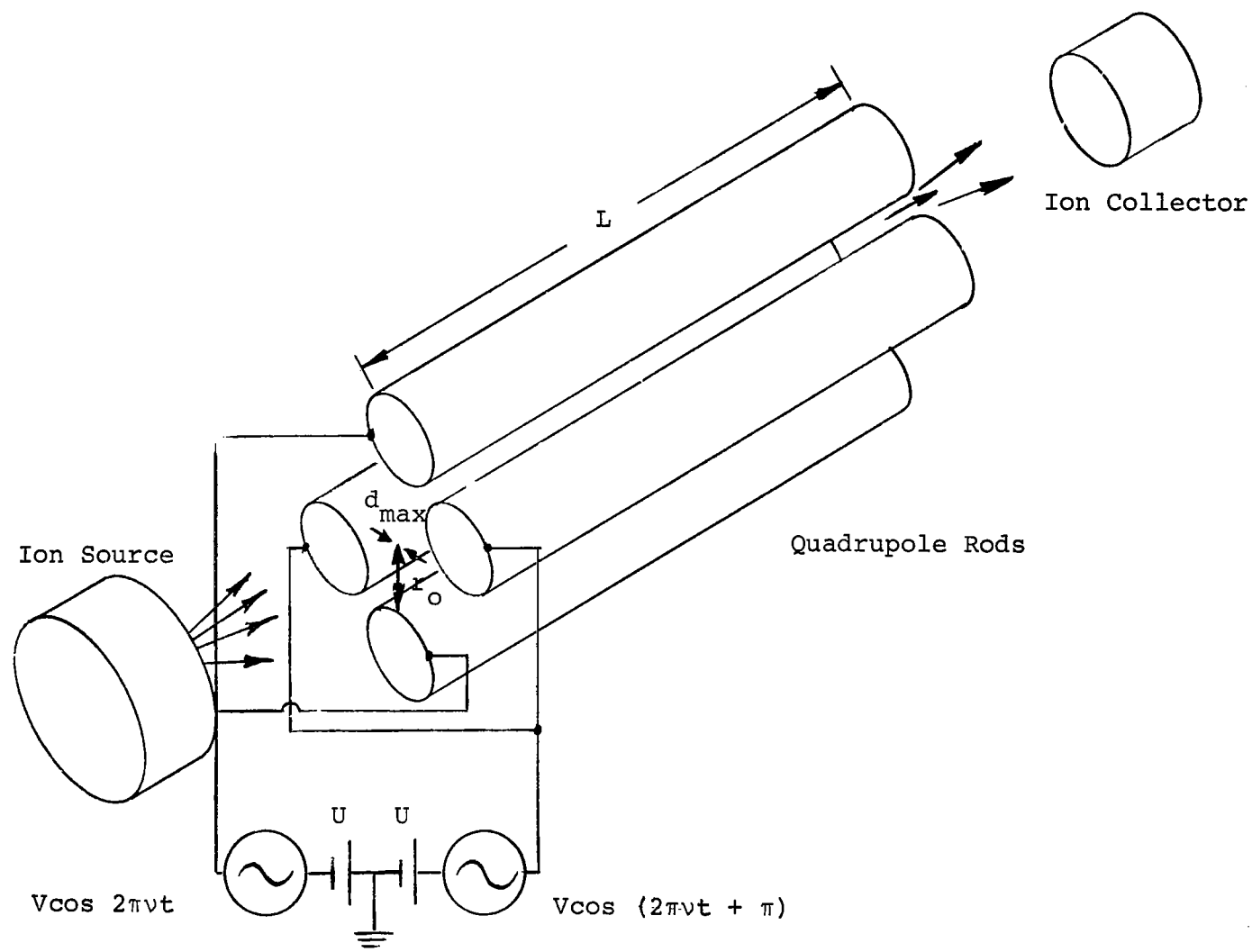
Figure B-20.- Schematic of Quadrupole Mass Analyzer
