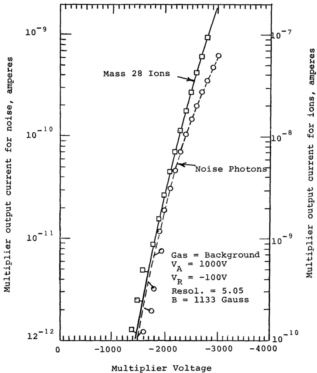
Fig. 31 Ion & Noise Current vs. Multiplier Voltage.
