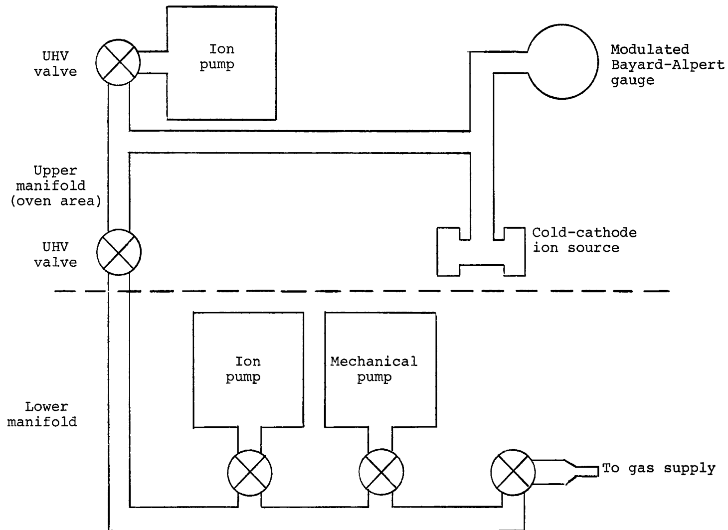
Figure B-5.- Vacuum system schematic
