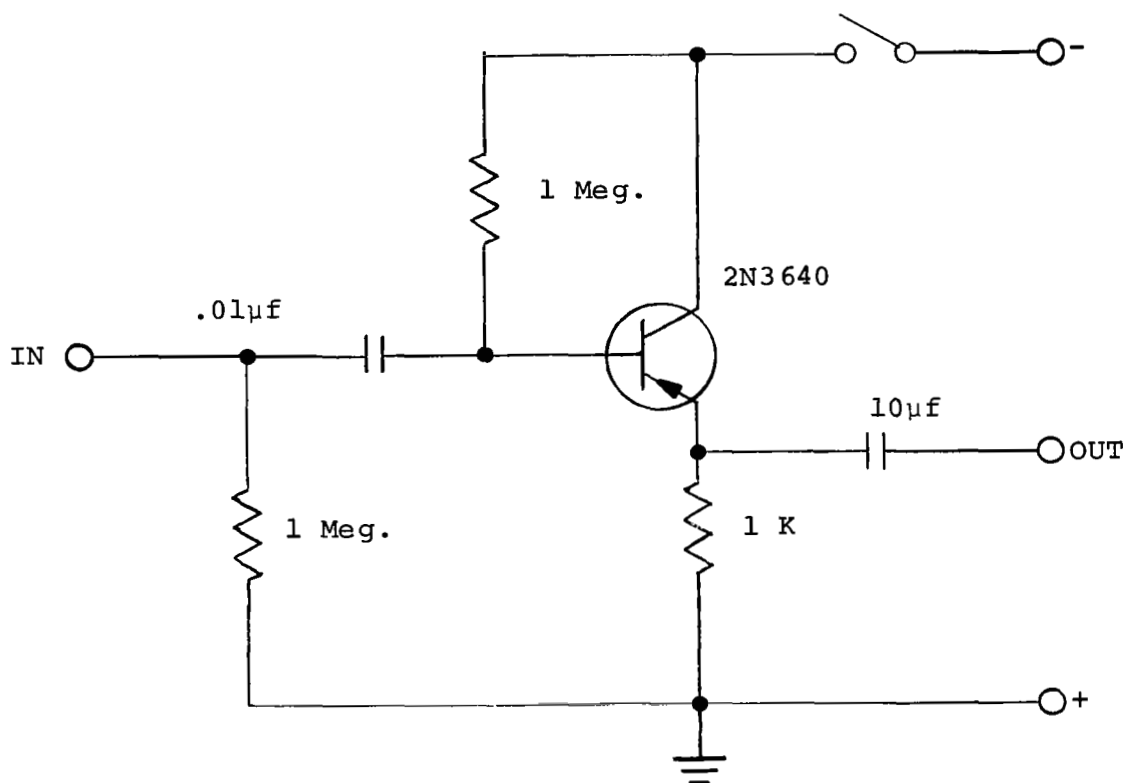
Figure 21. -Preamplifier Circuit Schematic
