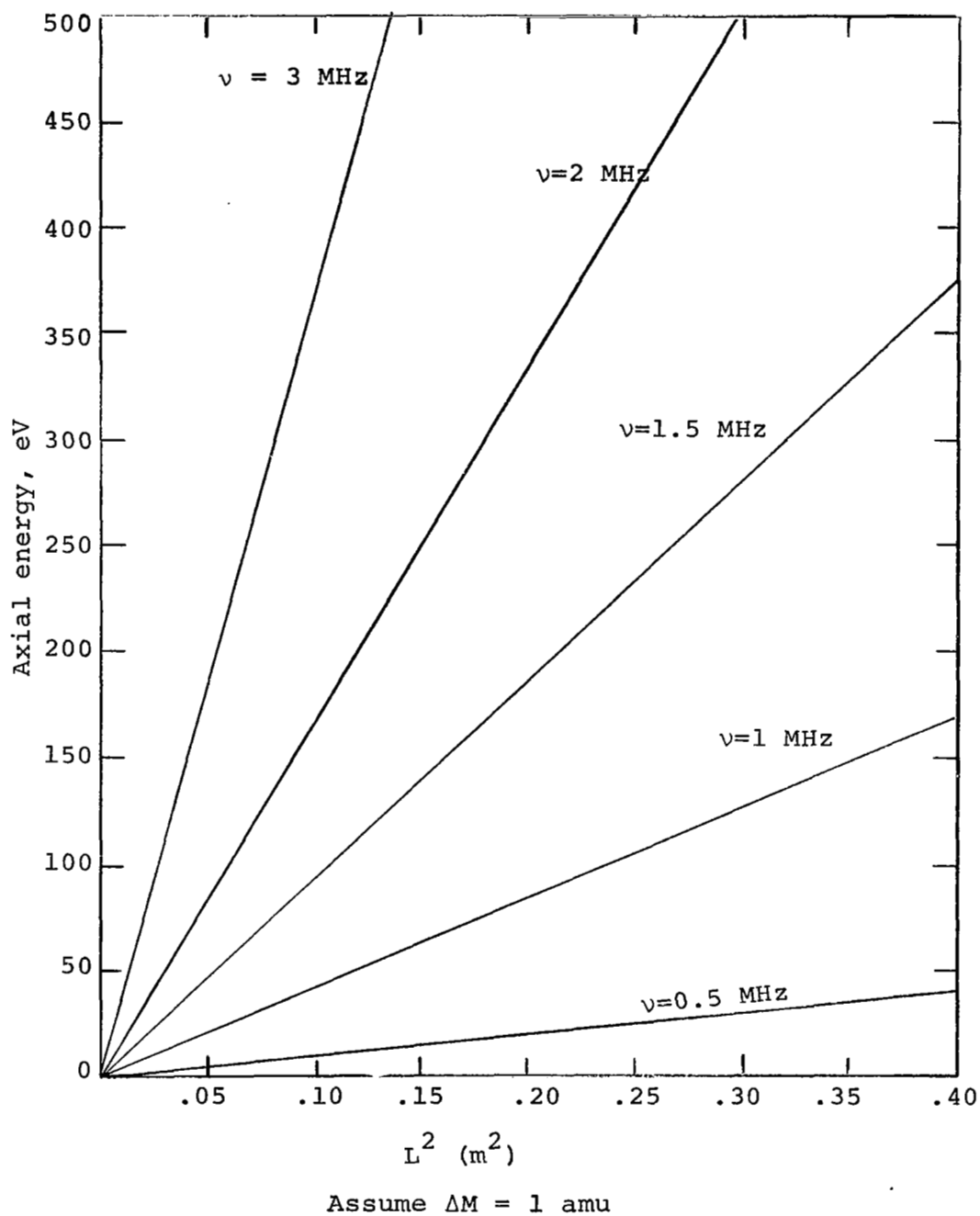
Figure A-16.— Maximum tolerable axial ion energy for selection to occur vs. rod length squared Assumed \Delta M = 1 amu
