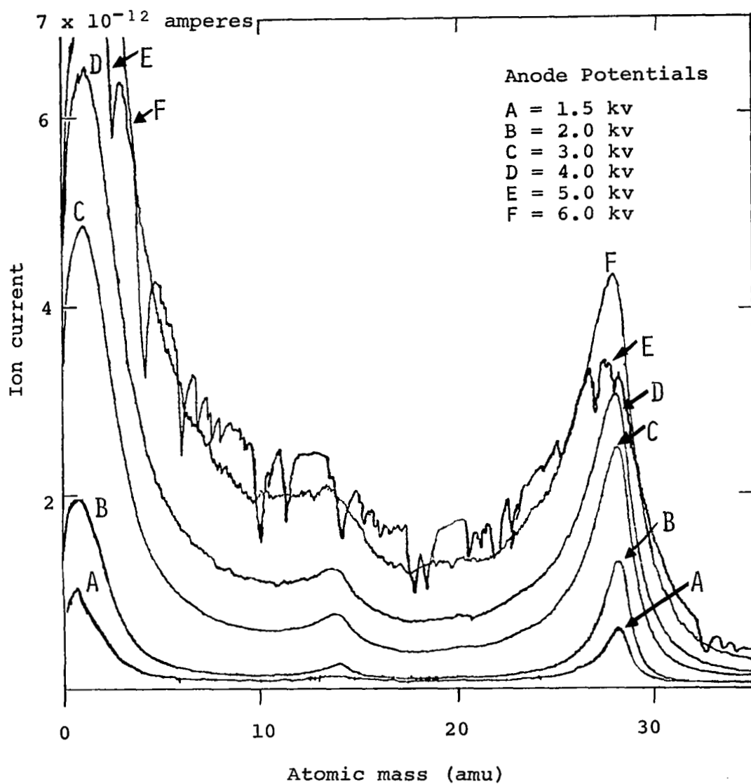
Figure 8.- Resolution and sensitivity vs. anode potential-medium mass range
