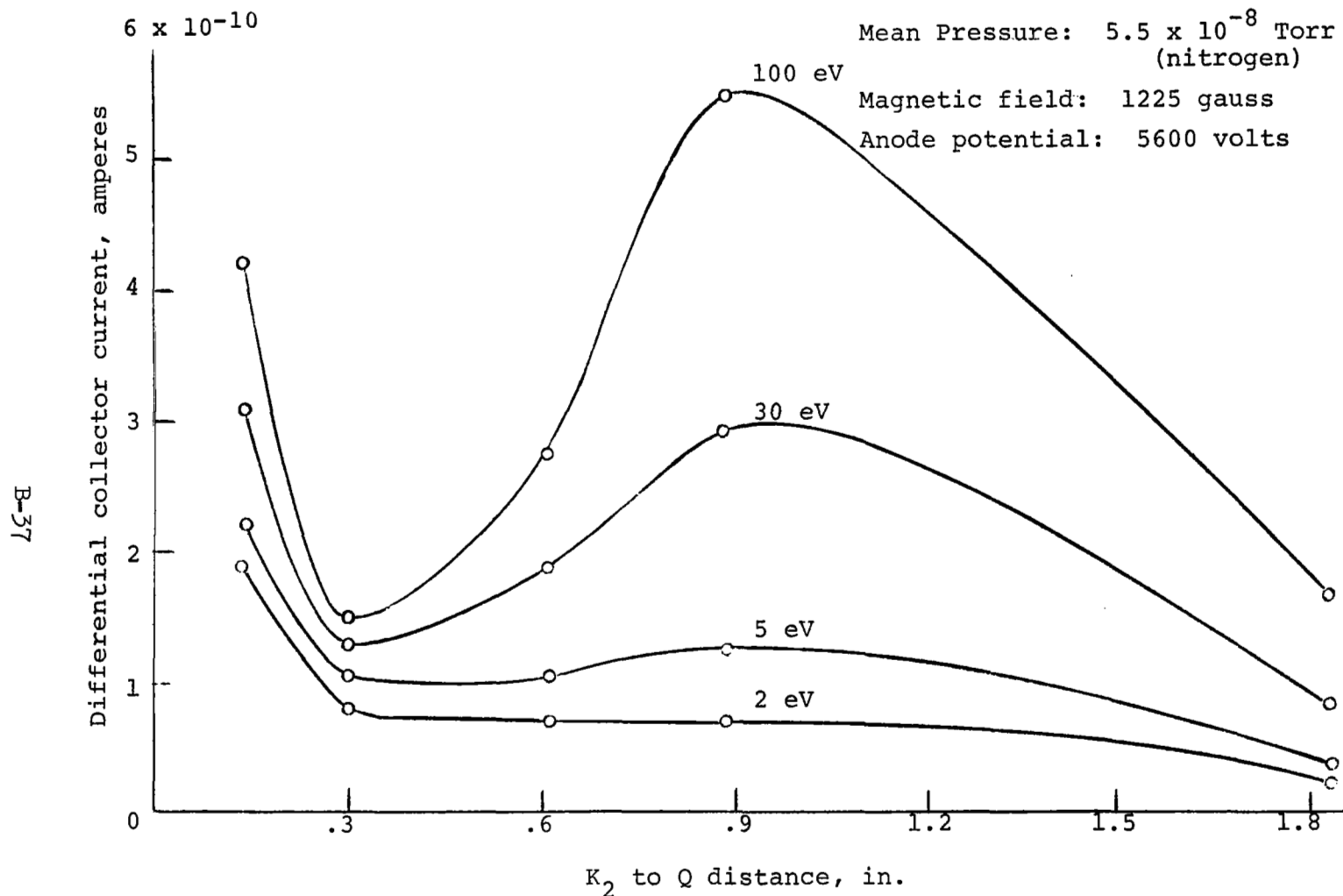
Figure B-11.- Differential collector current vs. distance for selected energy intervals, for V_{K1} = +40 volts
