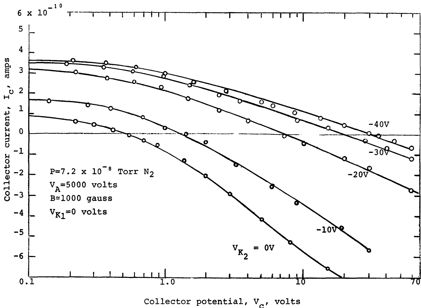
Figure A-9.- Collector current vs. collector potential Unfocused beam - not corrected for contact potentials
