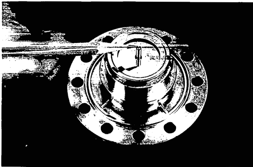
View of Anode End of Source - 1st Cathode ( K_1 )
