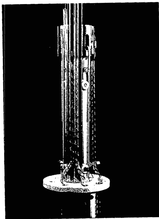
Fig. 40 Lead Assembly CCIS Quadrupole
