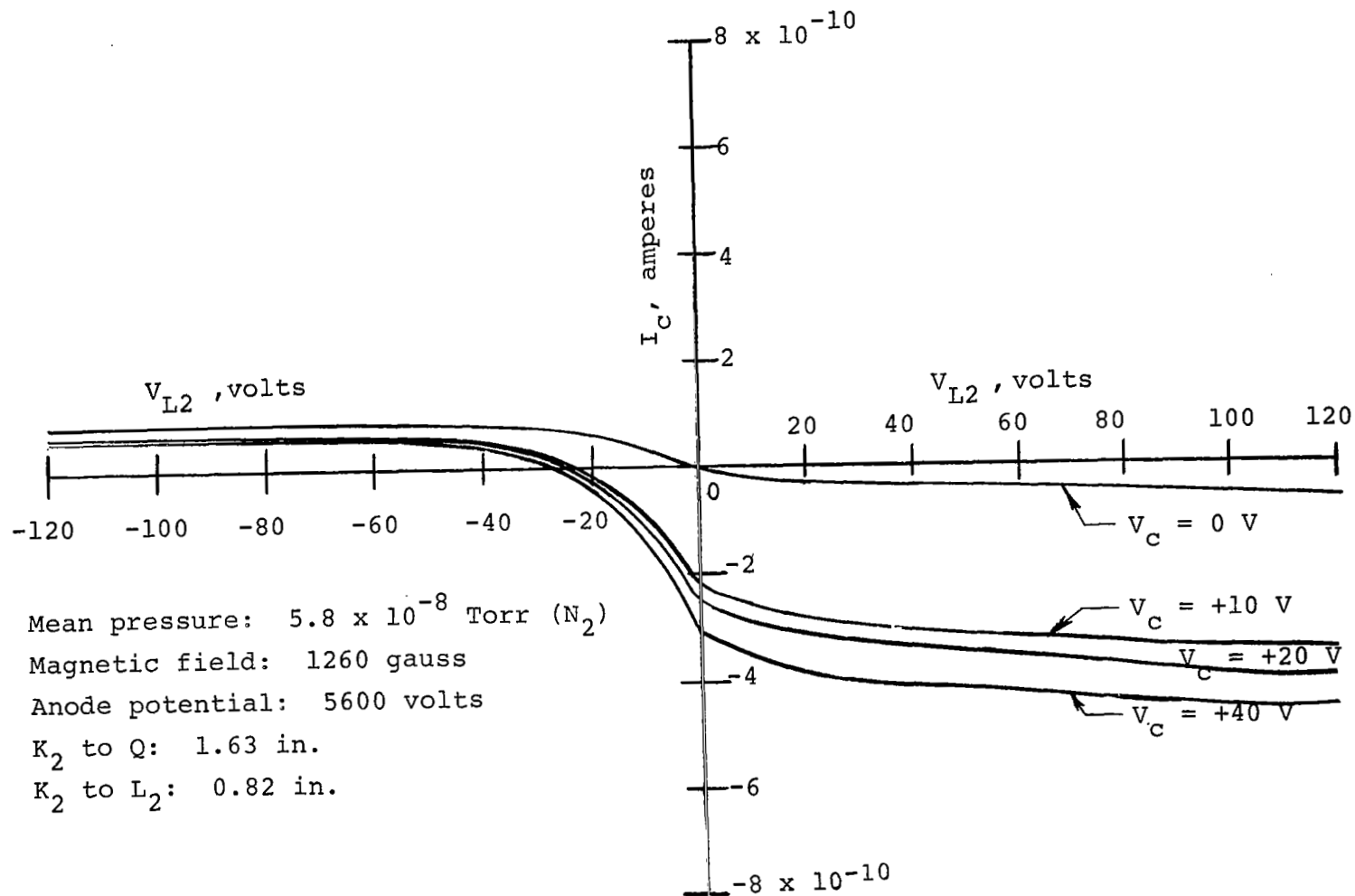
Figure B-16.- Effect of lens potential variations: I_C vs. V_{L2} for selected V_C values at position 2, V_{K1} = zero volts
