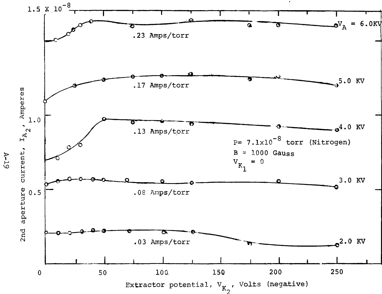
Figure A-5.- 2nd aperture current vs. negative extractor potential.
