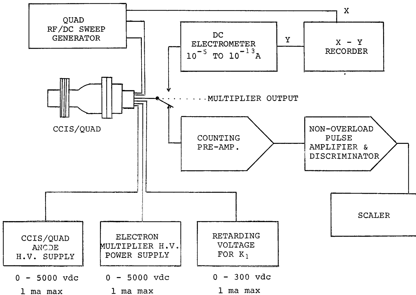
Fig. 17 - Block Diagram of Equipment
