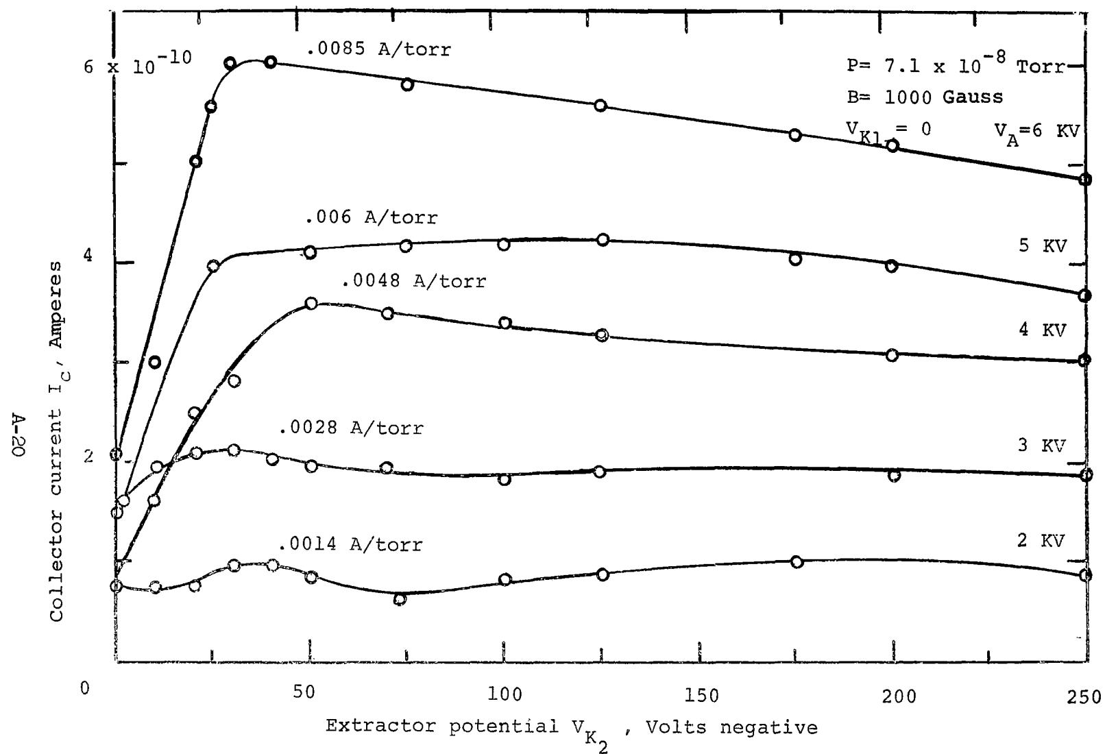
Figure A-6.- Collector current vs. negative extractor potential
