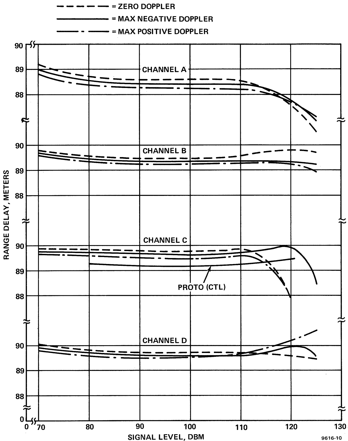
Figure 4.2.5-2 Range Delay vs. Signal Level
