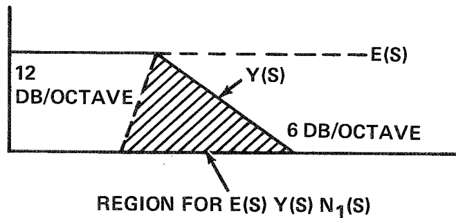
Figure 4.1.5-2 Noise Spectrum
