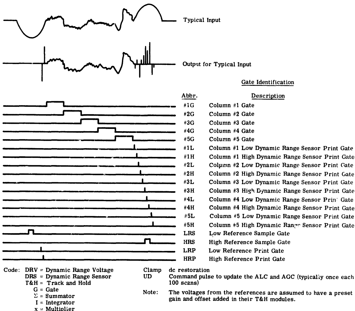
FIGURE 14. TERMS AND WAVEFORMS IN FIGURE 13
