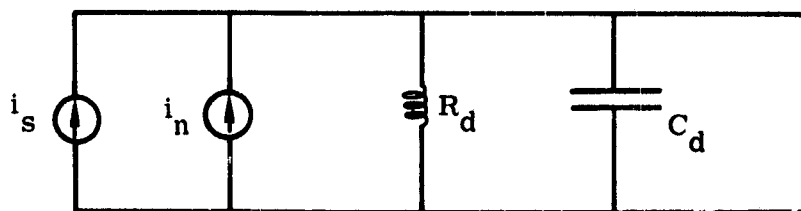
FIGURE 19. Ge:Hg DETECTOR EQUIVALENT CIRCUIT
