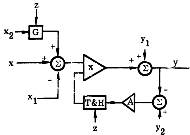
FIGURE 18. ALC-AGC CIRCUIT
