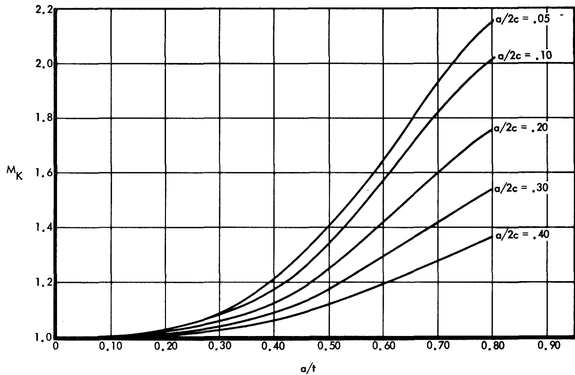
Figure 57: DEEP FLAW MAGNIFICATION CURVES (t = 0.200", 5Al-2.5Sn Titanium Base Metal (Transverse) & Weldment @ -320°F & -423°F)
