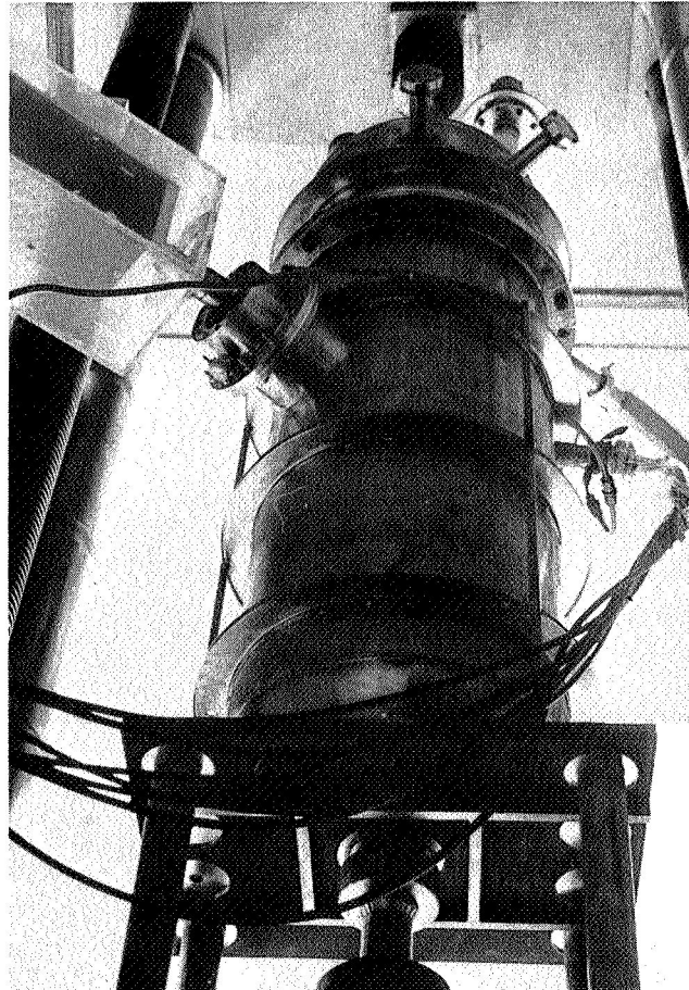
Figure 32: LH 2 CRYOSTAT
