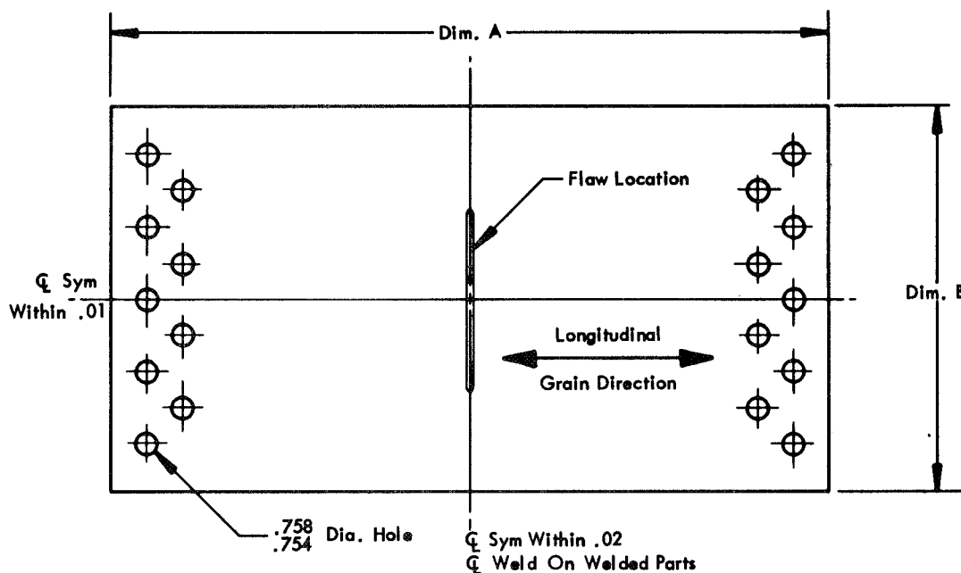
Figure 27: CENTER CRACK FLAW SPECIMEN FOR 5AL-2.5Sn (ELI) TITANIUM
