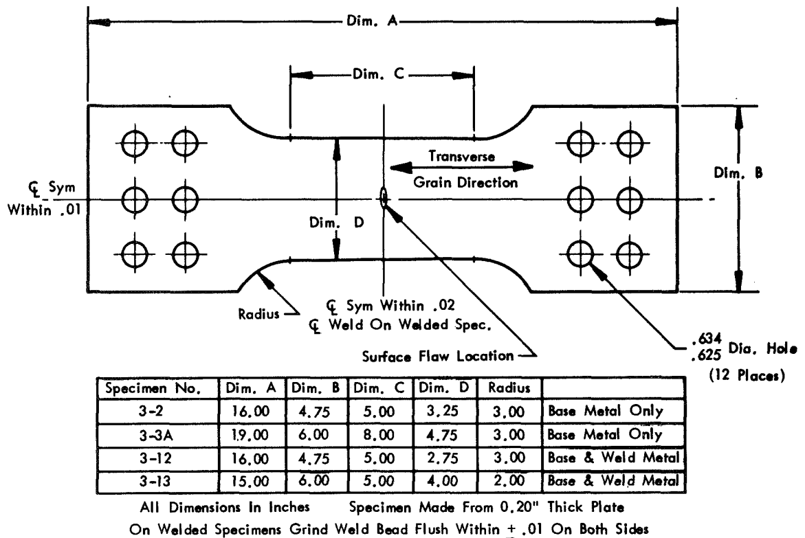
Figure 16: SURFACE FLAW SPECIMEN FOR 5AL-2.5Sn (ELI) TITANIUM
