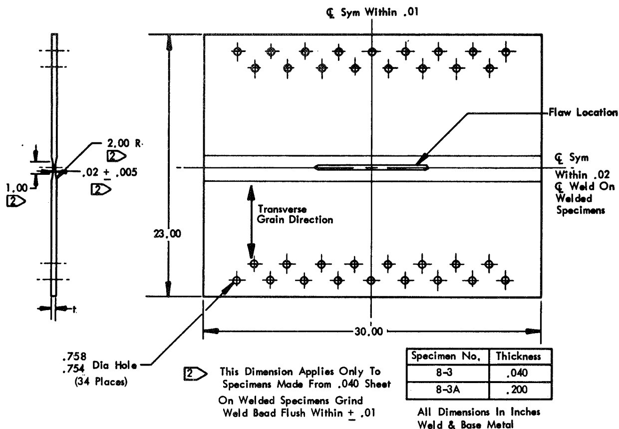
Figure 27: CENTER CRACK FLAW SPECIMEN FOR 5AL-2.5Sn (ELI) TITANIUM
