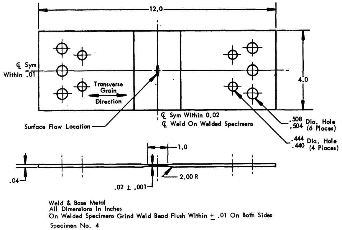
Figure 15: SURFACE FLAW SPECIMEN FOR 5AL-2.5Sn (ELI) TITANIUM
