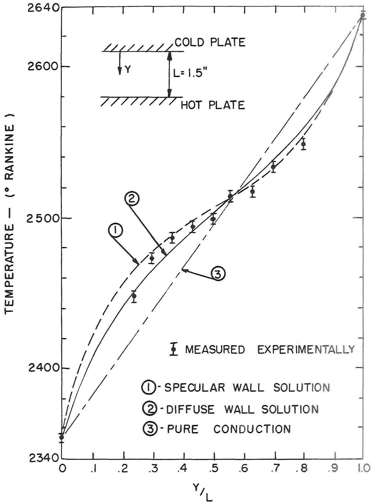
FIGURE 21 TEMPERATURE PROFILES IN GLASS
