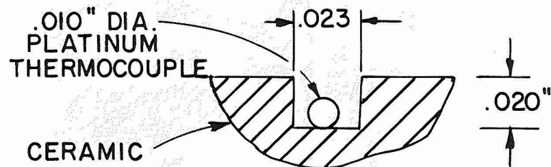
FIGURE 14 THERMOCOUPLE POSITIONS ON CERAMIC TRAY
