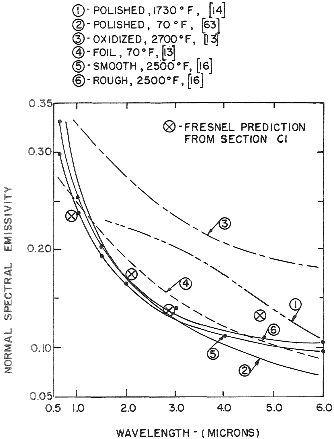
FIGURE C5 NORMAL SPECTRAL EMISSIVITY OF PLATINUM IN AIR
