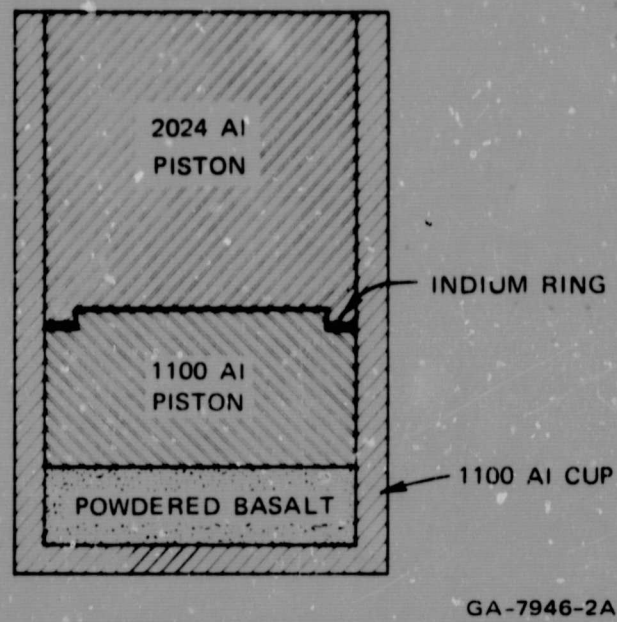
FIGURE 3 SOFT ALUMINUM CONTAINER
