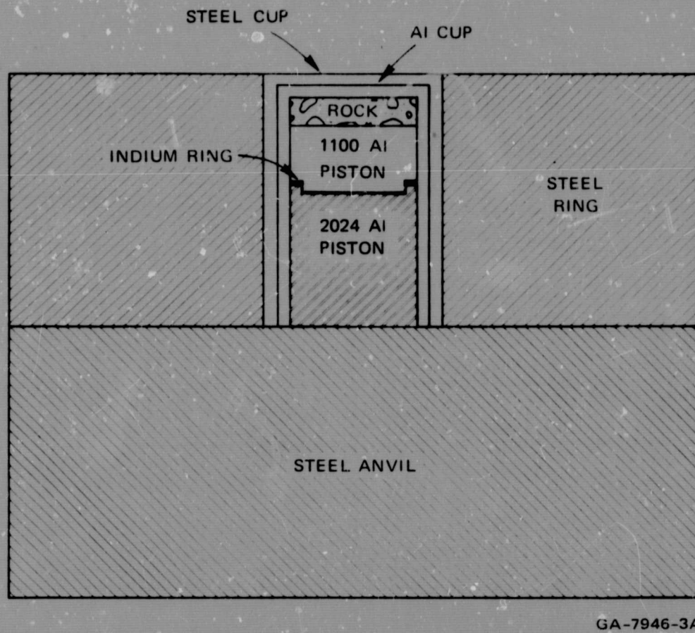
FIGURE 4 PLANE WAVE GEOMETRY CONTAINER AND MOMENTUM TRAP
