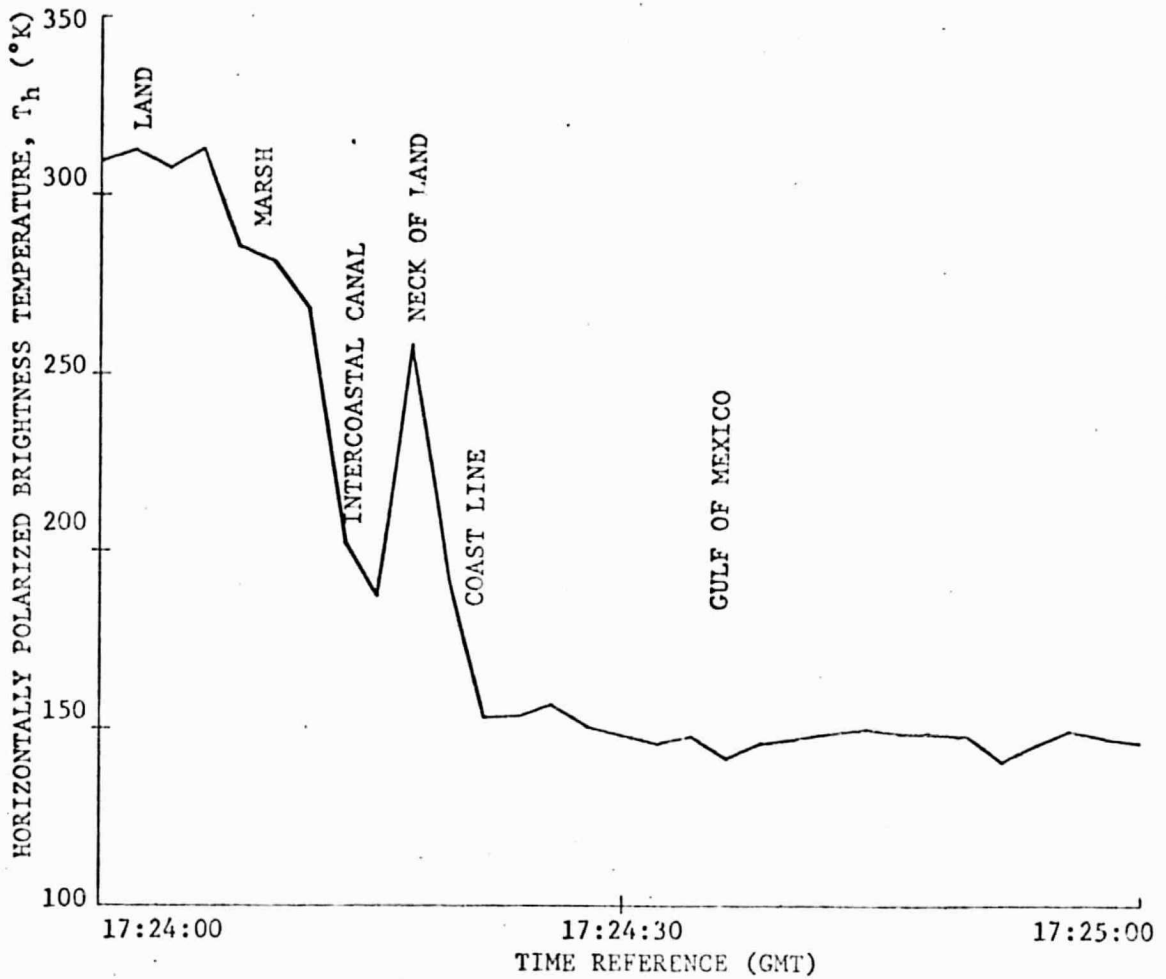
Measured values of the horizontally polarized brightness temperature from 17:24 Z to 17:25 Z during Flight 12 versus time for an incidence angle of 0^{\circ} and for a frequency of 19.35 GHz as the aircraft flew from land to water.
