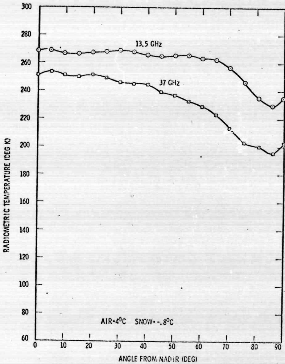
Horizontal Brightness Temperature of Snow.
