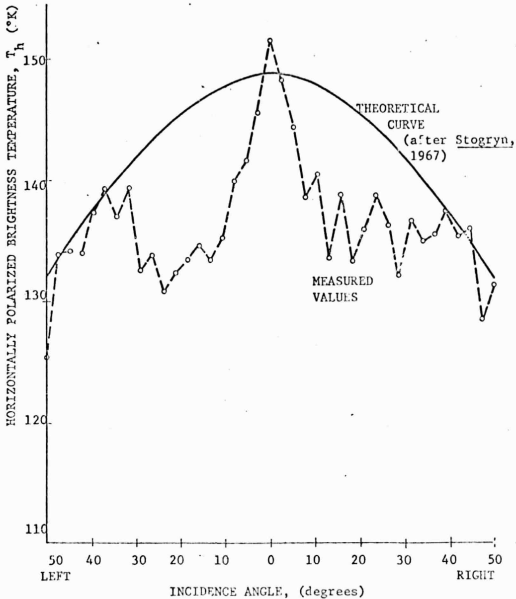
The average value of the horizontally polarized brightness temperature (circles and dashed line) measured during Flight 12 from 18:13:00Z to 18:13:30Z versus incidence angle and corresponding theoretical values (solid line) from Stogryn (1967) for a frequency of 19.35 GHz.
