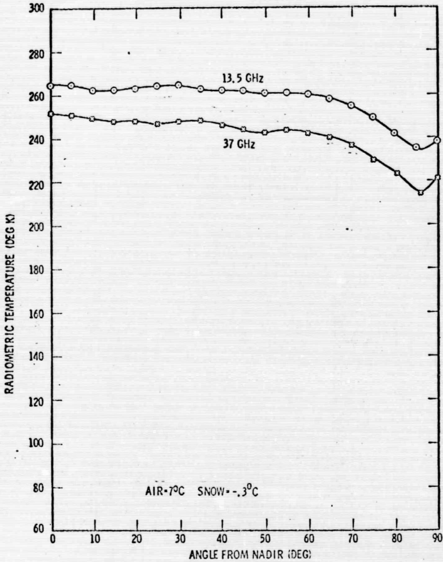
Vertical Brightness Temperature of Snow.
