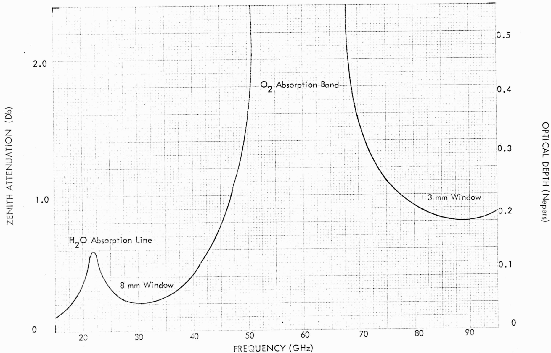
FIGURE B1 - APPROXIMATE ZENITH OPACITY OF THE TERRESTRIAL ATMOSPHERE
