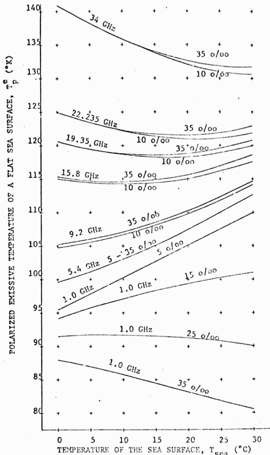
The polarized emissive temperature of a flat sea surface versus the thermometric temperature of the sea surface for frequencies of 1, 5.4, 9.2, 15.8, 19.35, 22.235, and 34 GHz and for various salinities.
