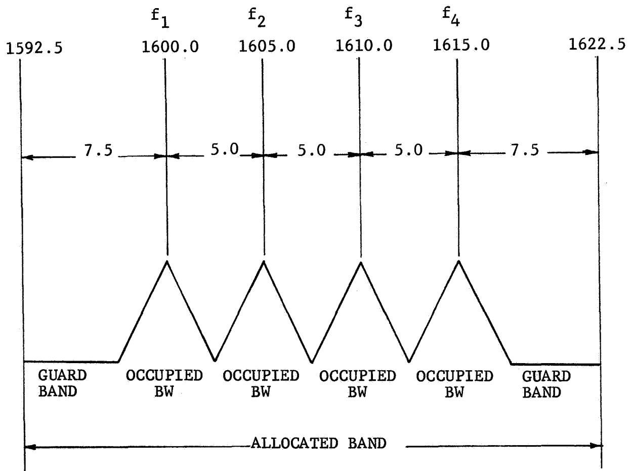
FIGURE 5 POSSIBLE CAS FREQUENCIES
