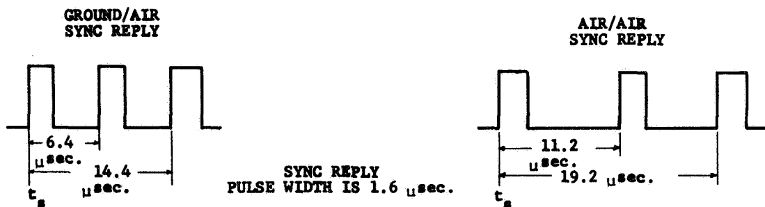
FIGURE 6 COLLISION AVOIDANCE SYSTEM MESSAGE FORMAT, BASIC SIGNAL
