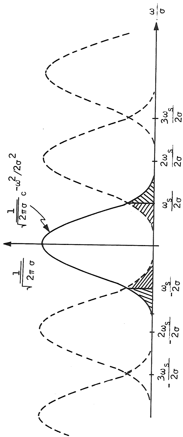
FigureG1. Spectrum of Sampled Gaussian Pulse ( e^{-t^2d^2/2} )
