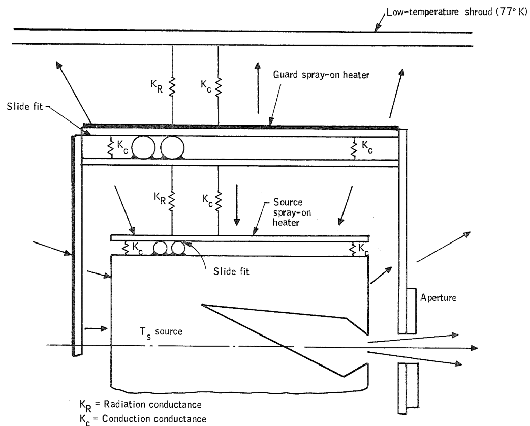
Figure H3. Schematic of LRC Source and Temperature Control System
