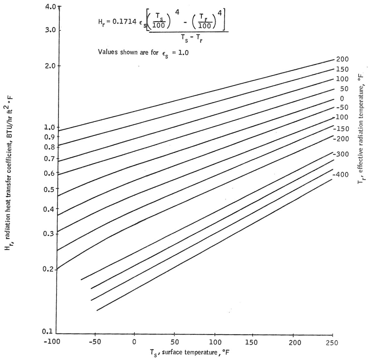
Figure I2. Radiation Heat Transfer Coefficient versus Surface Temp.
