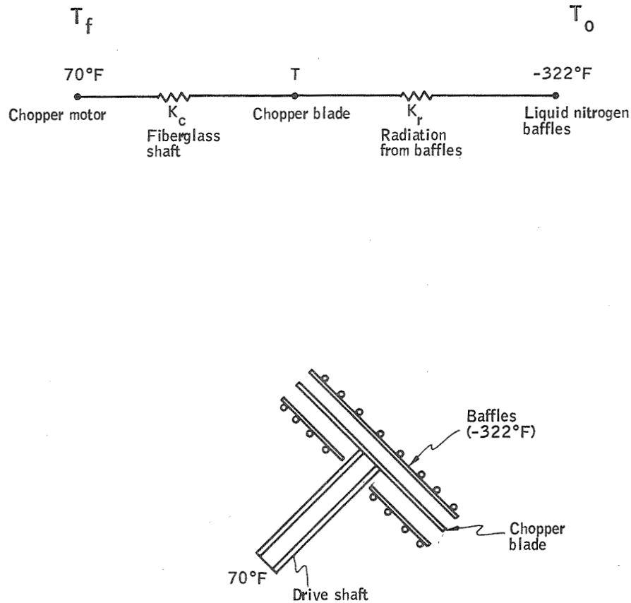
Figure I1. Three-Node Thermal Network
