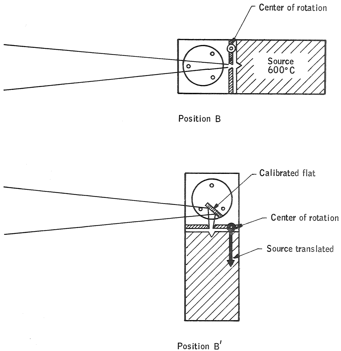
Figure 103. Calibrated Flat Reflectance Measurement
