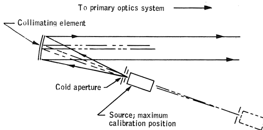
Figure 110. Movable-Source Mechanization
