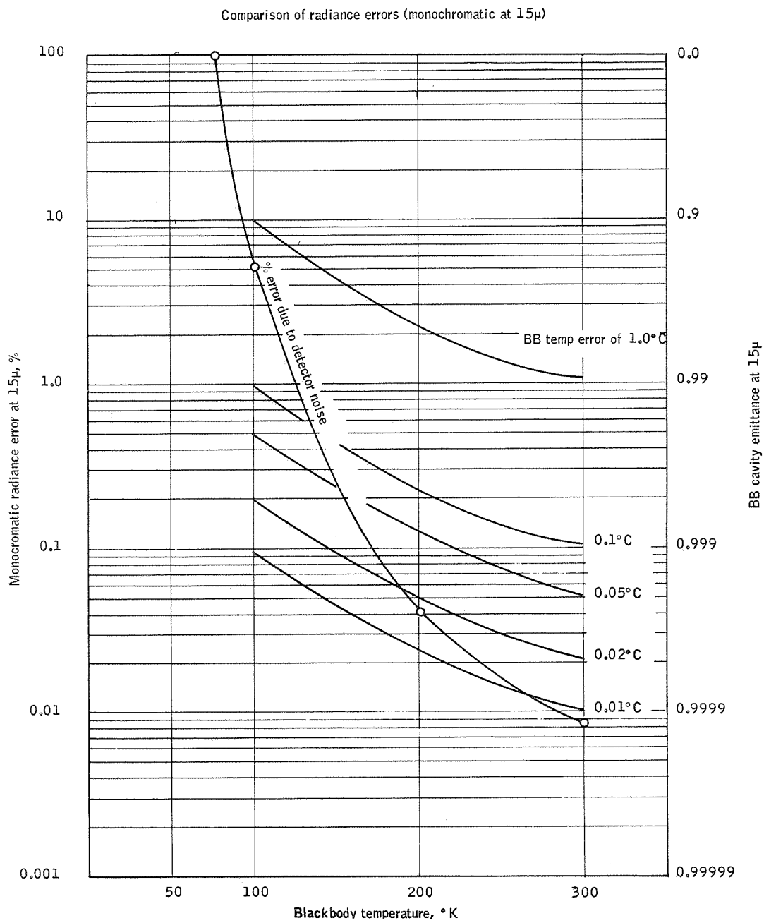
Figure 79. Radiance Error Due to Temperature Error
