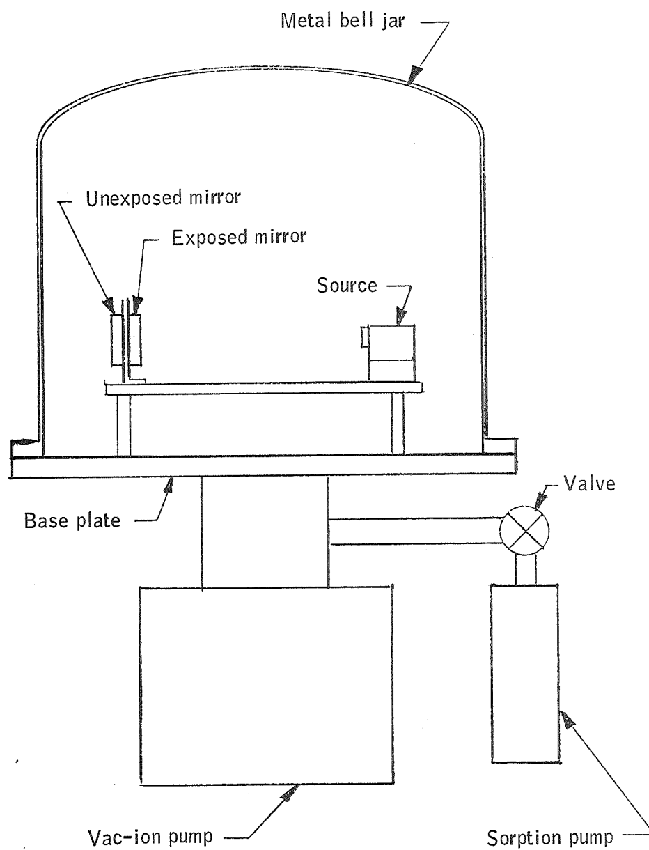
Figure 125. Source Stability and Mirror Aging Test
