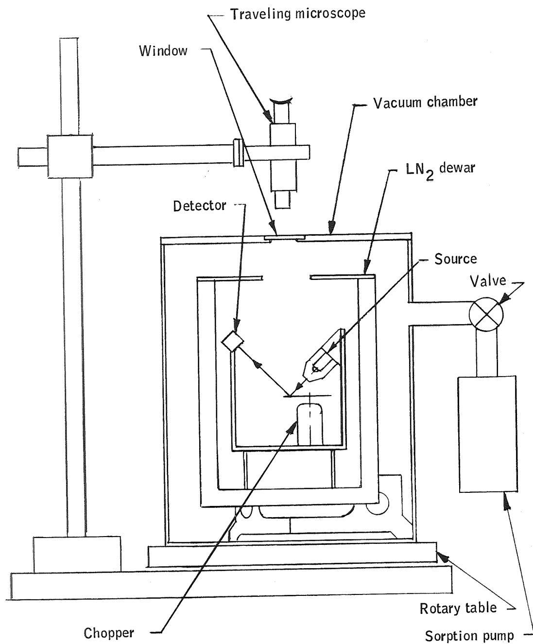
Figure 128. Chopper Test Setup
