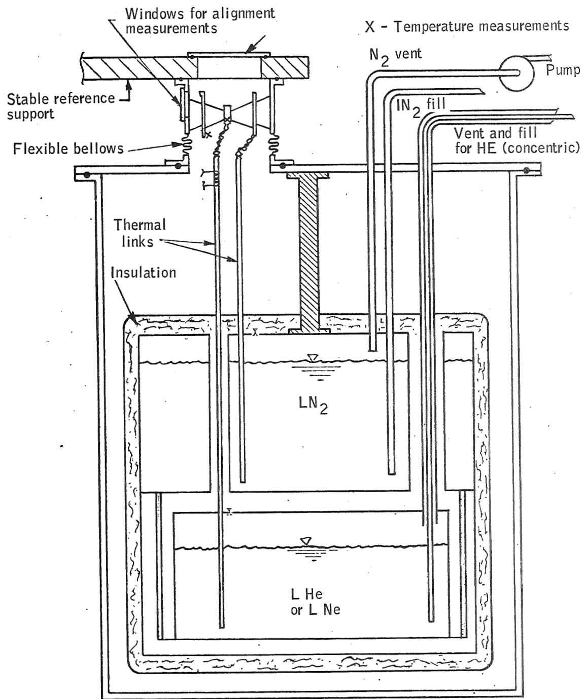
Figure 144. Detector and Lens Cooling Concept for Testing
