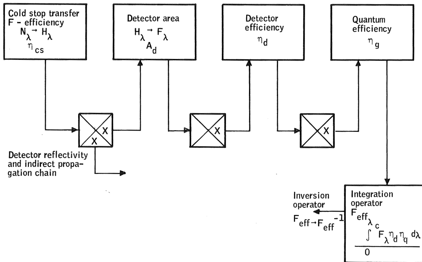
Figure 19. Modification of Final Model Stage Needed to Consider Propagation of Spectral Radiances
