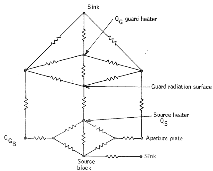
Figure H4. Twelve-Node Thermal Network Simulation of the LRC Calibration System
