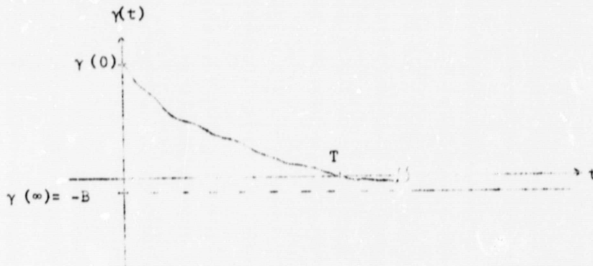
\gamma(t) Reaches Zero in Finite Time
