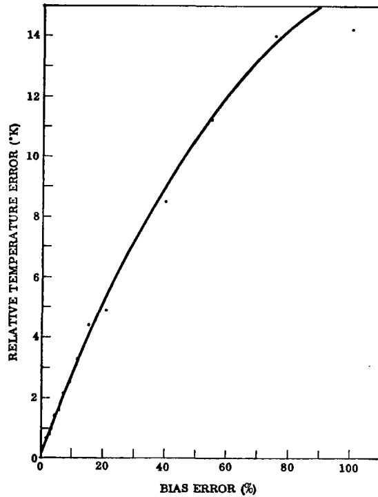
Fig. 10 Relative Temperature Error Resulting From a Bias Radiance
