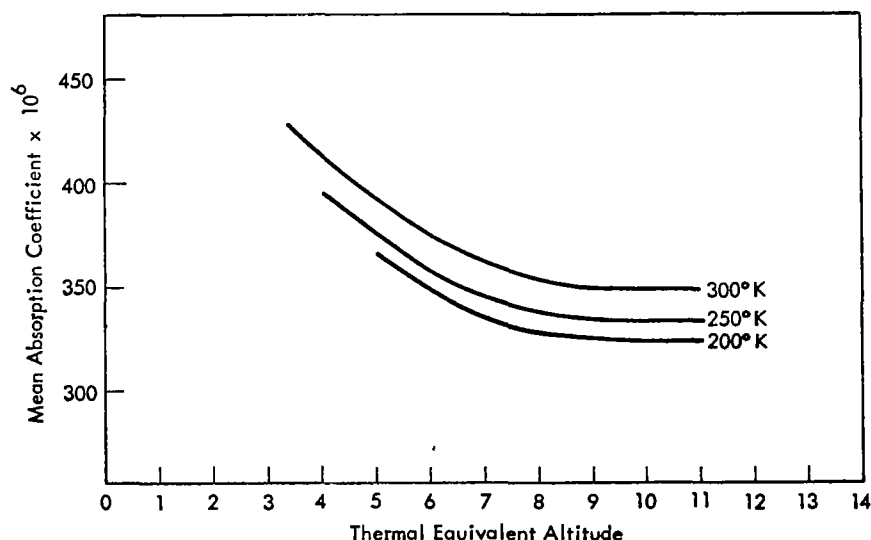
Fig. 7 Calculated Mean Absorption Coefficients for 200°, 250°, and 300°K Isothermal Atmospheres
