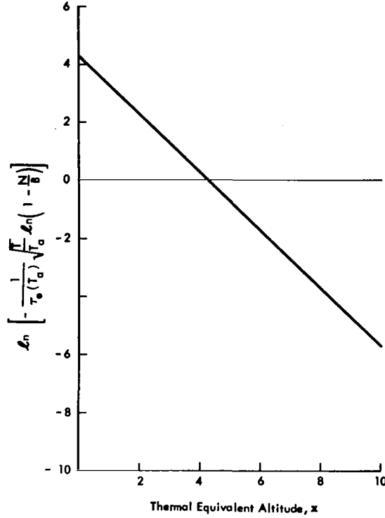
Fig. 6 Linearized Limb Radiance for Isothermal Atmospheres
