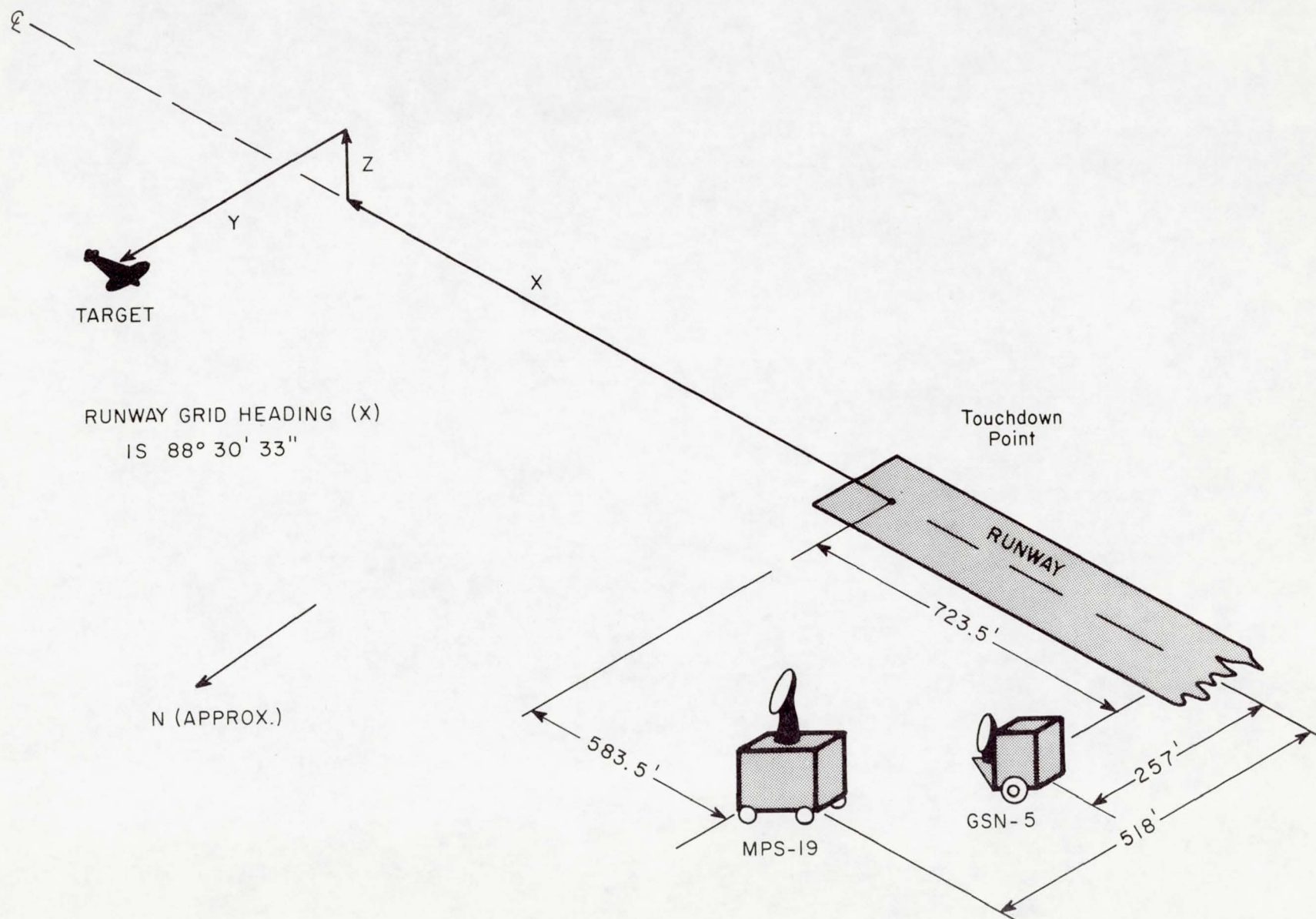
Fig. 4-2. Coordinate system and radar offsets.
