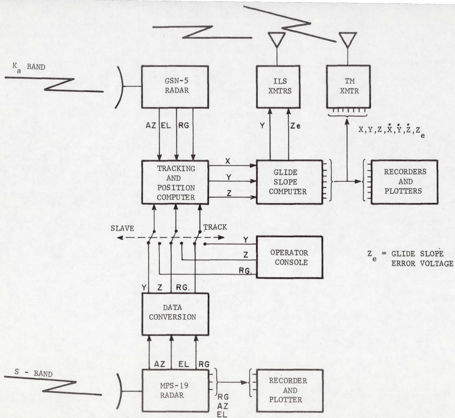
Fig. 4-1. System block diagram.
