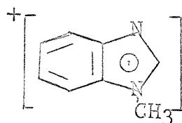
the cation and anion radicals
