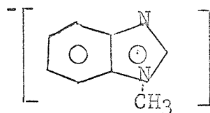
the cation and anion radicals
