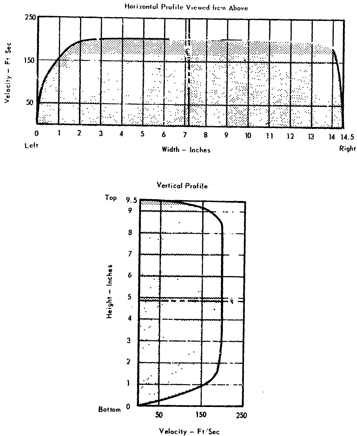
Figure 3 - A Typical Wind Velocity Profile at 9.5 Inch X 14.5 Inch Tunnel Exit
