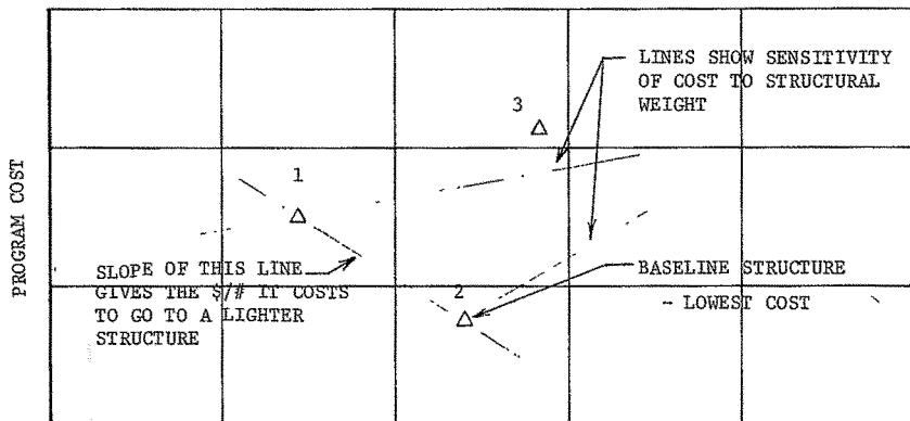
WEIGHT OF ORBIT MANEUVER SYSTEM AS STRUCTURAL ALTERNATES ARE VARIED
