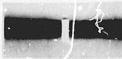
Figure 32. Radiograph and fracture surface macrograph of weld 2014-1.0-3C at IX.
