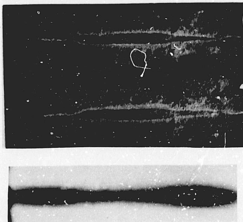
Figure 30. Radiograph and fracture surface macrograph of weld 2014-1.0-2A at 1X
