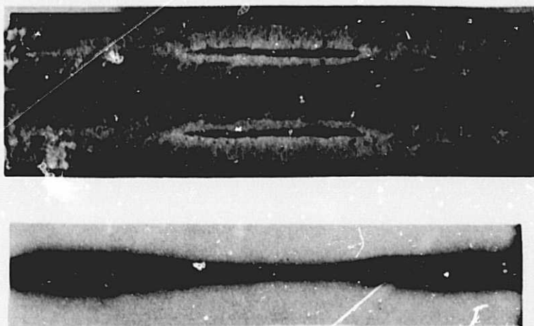
Figure 28. Radiograph and fracture surface macrograph of weld 2219-0.5-5B at IX.
