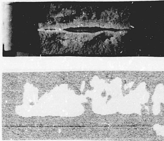
Figure 44. Delta scan recording and fracture surface of weld 2014-1.0-3D at IX.
