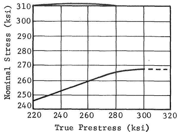
(e) -320°F Unaged Nominal Ultimate Response - Uniaxial
