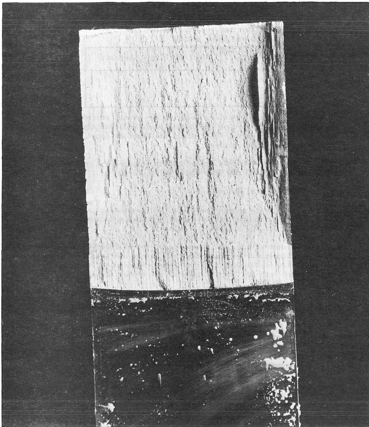
Fig. VI-32 Fracture Face of Parent-Metal X7007-T6 Compact-Tension Specimen
