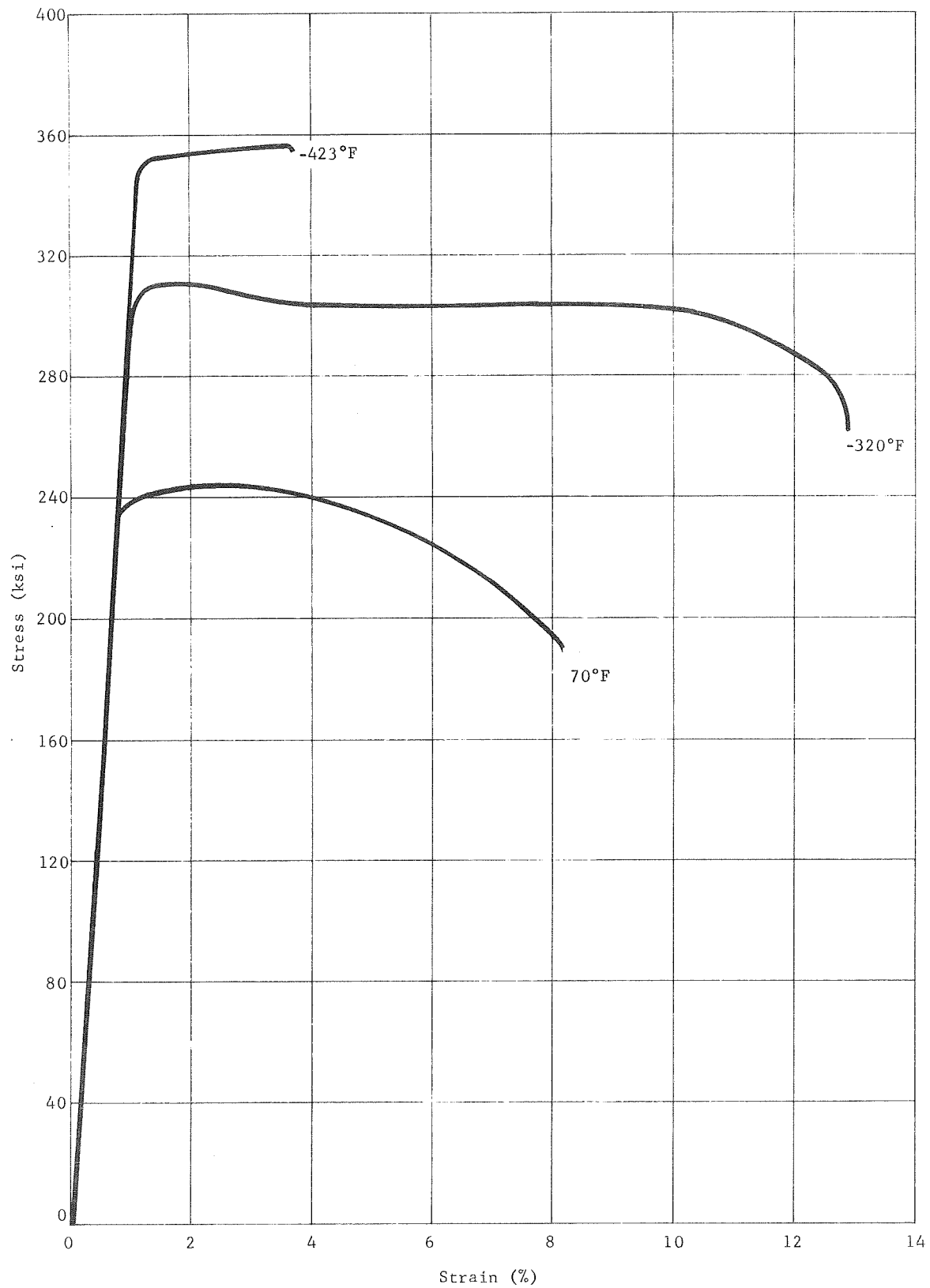
Fig. VI-22 Conventional Stress vs Strain Curve for Cryogenically-Stretched Parent Metal Specimens (Type 301 Stainless Steel; Longitudinal Direction)
