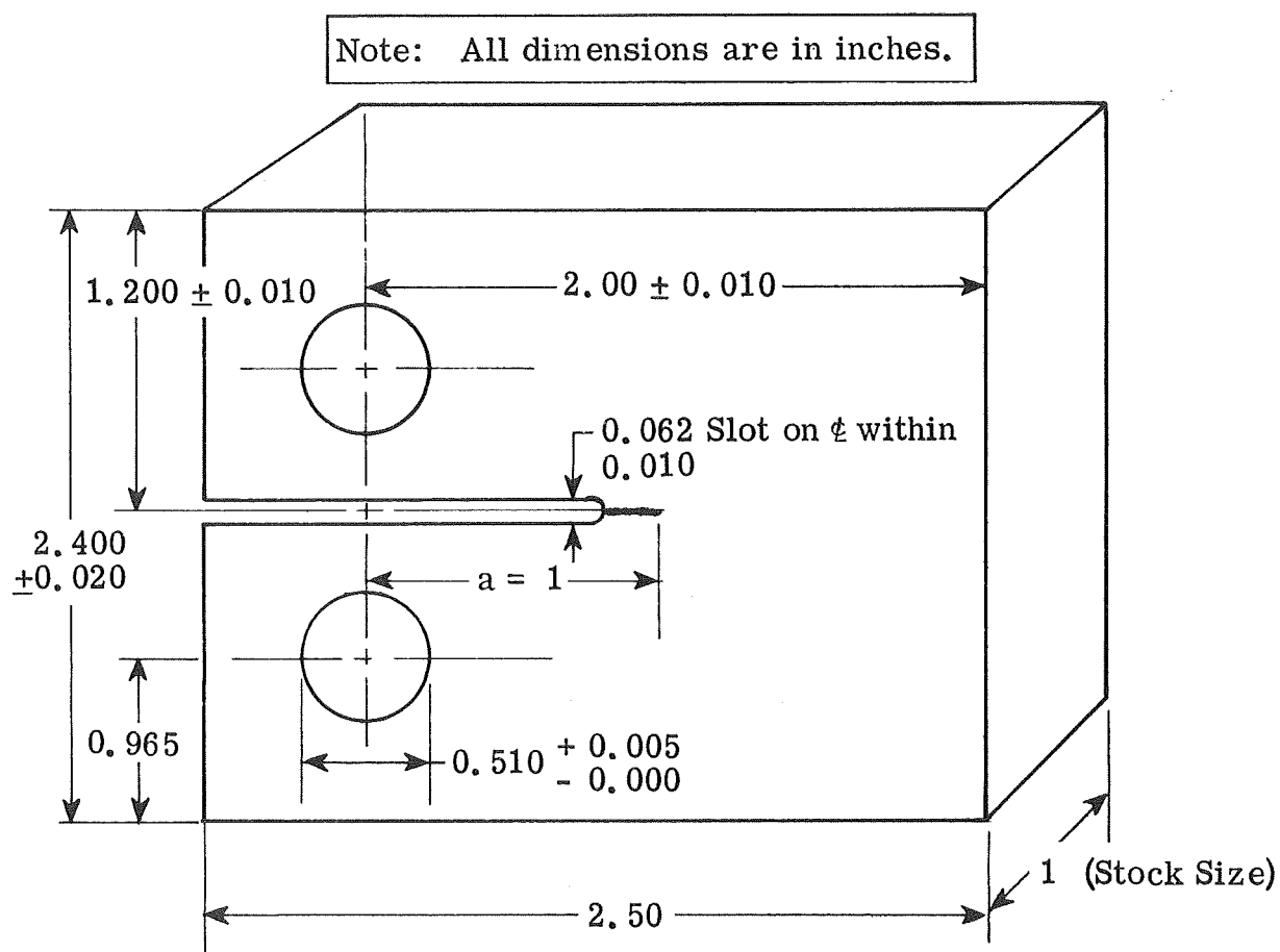
Fig. V-8 Specifications for Compact Tension Specimens
