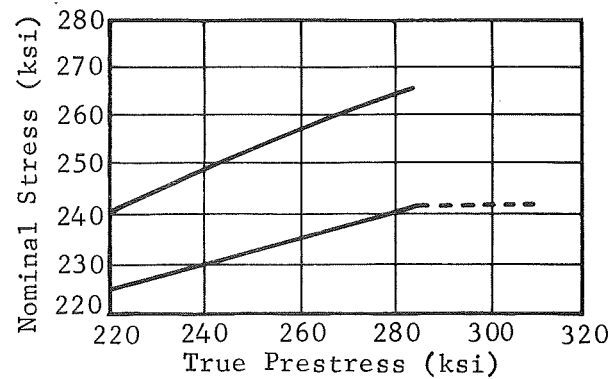
(b) Room Temperature, Aged Nominal Ultimate Response - Uniaxial
