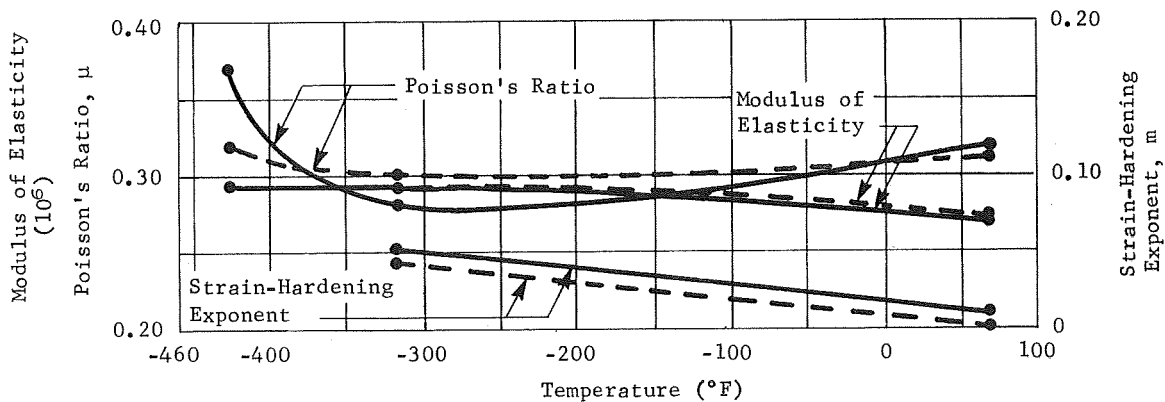
Fig. VI-20 Tensile Properties of Cryogenically-Stretched Parent Metal (Type 301 Stainless Steel)
