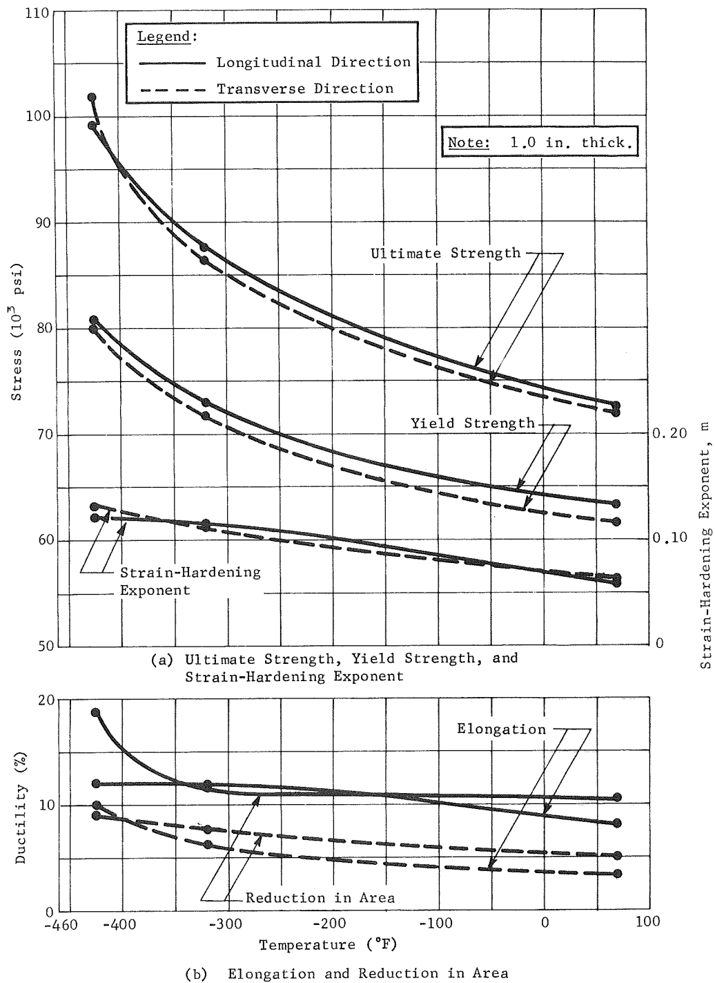
Fig. VI-1 Tensile Properties of Parent Metal (2021-T81 Aluminum Alloy)
