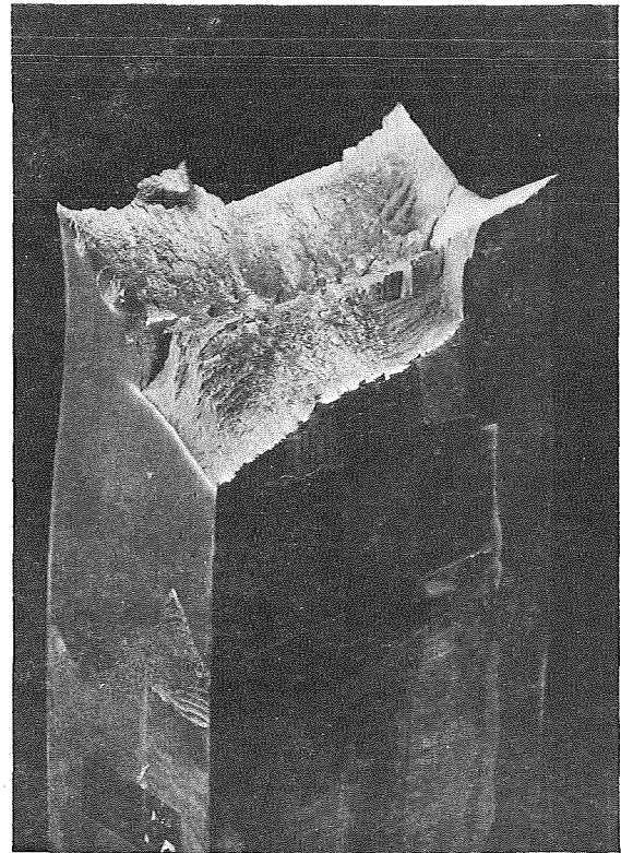
Fig. VI-4 Fractured Al X7007-T6 Tension Specimen, Load Applied in Longitudinal Direction, Temperature = 70^{\circ}\text{F}
