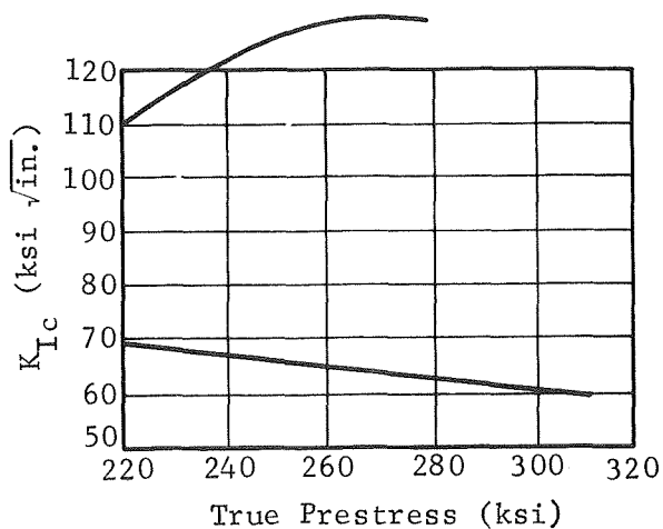
(f) Aged K_{Ic} at Room Temperature
