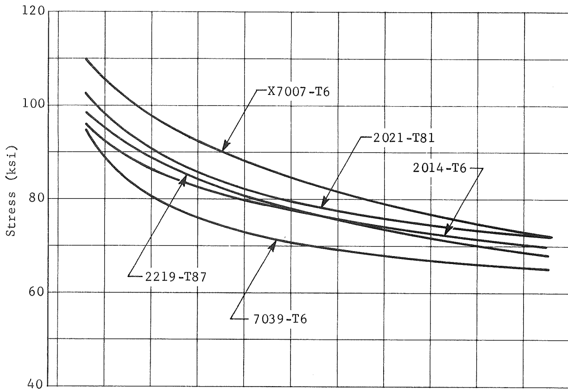
(a) Ultimate Strength
