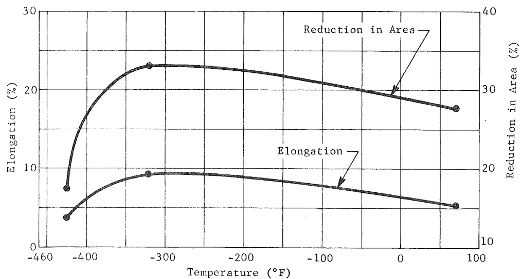
(b) Elongation and Reduction in Area
