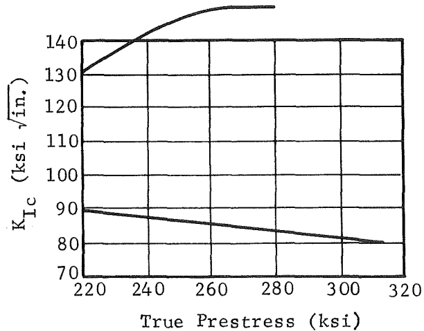
(g) Aged K_{Ic} at -320°F
