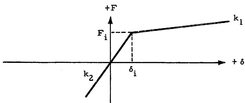
Fig. 12 - Joint Force-Displacement Relation
