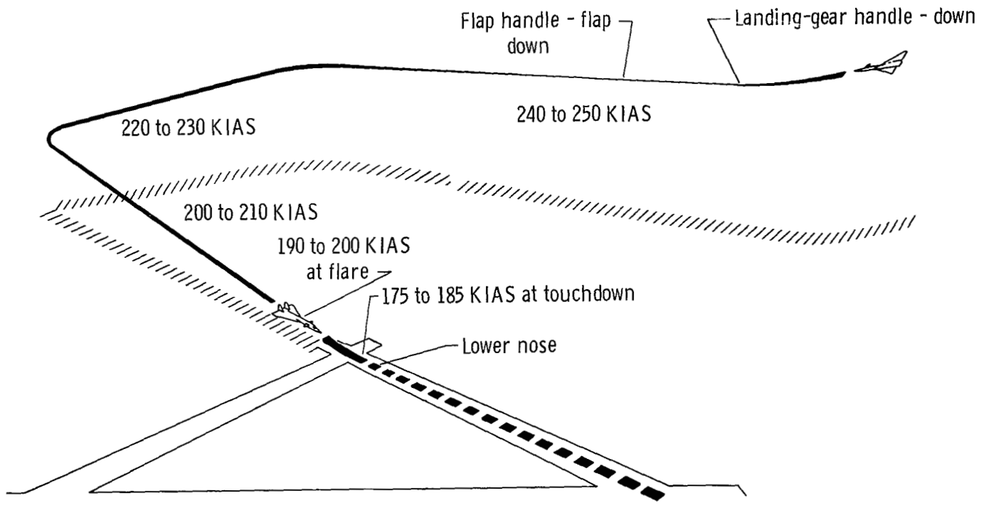
Figure 3. - Typical XB-70 landing pattern.
