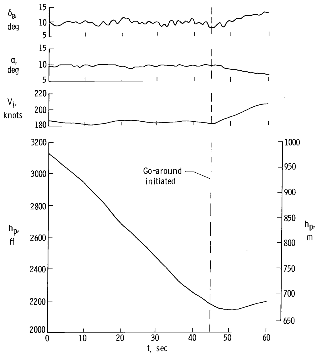
Figure 6. — Time history of XB-70 3° glide-slope approach at lower than recommended speed. V_{\text{appr}} = 185 KIAS, W = 311,000 lb (141,000 kg), center of gravity = 23.5 percent \bar{c} .
