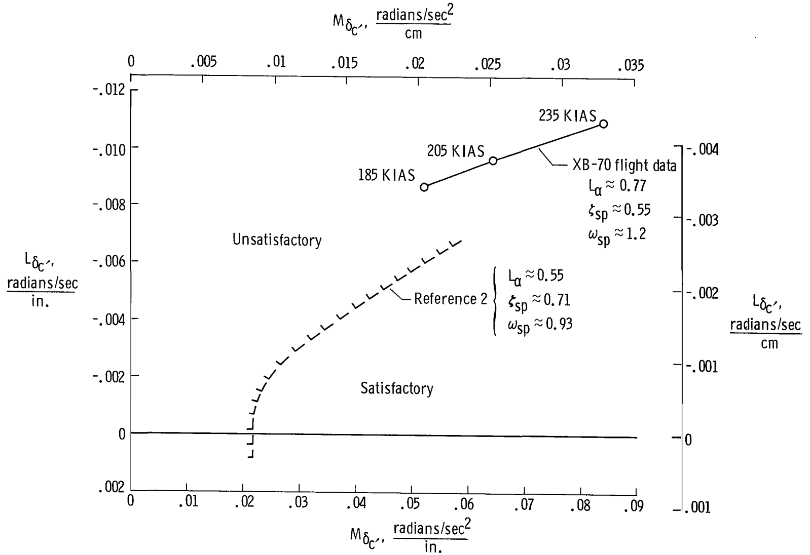
Figure 10. - Comparison of XB-70 longitudinal-control sensitivity with suggested longitudinal-control-sensitivity criterion for landing configuration.
