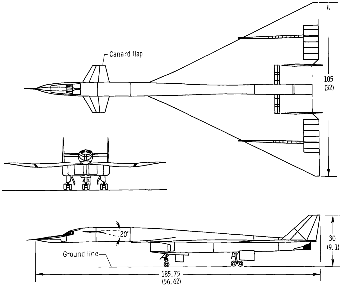
Figure 1.—XB-70 airplane. Landing configuration; dimensions in feet (meters) unless otherwise noted.
