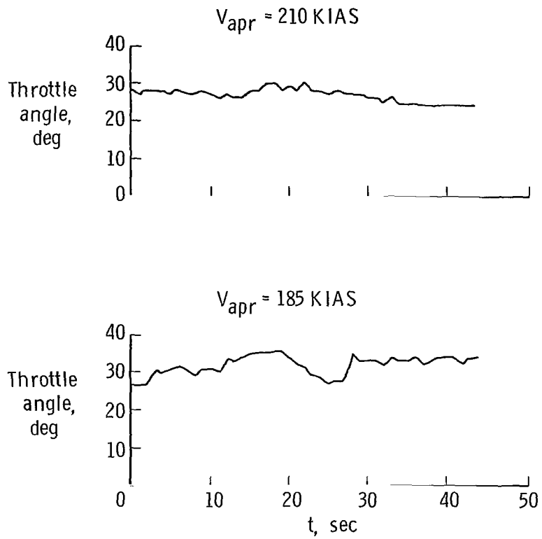
Figure 7. - Time history of throttle activity during XB-70 landing-approach maneuvers.
