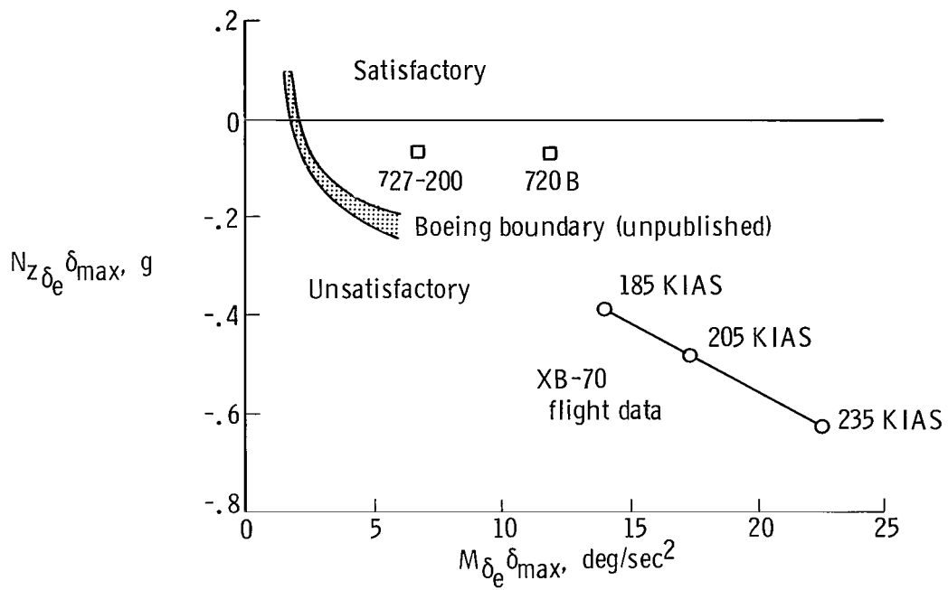
Figure 9. — Comparison of XB-70 control power with unpublished longitudinal-control-power criteria for the landing configuration.
