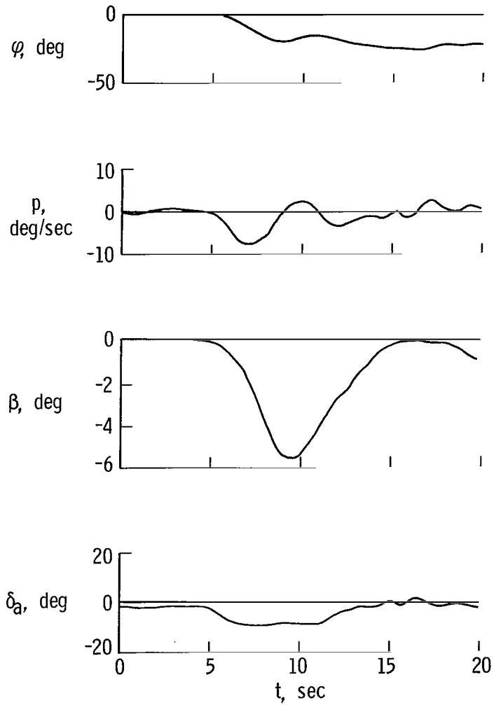
Figure 15.— Time history of XB-70 rudder-fixed, FACS-off, aileron roll. V_i = 230 knots; h_p = 10,000 ft (3050 m); center of gravity = 23.5 percent \bar{c} ; landing configuration.
