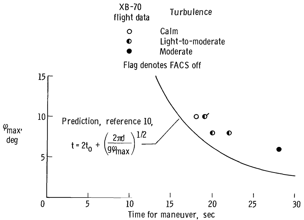
Figure 18.— Comparison of XB-70 flight results with predictions (ref. 10) of time to accomplish a sidestep maneuver during landing approach as a function of maximum bank angle used. 200-foot (61-meter) offset.
