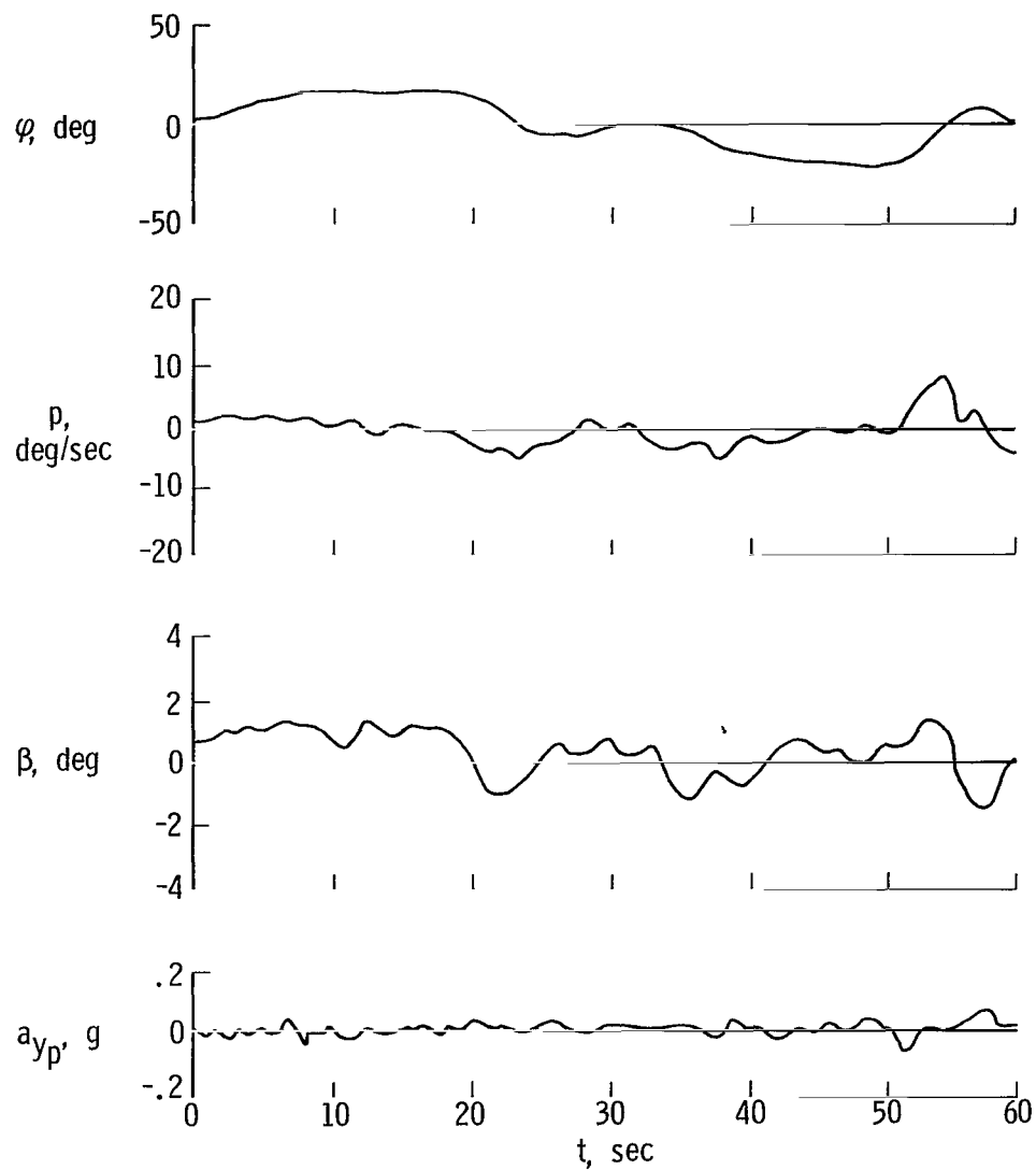
(a) \varphi , p , \beta , and a_{y_p} .
