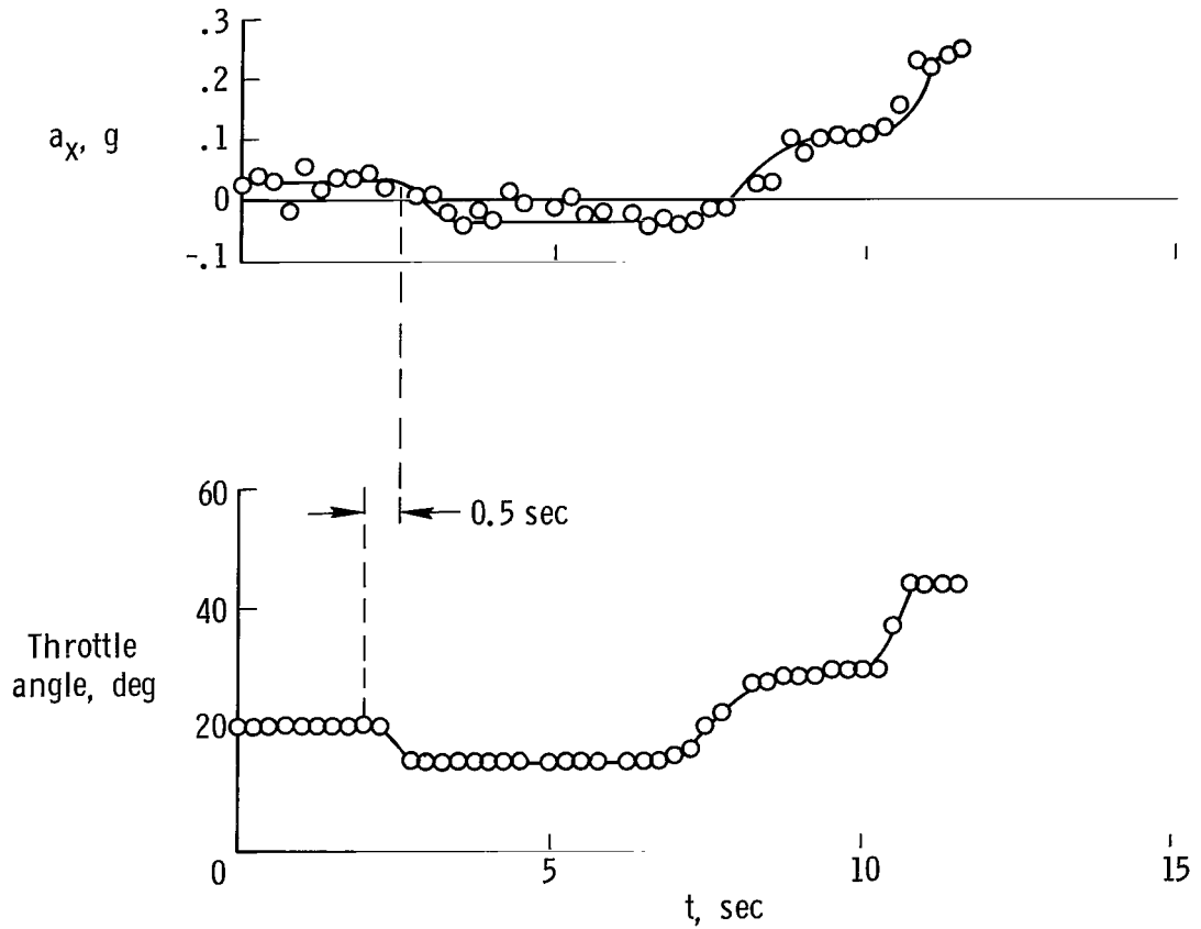
Figure 12. —XB-70 throttle response during a touch-and-go maneuver.
