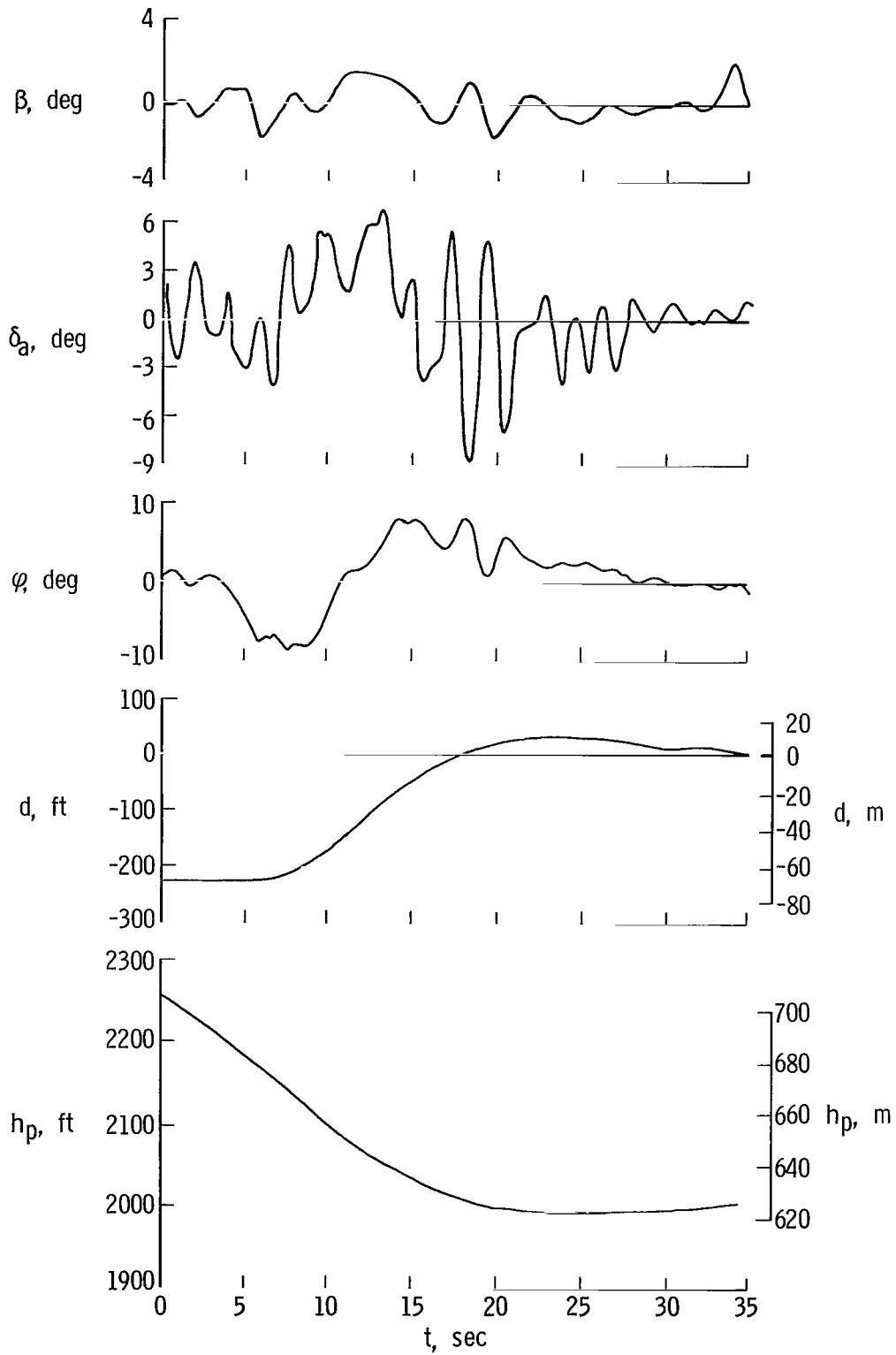
Figure 13. - Typical time history of an XB-70 lateral-offset maneuver. W = 446,000 \text{ lb (} 202,000 \text{ kg)} ; center of gravity = 23.5 percent \bar{c} .
