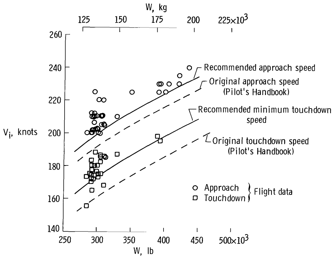
Figure 4. - Variation of XB-70 approach and touchdown speeds with gross weight.
