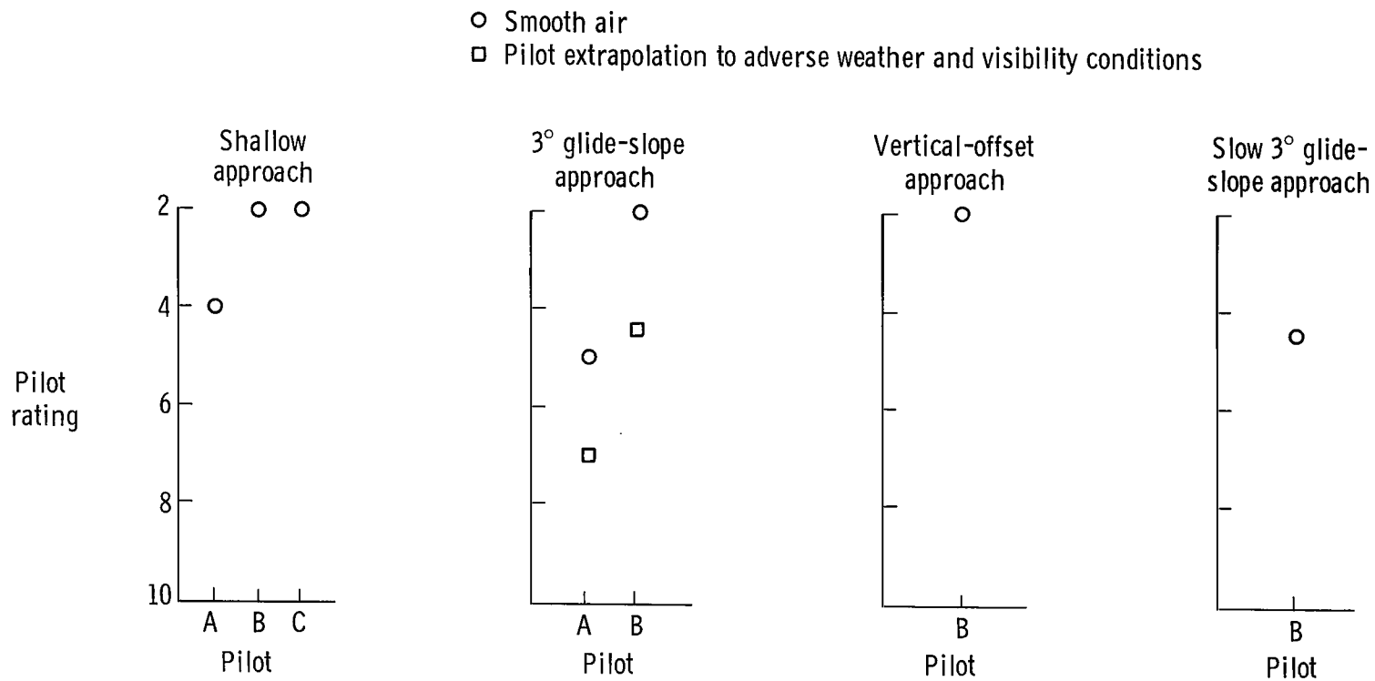
Figure 8. — Summary of pilot ratings of XB-70 longitudinal handling qualities.
