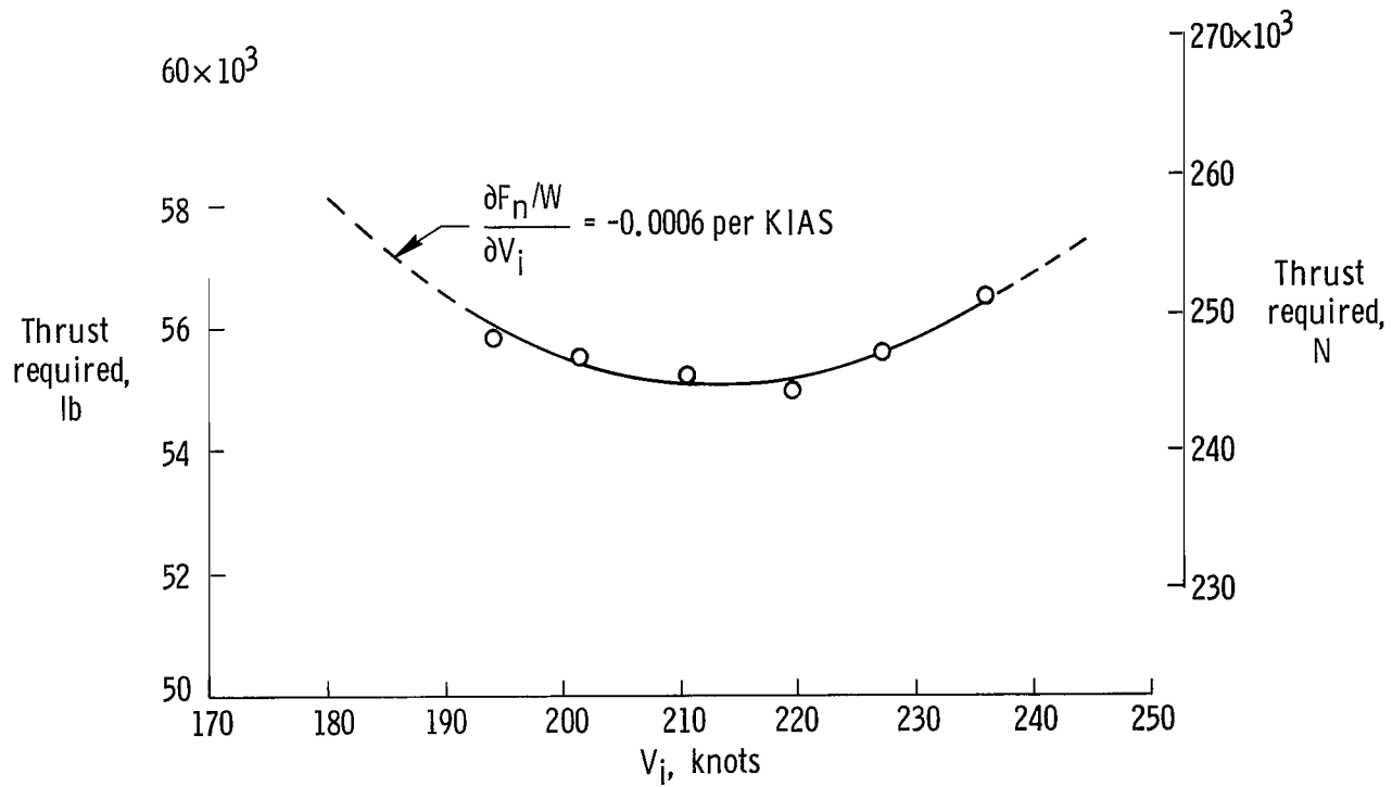
Figure 11. - XB-70 landing configuration speed-thrust variation. W = 300,000 lb (136,000 kg), center of gravity = 23.5 percent \bar{c} .
