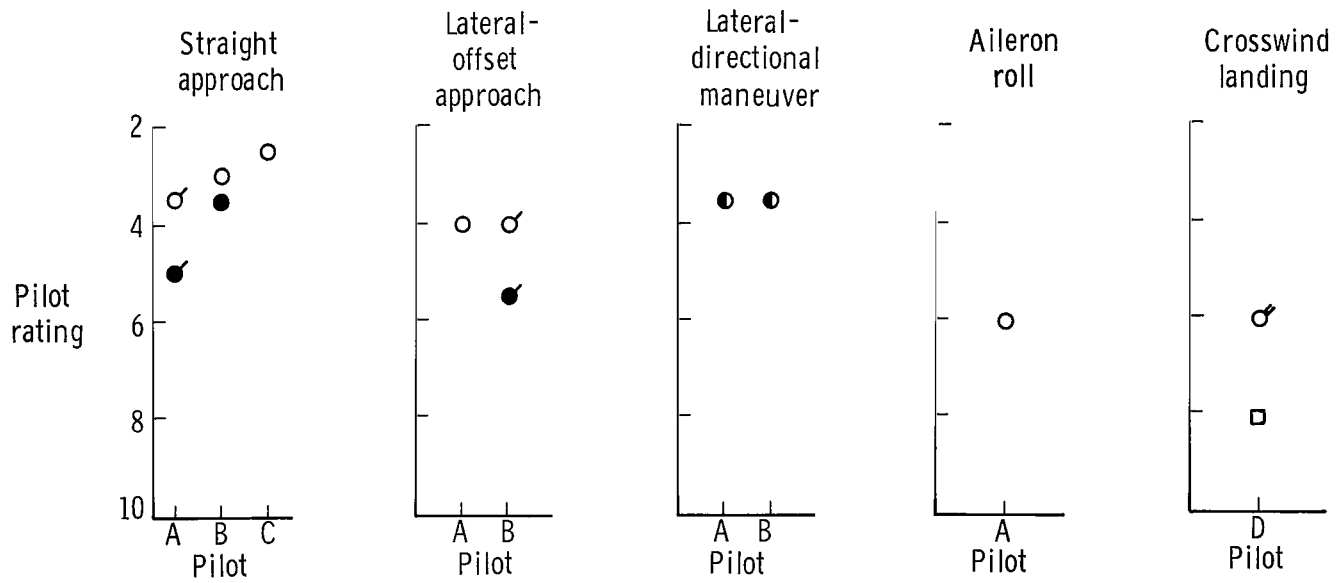
Figure 17. - Summary of pilot ratings of XB-70 lateral-directional characteristics.
