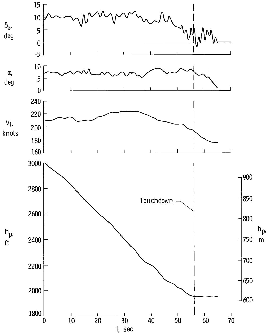
Figure 5. — Time history of typical XB-70 3° glide-slope approach and landing. V_{\text{appr}} = 210 KIAS, W = 310,000 lb (140,000 kg), center of gravity = 23.5 percent \bar{c} .
