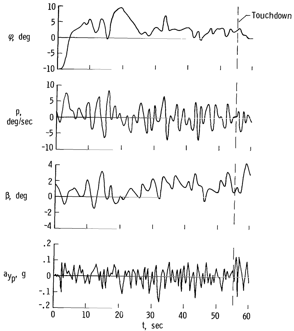
(c) \varphi , p , \beta , and a_{y_p} .
