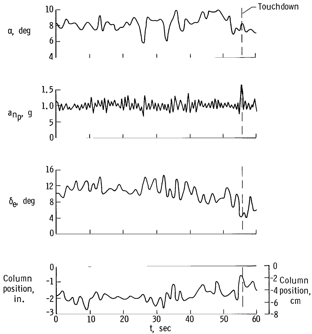
(b) \alpha , a_{np} , \delta_e , and column position.
