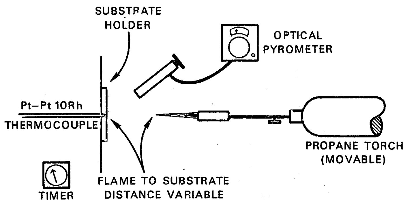
Figure 3. Top View Schematic of Flame Resistance Test
