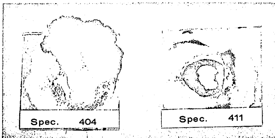
Figure 4. Appearance of Silicate Coatings After Exposure to 1800°F-2000°F Combustion Flame
