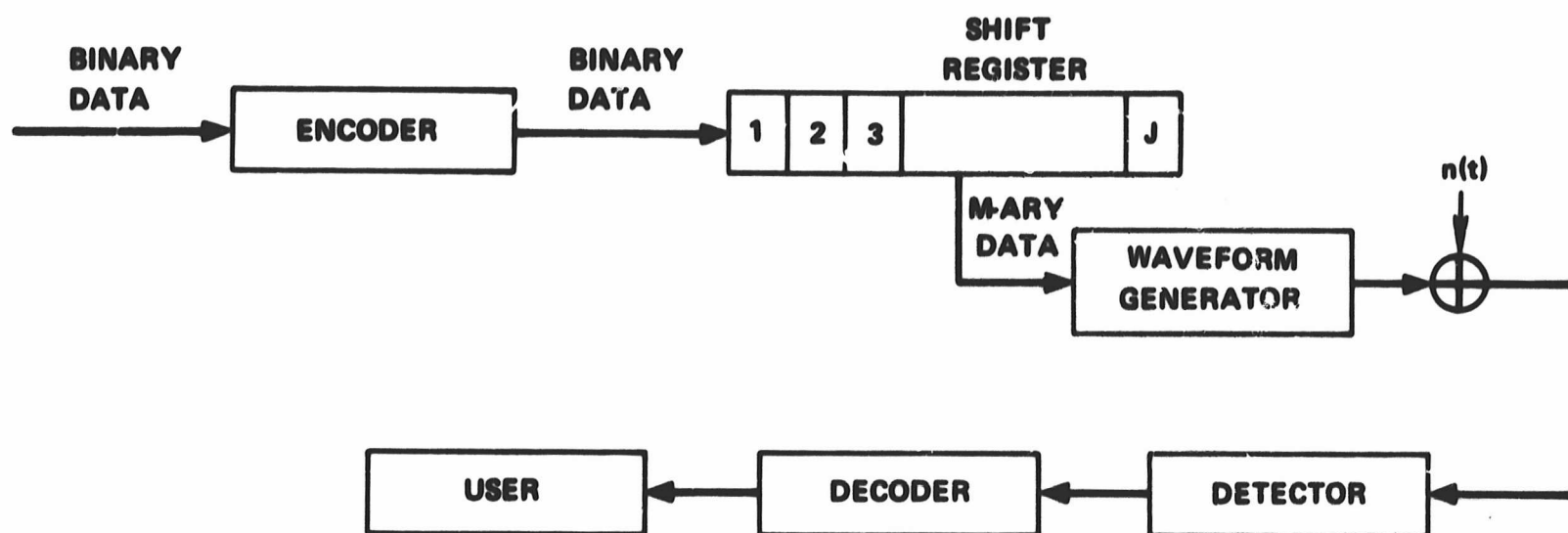
FIG. 1-1 SYSTEM BLOCK DIAGRAM
