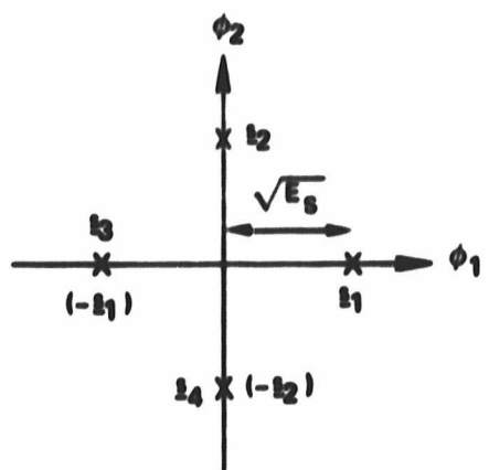
BIORTHOGONAL CODE, N = 2, M = 4
