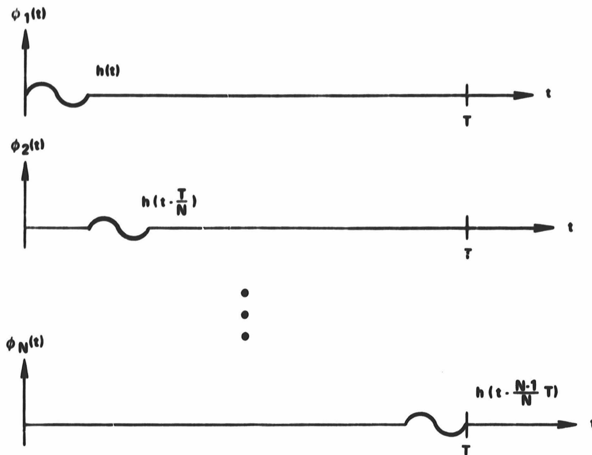
FIG. 4-3 TIME DISJOINT ORTHONORMAL WAVEFORMS
