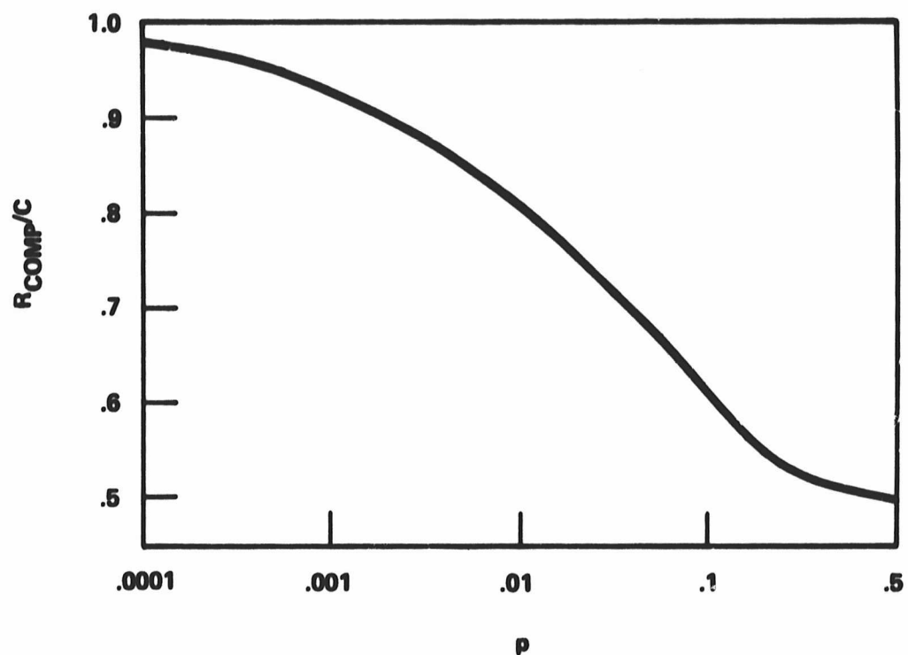
FIGURE 4 - 15 R_{COMP}/C AS A FUNCTION OF THE CROSSOVER PROBABILITY, p , OF A BINARY SYMMETRIC CHANNEL.
