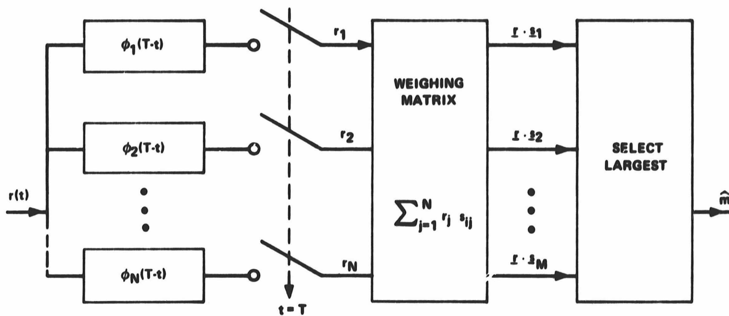
FIG. 4-2 ALTERNATE REALIZATION OF OPTIMUM DETECTOR FOR WAVEFORM CODE
