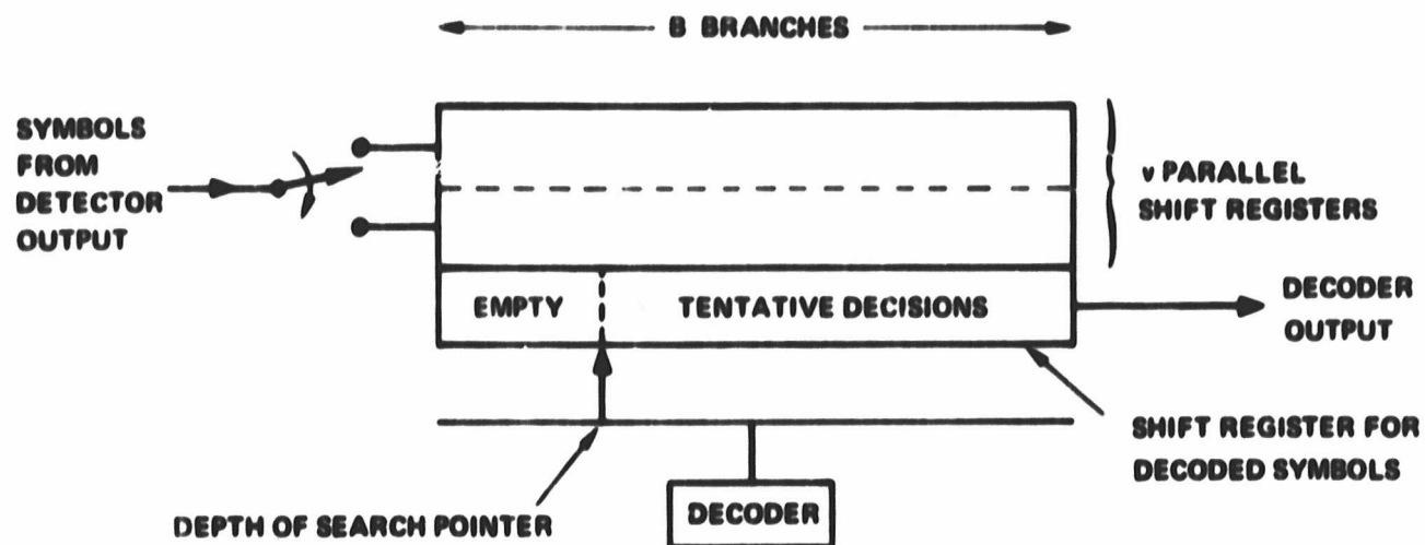
FIGURE 4 - 18 BUFFER FOR SEQUENTIAL DECODER
