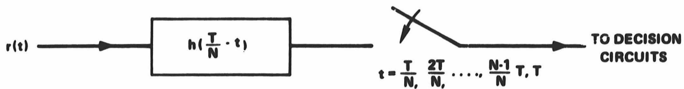
FIGURE 4 - 4 OPTIMUM RECEIVER FOR TIME DISJOINT PULSE WAVEFORMS
