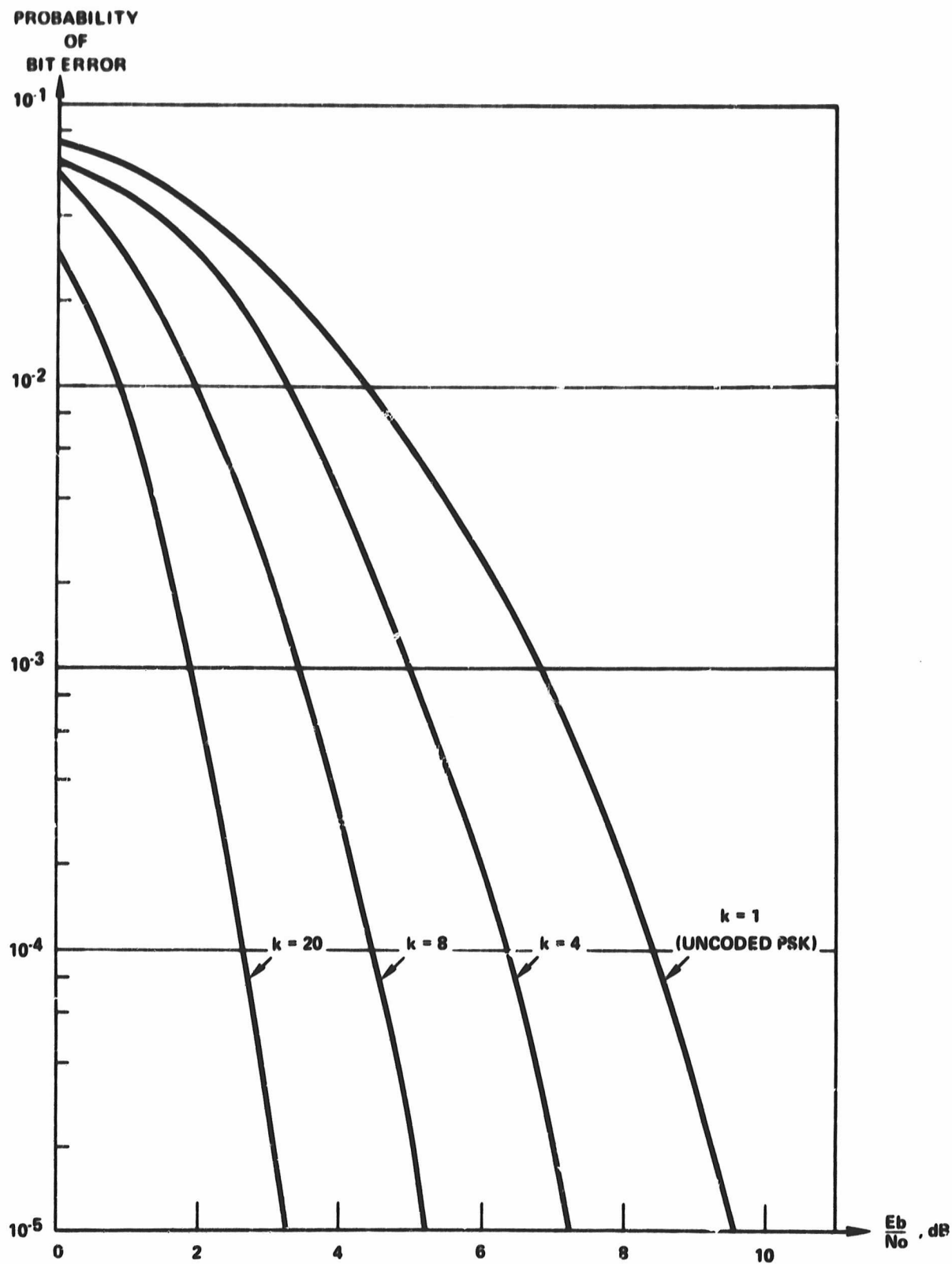
FIGURE 4-8 PROBABILITY OF BIT ERROR VS. \frac{E_b}{N_0} FOR BIORTHOGONAL CODES
