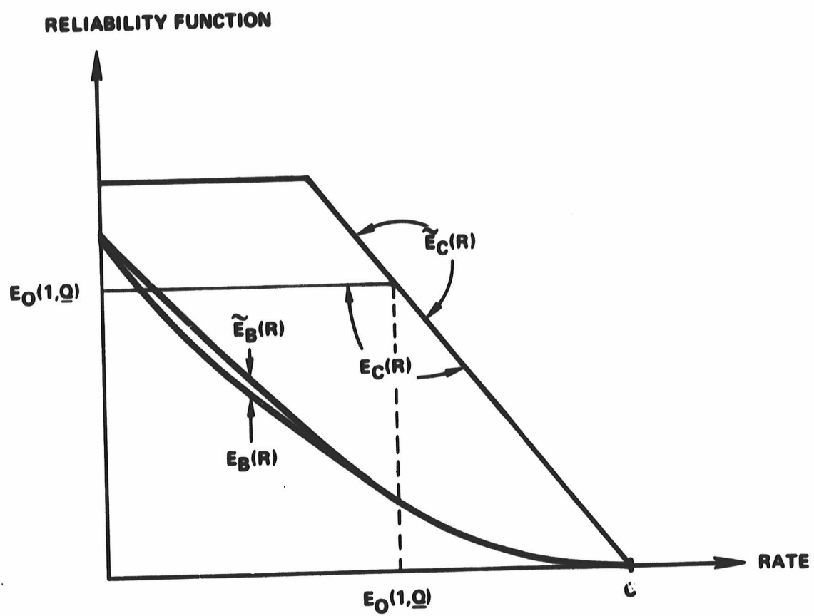
FIG. 3-2 BLOCK AND CONVOLUTIONAL RELIABILITY FUNCTIONS
