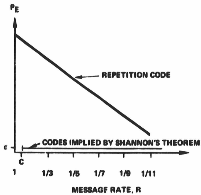
FIG. 2-4 PERFORMANCE OF REPETITION CODE
