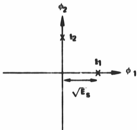
ORTHOGONAL CODE, N = M = 2
