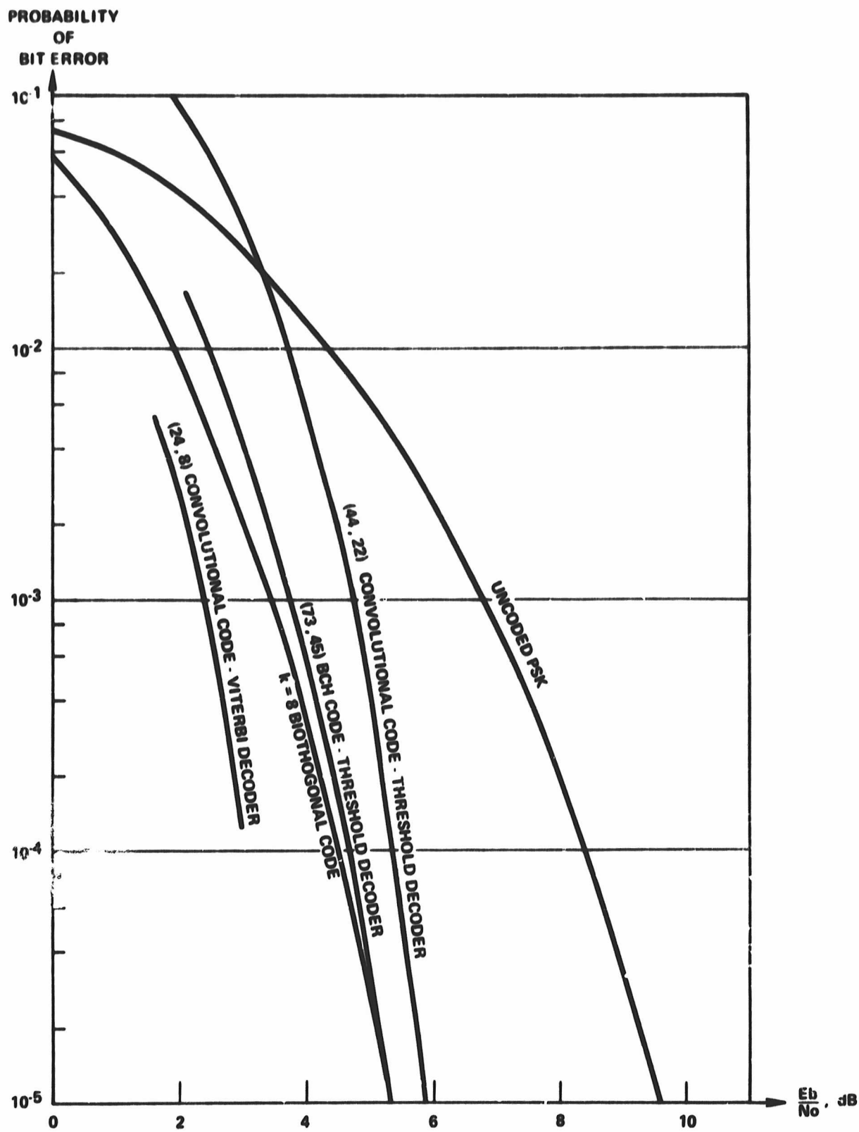
FIGURE 4 - 11 PROBABILITY OF BIT ERROR VS. \frac{E_b}{N_0} FOR VARIOUS CODES AND DECODERS
