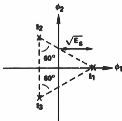
TRANSORTHOGONAL CODE, N = 2, M = 3
