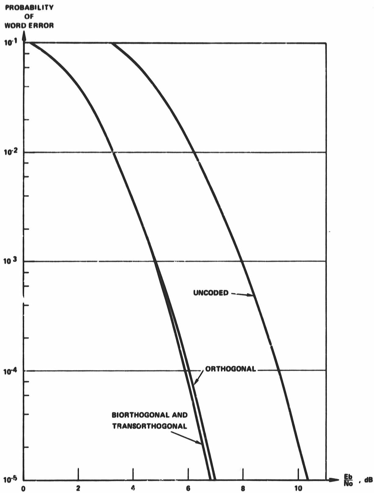
FIGURE 4 - 7 PROBABILITY OF WORD ERROR VS. \frac{E_b}{N_0} FOR k = 5 WAVEFORM CODES
