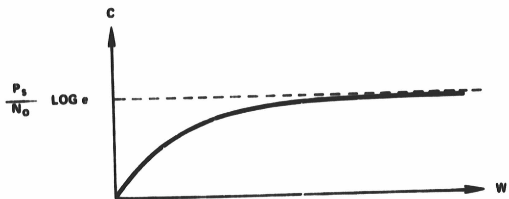
FIG. 3-1 CAPACITY OF WHITE GAUSSIAN CHANNEL WITH BANDWIDTH W
