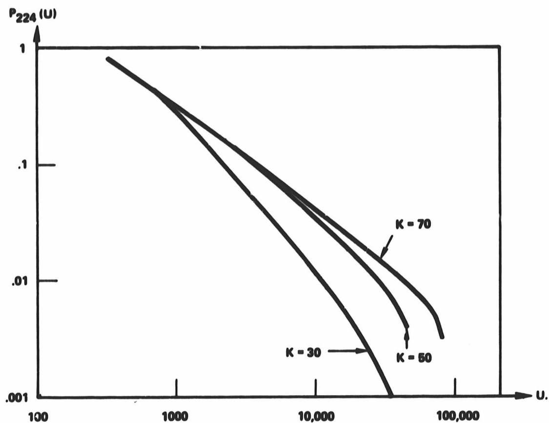
FIGURE 4 - 19 PROBABILITY THAT NUMBER OF COMPUTATIONS REQUIRED TO DECODE 224 BRANCHES EXCEEDS U.
