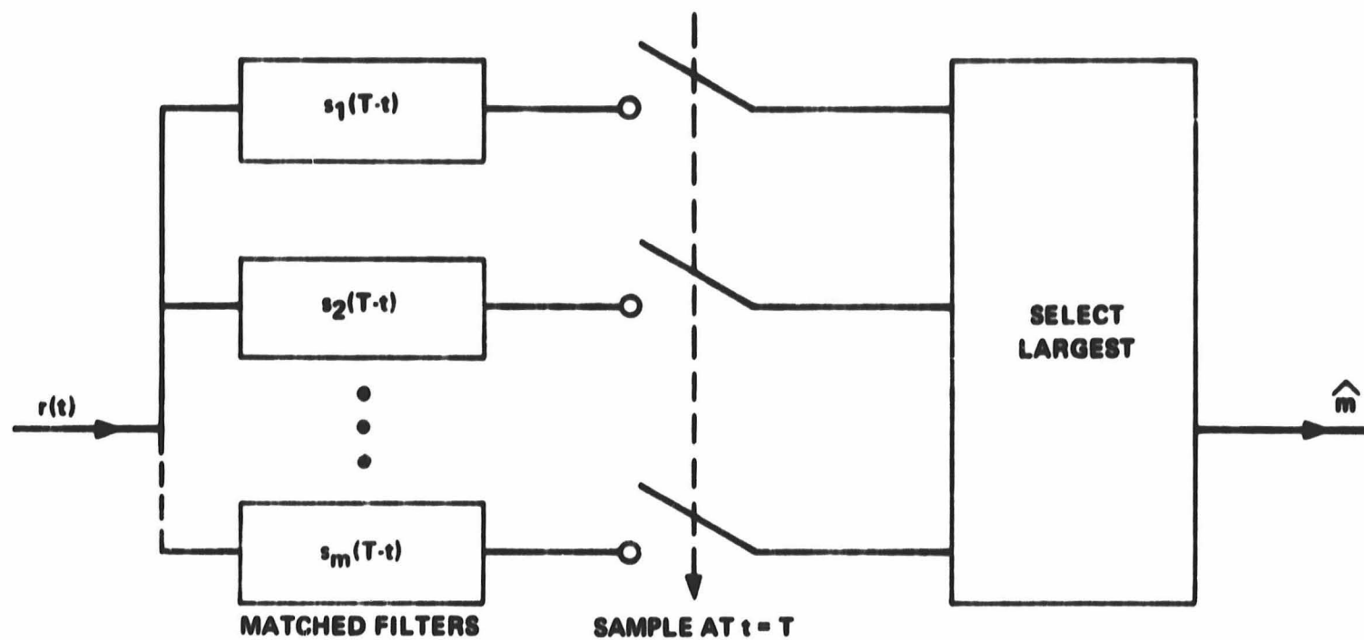
FIG. 4-1 OPTIMUM DETECTOR FOR WAVEFORM CODE
