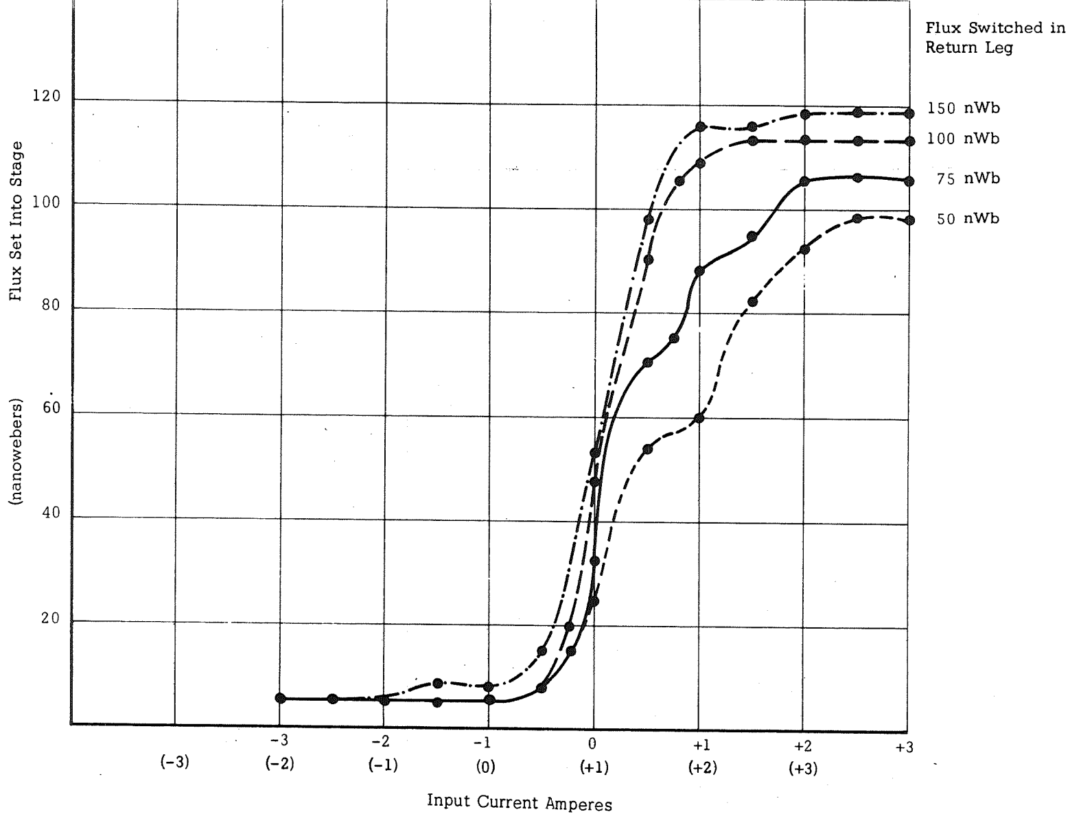
Fig. 25 Flux Set Into a Stage as a Function of Input Current
