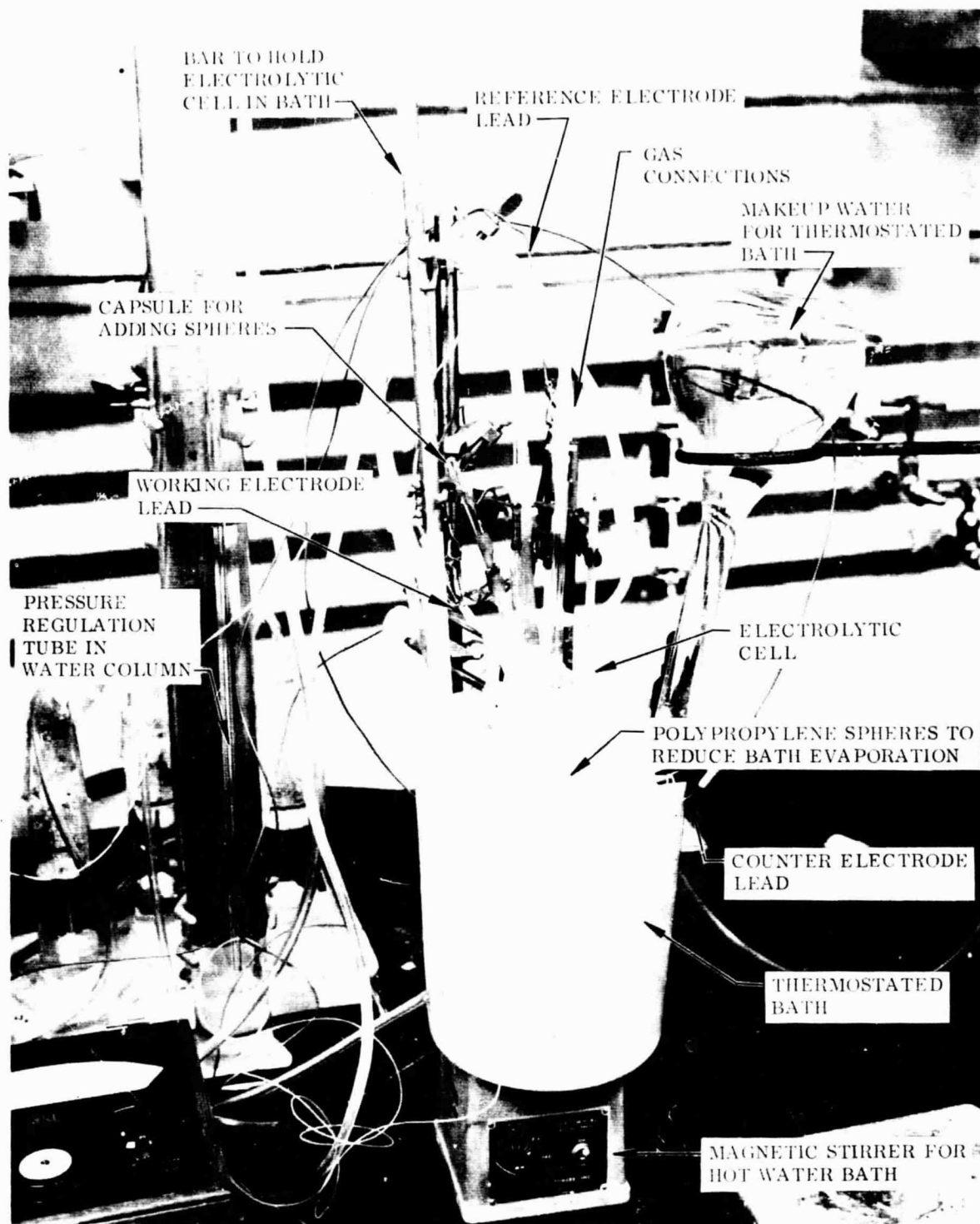
Fig. 5 Electrolytic Cell in Operation in Thermostated Bath
