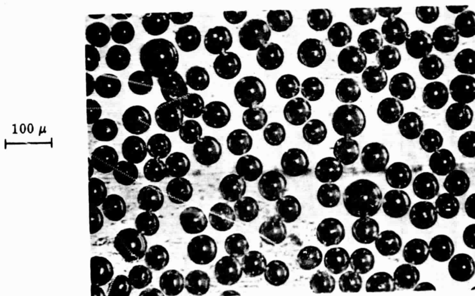
Fig. 15 Silver Spheres, 86-μ Average Diameter
