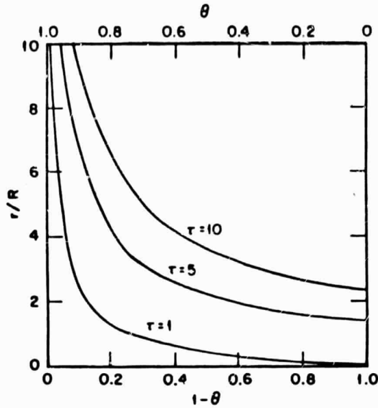
Fig. 73 Variation of Ratio of Pore Radius to Sphere Radius With Changes in Tortuosity Factor and Fractional Void Volume
