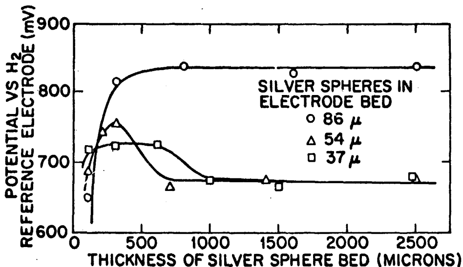
Fig. 31 Effect of Electrode Thickness on Electrode Potential for Various Sphere Sizes. Oxygen Differential Pressure, -2 25 cm of Water; Cathodic Current Density, 4.2 mA cm -2
