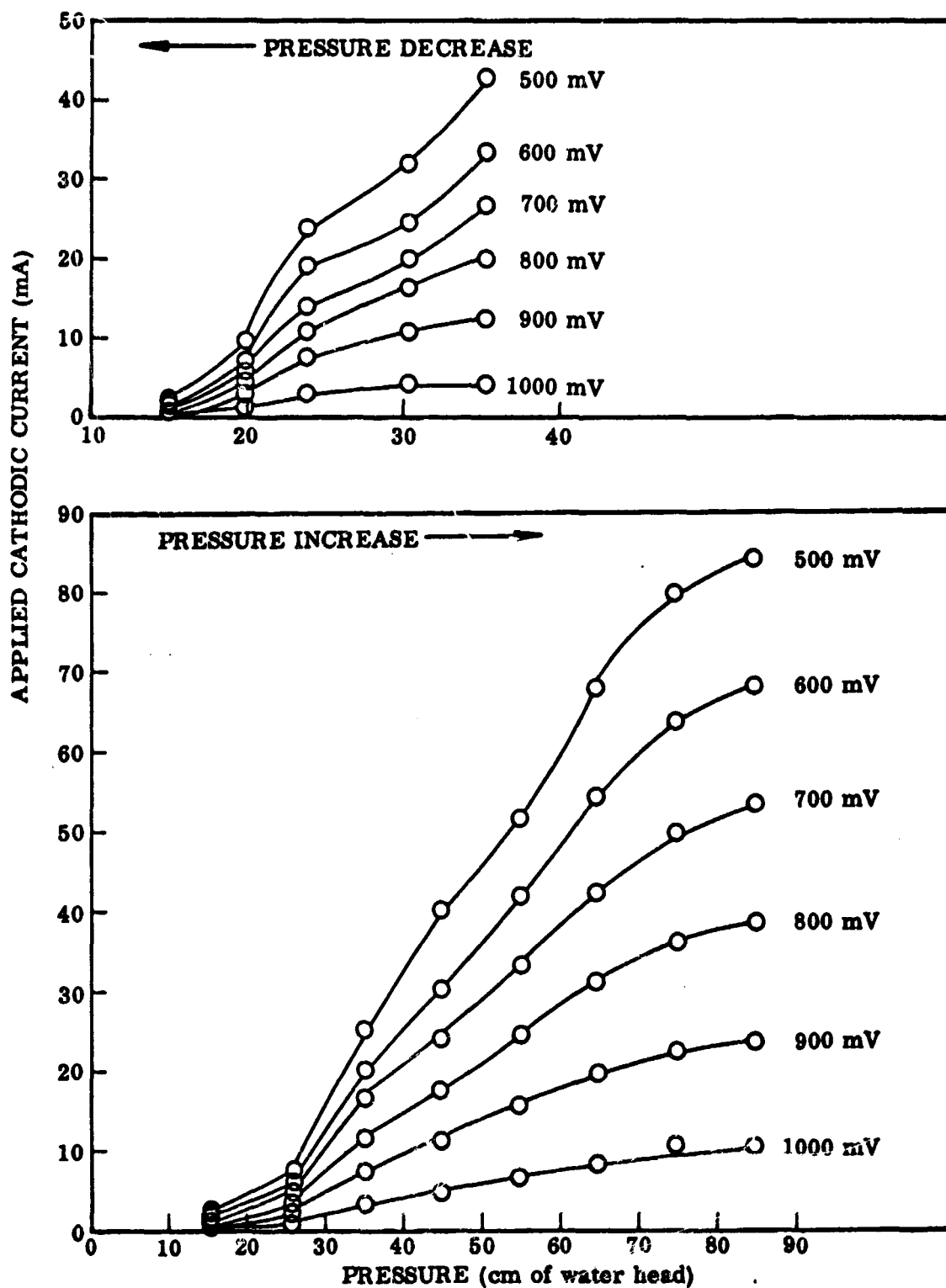
Fig. 42 Silver Sphere Bed With 10 mg of Platinum in Coarse Layer
