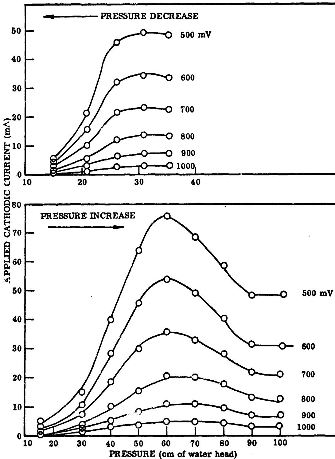
Fig. 41 Silver Spherc Bed With No Platinum in Coarse Layer
