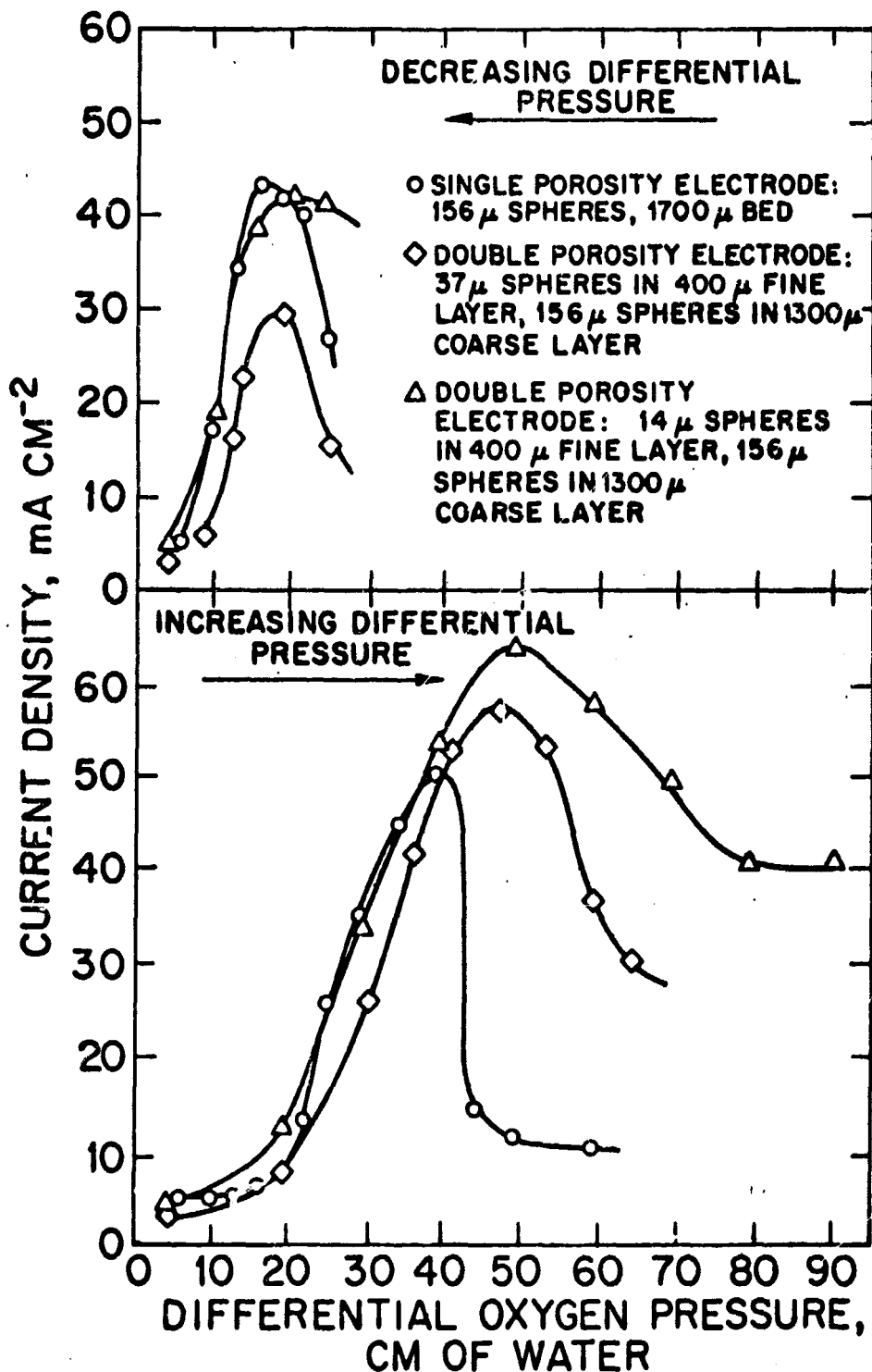
Fig. 36 Comparison of Single- and Double-Porosity Electrodes as Differential Pressure Is Changed. Silver Sphere Beds With Total Thickness at 1700 \mu at Potential of 500 mV Versus Hydrogen Reference Electrode
