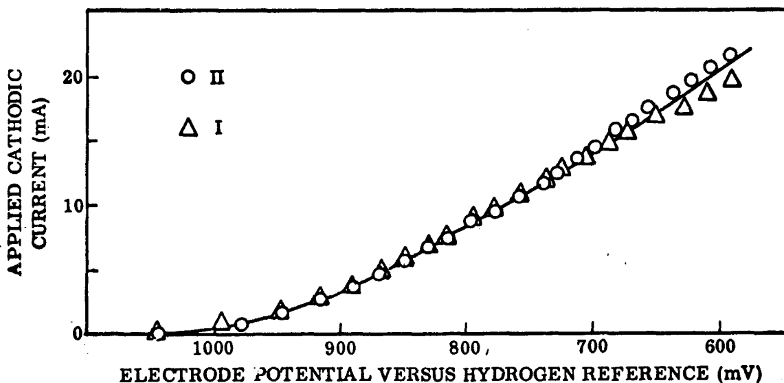
Fig. 39 Performance of Triple-Porosity Electrode Structures. Structure I With Coarse Side Toward Electrolyte; Structure II With Fine Side Toward Electrolyte
