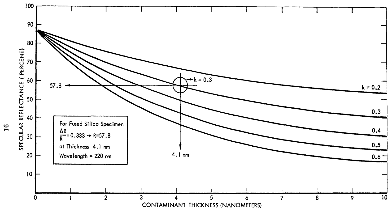
Figure 43: REFLECTANCE OF MIRROR COATED WITH Al + 25 NM \text{MgF}_2 + CONTAMINANT FILM WITH COMPLEX REFRACTIVE INDEX (1.40 - ik)
