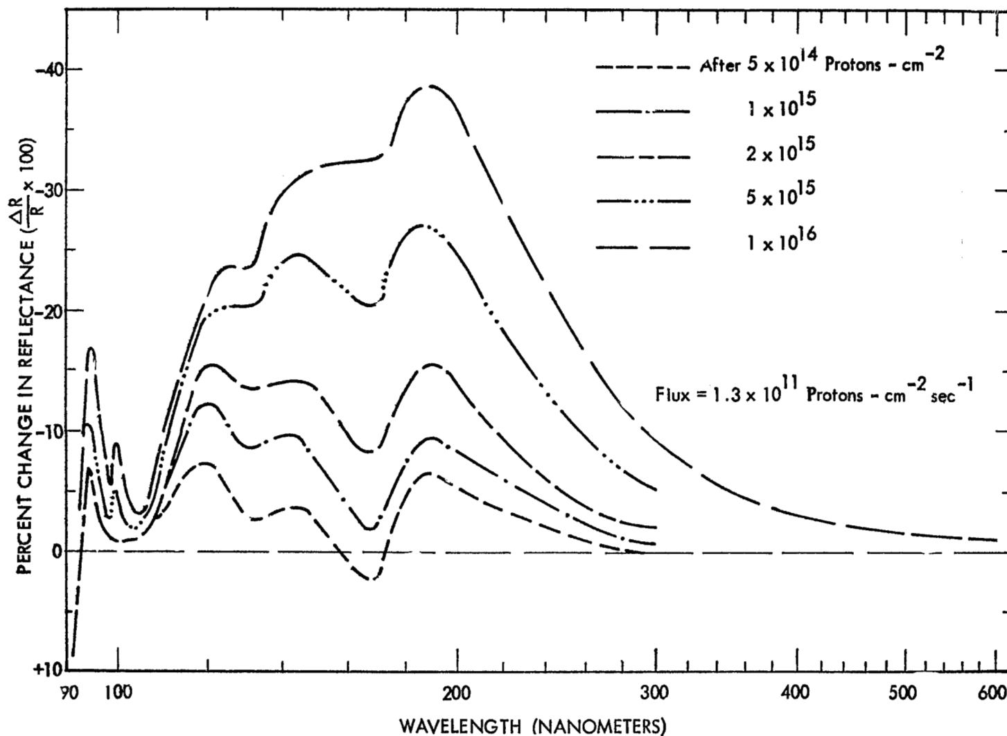
Figure 19: REFLECTANCE CHANGES OF A LiF/Al-COATED FUSED SILICA MIRROR IRRADIATED BY 10 KEV PROTONS
