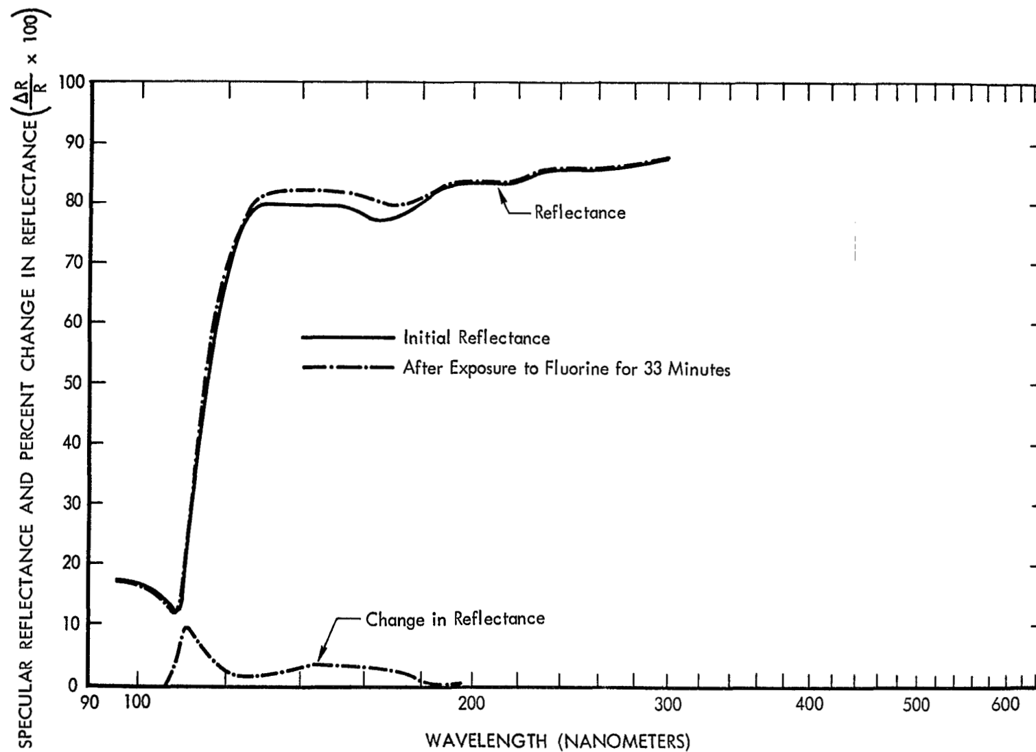
Figure 33: EFFECT OF FLUORINE EXPOSURE ON REFLECTANCE OF AN UNIRRADIATED \text{MgF}_2/\text{Al} -COATED MIRROR
