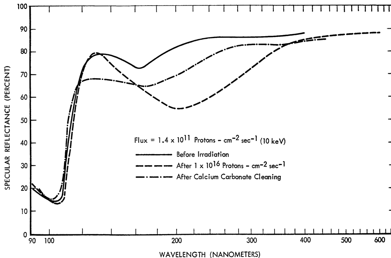
Figure 30: EFFECT OF ABRASIVE CLEANING ON REFLECTANCE OF AN IRRADIATED \text{MgF}_2/\text{Al} -COATED MIRROR
