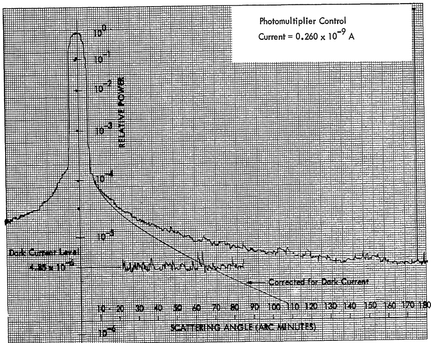
Figure 16: TYPICAL SCATTERED LIGHT DATA FOR AN UNIRRADIATED \text{MgF}_2/\text{Al} -COATED FUSED SILICA MIRROR AT 253.7 NM WAVELENGTH
