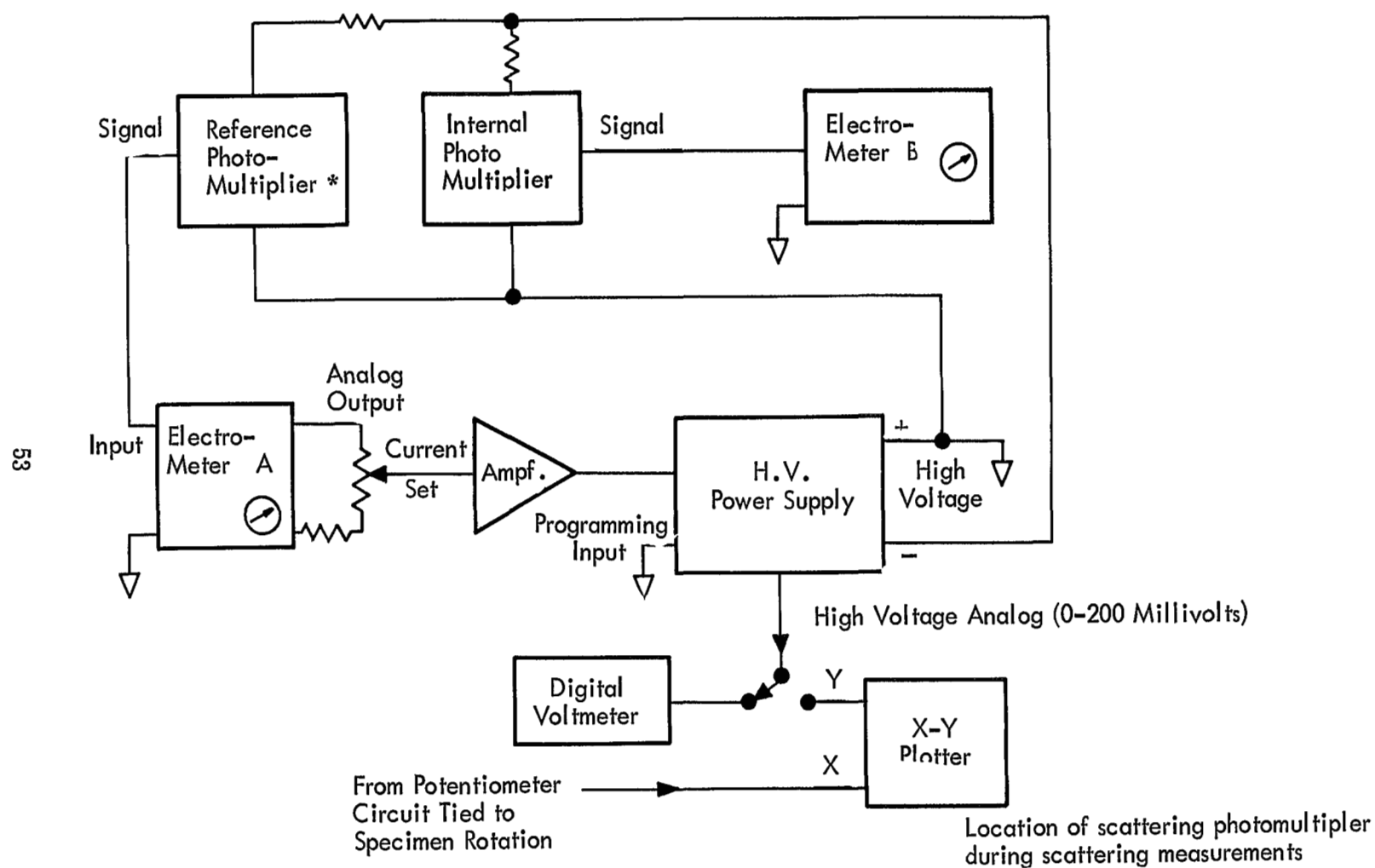
Figure 5: REFLECTOMETER/SCATTERING MEASUREMENT ELECTRONICS
