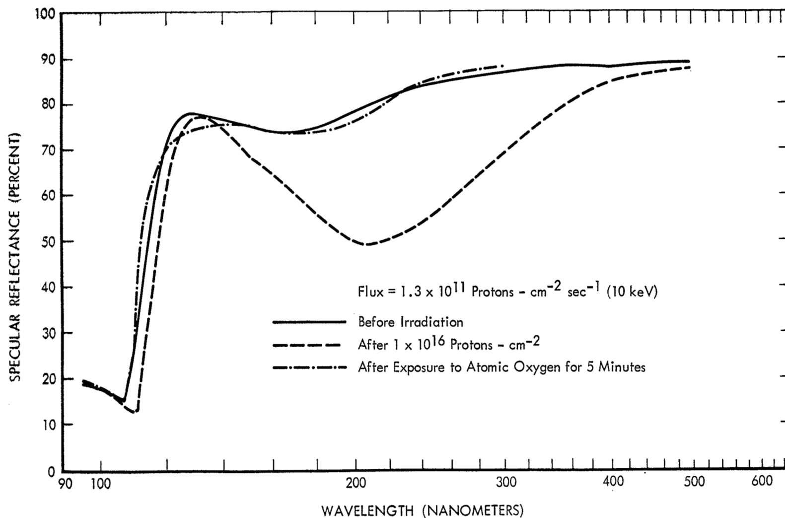
Figure 34: REFLECTANCE RECOVERY OF AN IRRADIATED \text{MgF}_2/\text{Al} -COATED CER-VIT MIRROR EXPOSED TO ATOMIC OXYGEN
