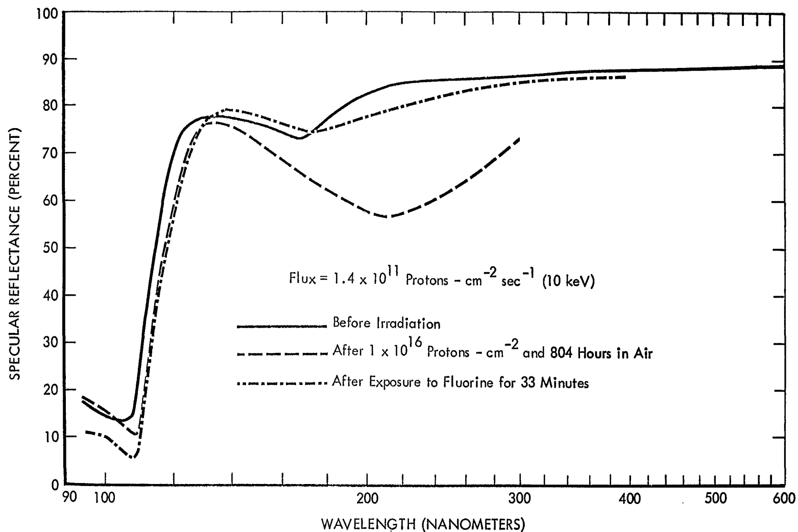
Figure 31: REFLECTANCE RECOVERY OF AN IRRADIATED \text{MgF}_2/\text{Al} -COATED CER-VIT MIRROR EXPOSED TO FLUORINE
