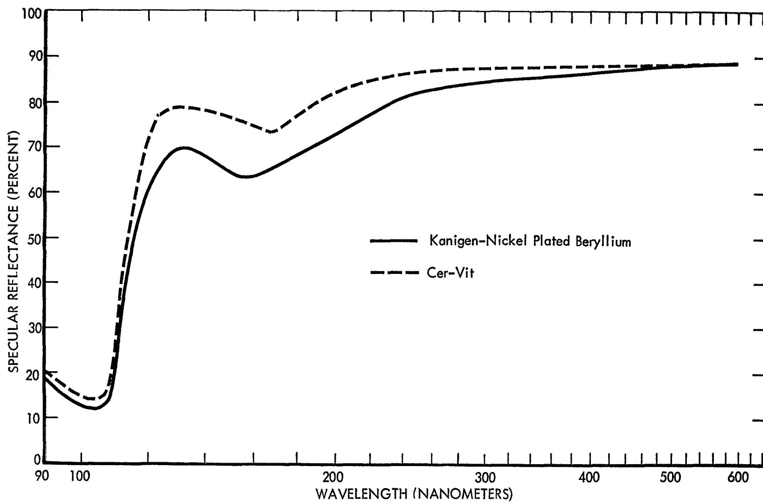
Figure 13: REFLECTANCE COMPARISON OF \text{MgF}_2/\text{Al} -COATED BERYLLIUM AND CER-VIT MIRRORS
