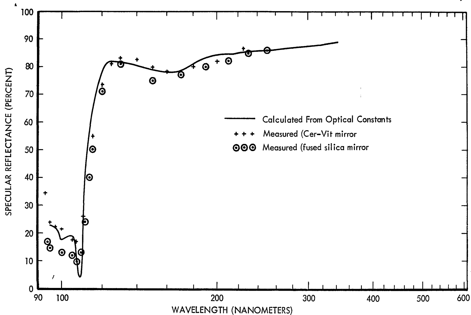
Figure 4I: CALCULATED AND MEASURED REFLECTANCE OF \text{MgF}_2/\text{Al} - COATED MIRRORS(25 NM OF \text{MgF}_2 )
