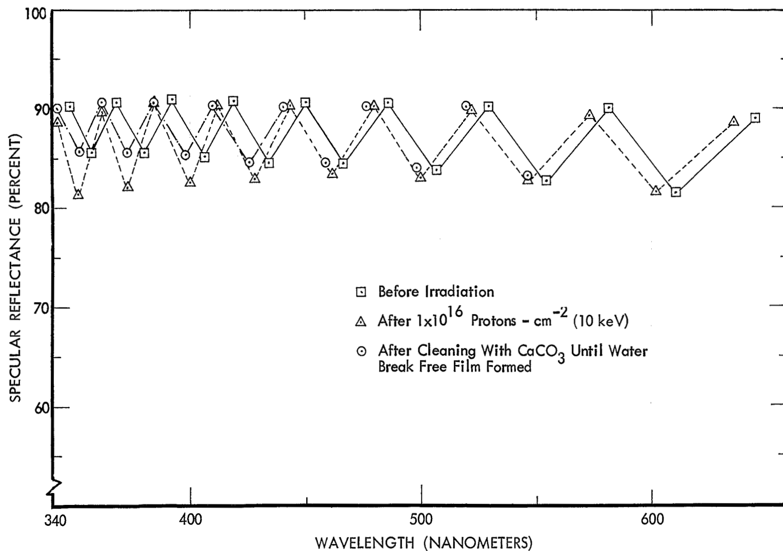
Figure 24: EFFECT OF IRRADIATION AND CLEANING ON INTERFERENCE CHARACTERISTICS OF \text{SiO}_2/\text{Al} -COATED MIRROR
