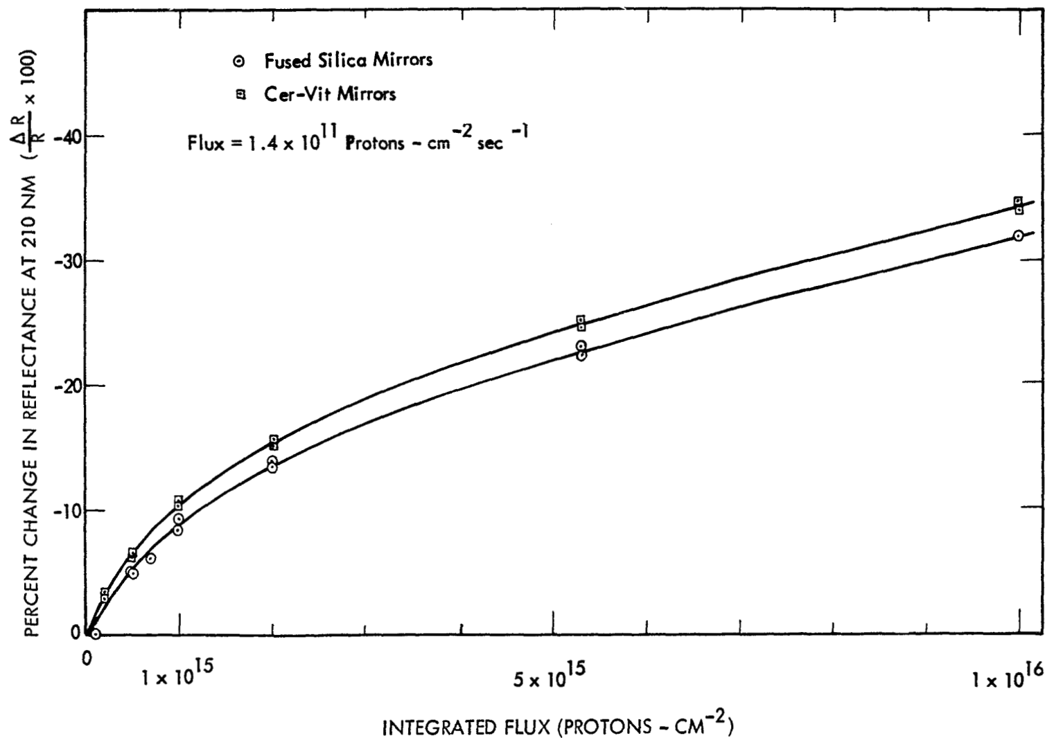
Figure 8: DIFFERENCE IN RADIATION DAMAGE OF \text{MgF}_2/\text{Al} -COATED MIRRORS AS SHOWN BY REFLECTANCE CHANGES AT 210 NM
