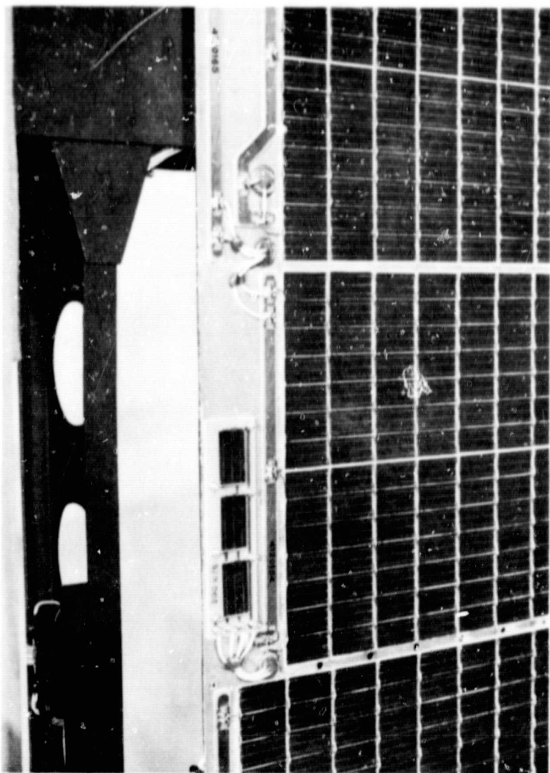
Fig. 5. Closeup of I_{sc} - V_{oc} transducer
