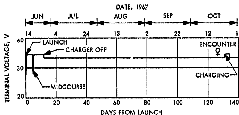
Fig. 41. Battery terminal voltage; launch to end of mission
