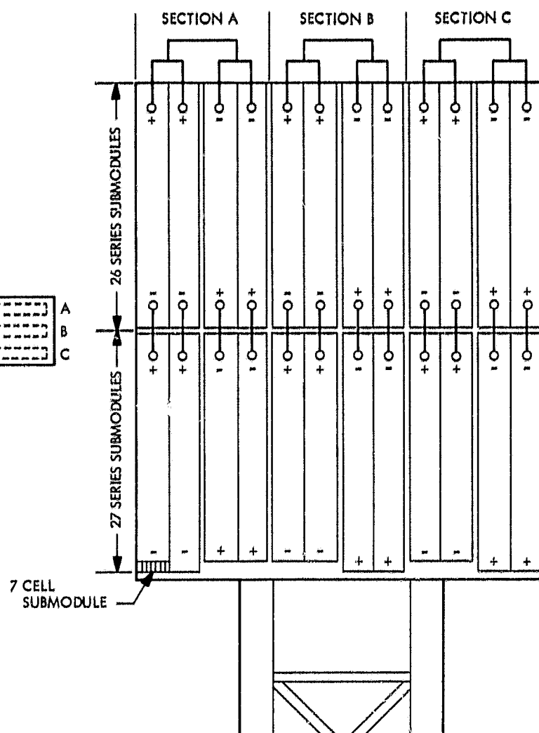
Fig. 1. Mariner Venus 67 solar panel
