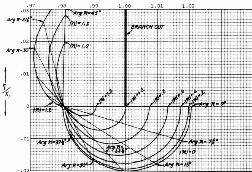
b) POLE LOCATION IS \frac{K}{K_1} PLANE AS A FUNCTION OF |n| AND \text{Arg } n, |V| = .2
