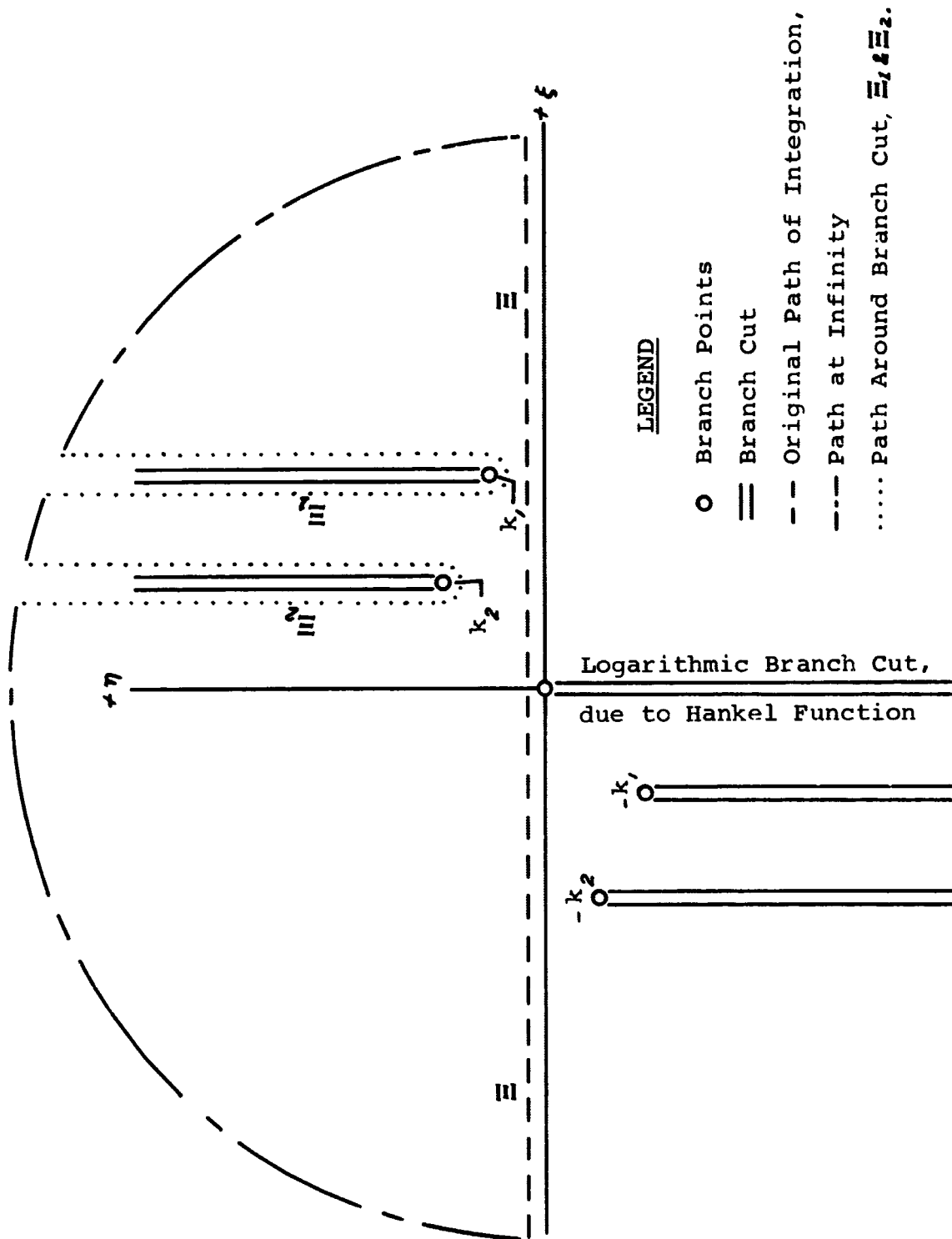
FIGURE 2.2. MAP OF \kappa PLANE BRANCH CUTS ASSOCIATED WITH +\kappa_2 AND H_0^1(\kappa r) AND THE PATHS OF INTEGRATION.
