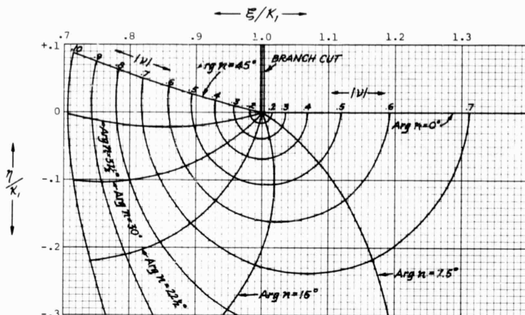
a) POLE LOCATION IS \frac{K}{K_1} PLANE AS A FUNCTION OF |V| AND \text{Arg } n, |n| = .5
