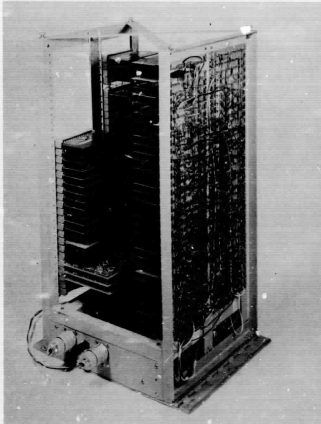
Figure 20. Electronics flight package
