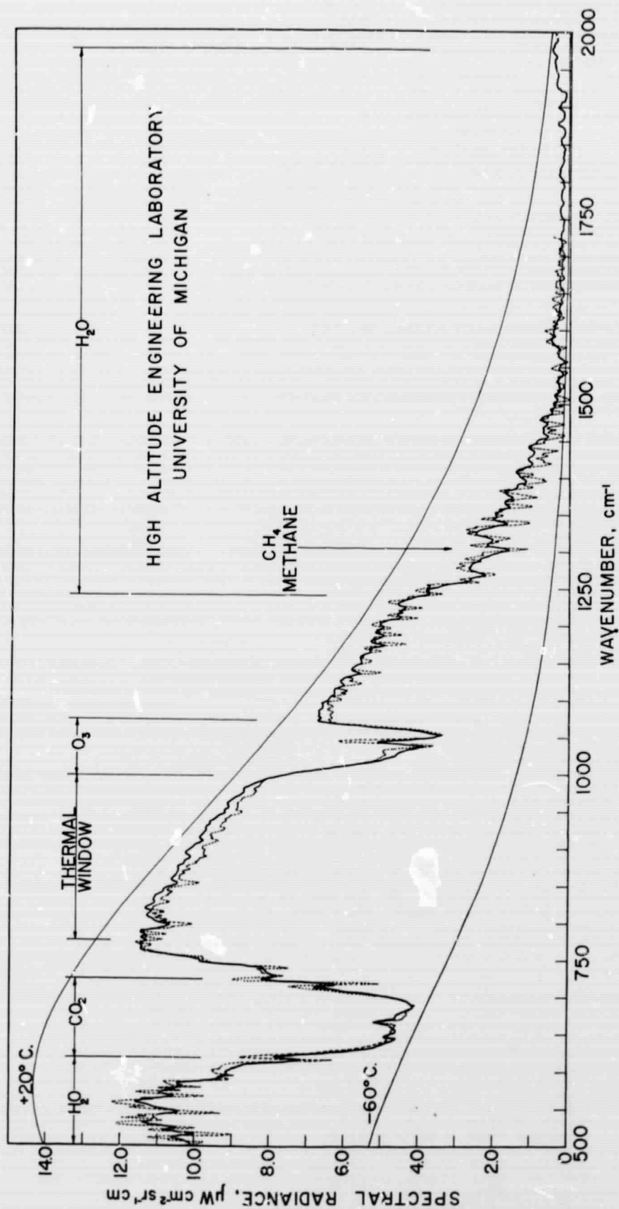
Figure 38. Spectra comparison
