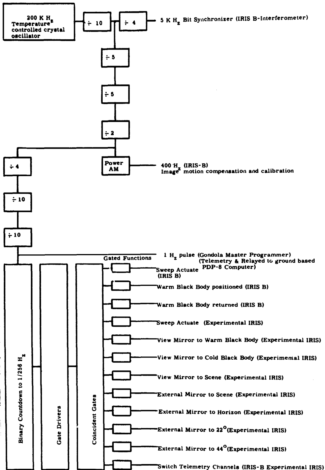
Figure 22 IRIS Control Block Diagram
