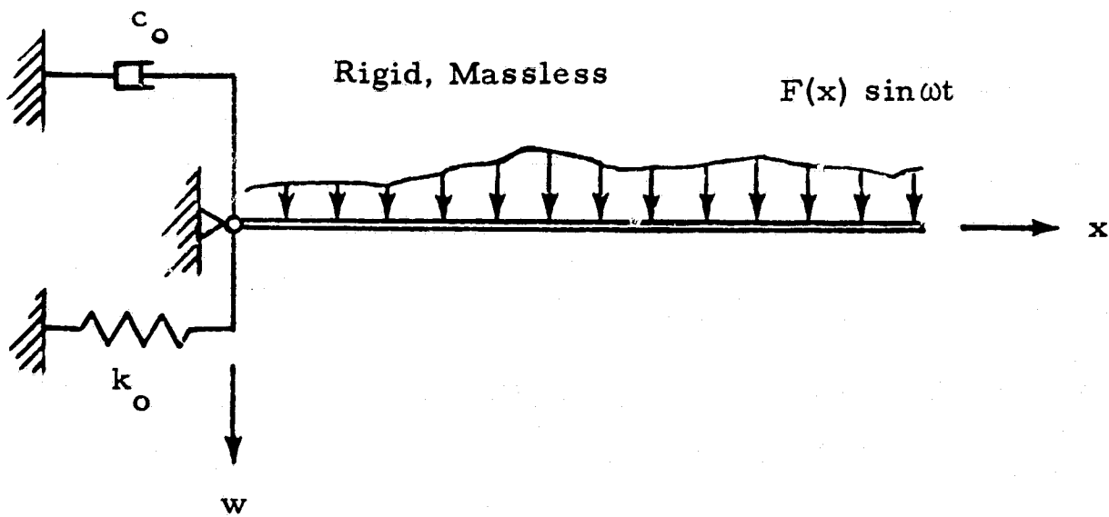
Fig.1 - Modeling of a Clamped Beam
