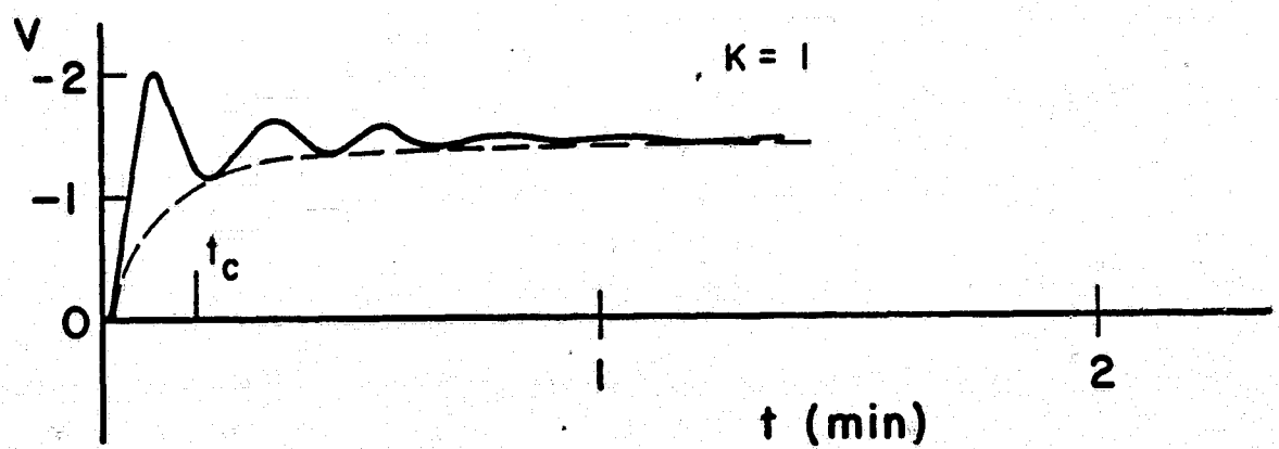
Figure 9. COMPUTER SOLUTION OF \dot{V} = -\frac{3}{50} (V + KV)^2 + E_0 , E_0 = 0.3 VOLT.
