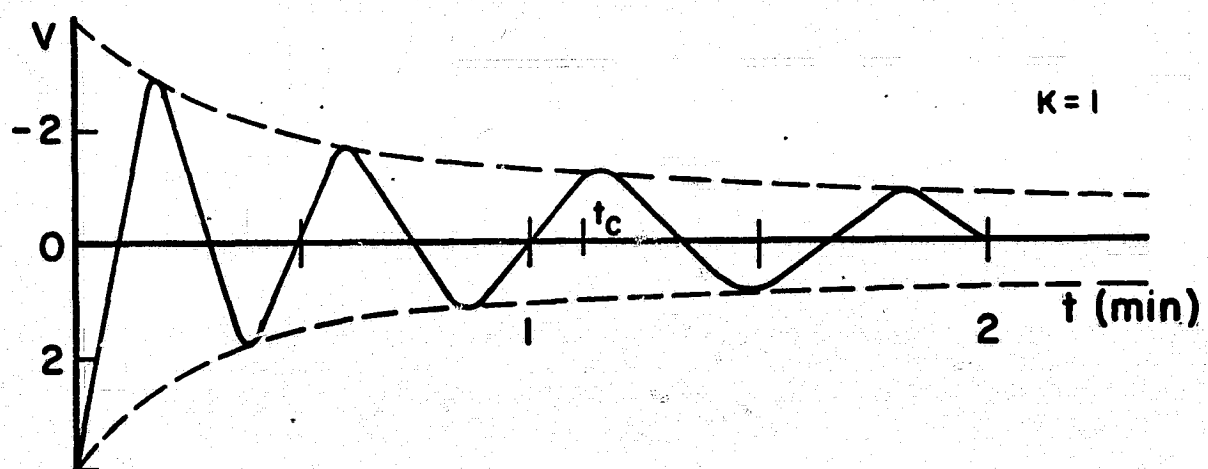
Figure 6. COMPUTER SOLUTION OF \dot{v} = -\frac{3}{50} (v + Kv)^2 , FOR K \leq 1 .
