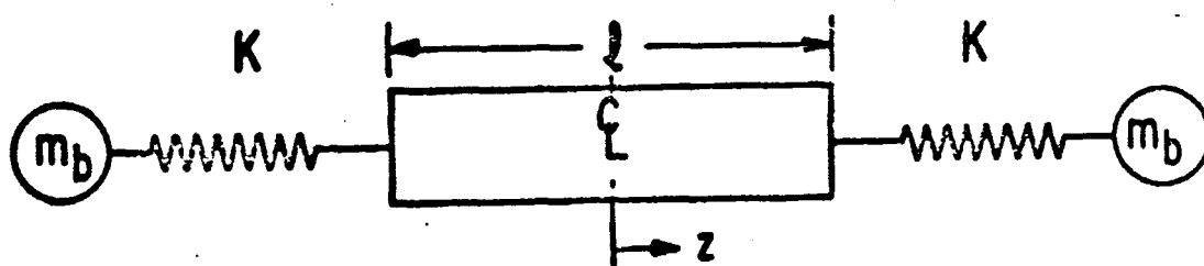
FIGURE 5. SCHEMATIC OF WAVE EXTENDER
