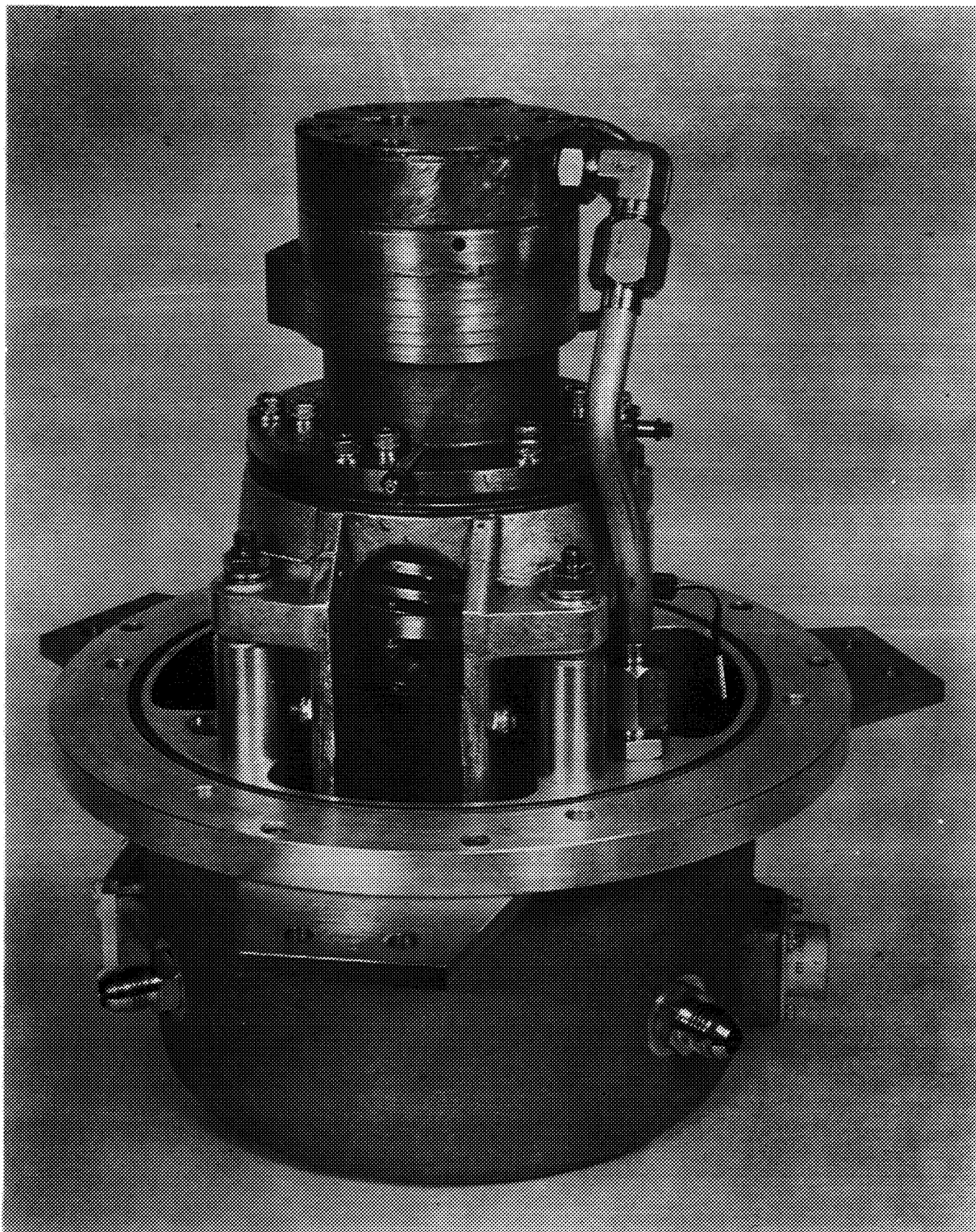
Fig. 4 View Showing Assembled Arrangement of the Improved Resonant Spring in the Improved Compressor of Contract NAS 8-20720.
