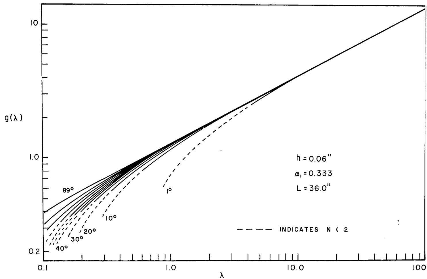
FIGURE 3.17 NORMALIZED EIGENVALUE DENSITY VERSUS \lambda WITH \psi AS THE PARAMETER FOR FREQUENCY EQUATION TWO
