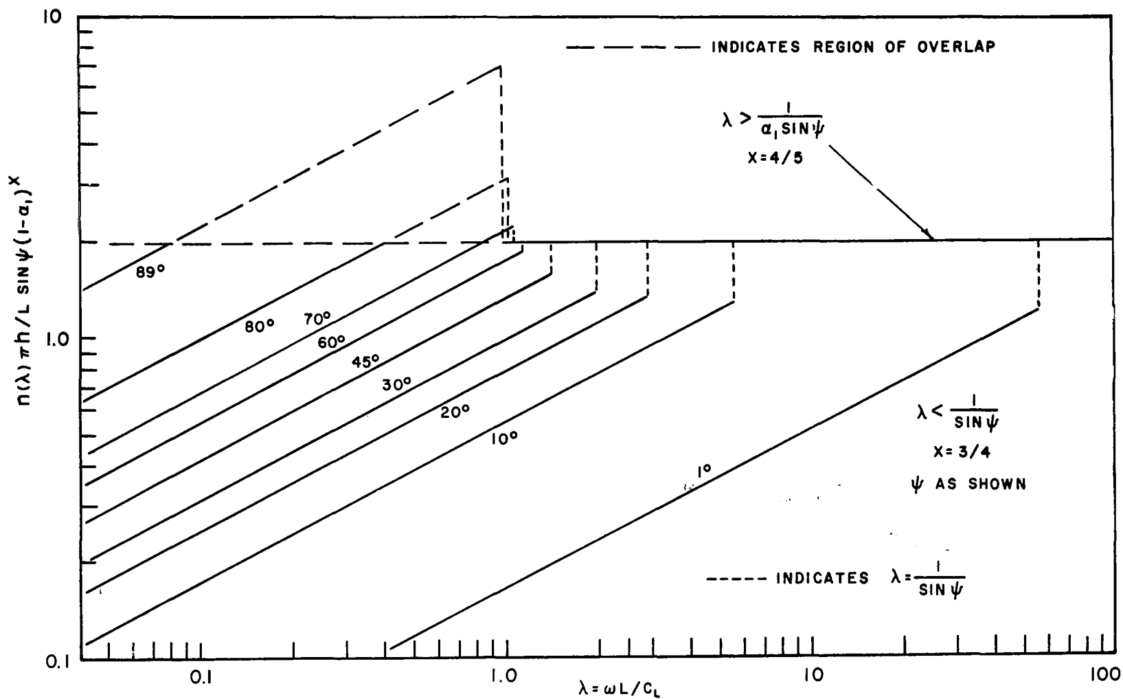
FIGURE 3.21 THEORETICAL EIGENVALUE DENSITY CURVES
