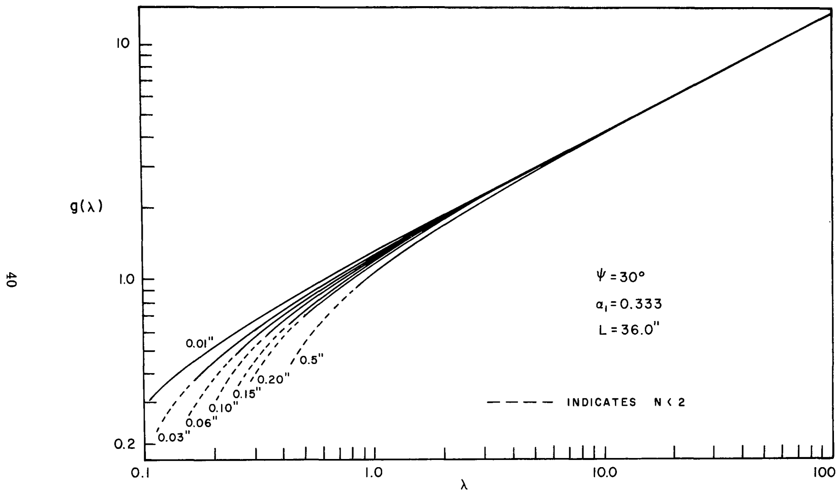
FIGURE 3.18 NORMALIZED EIGENVALUE DENSITY VERSUS \lambda WITH h AS THE PARAMETER FOR FREQUENCY EQUATION TWO
