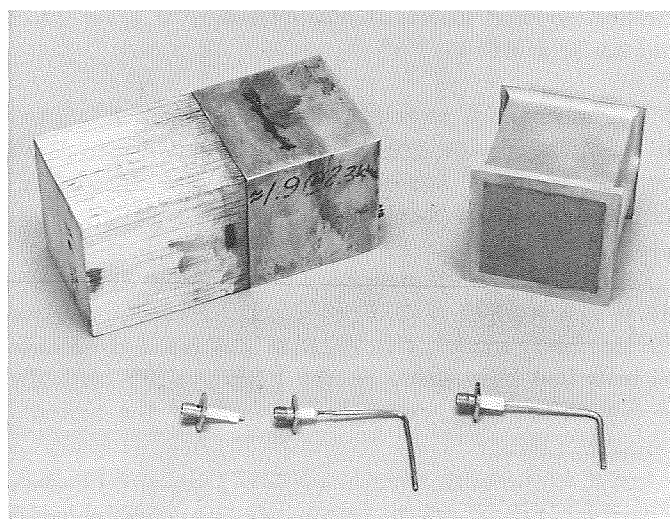
Fig. 12. Antenna and probe
