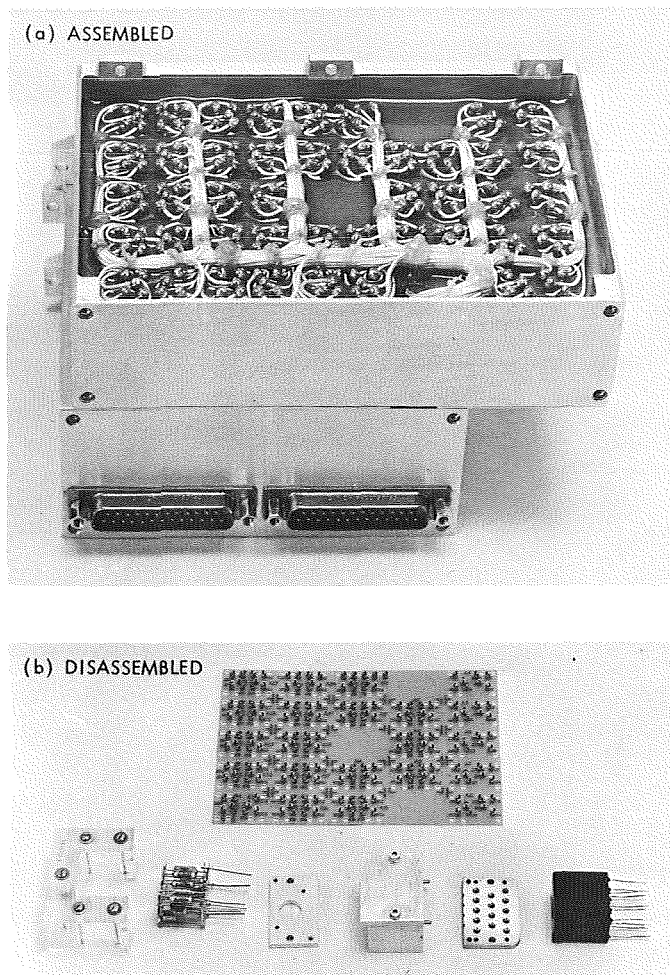
Fig. 15. Sequencer and timer
