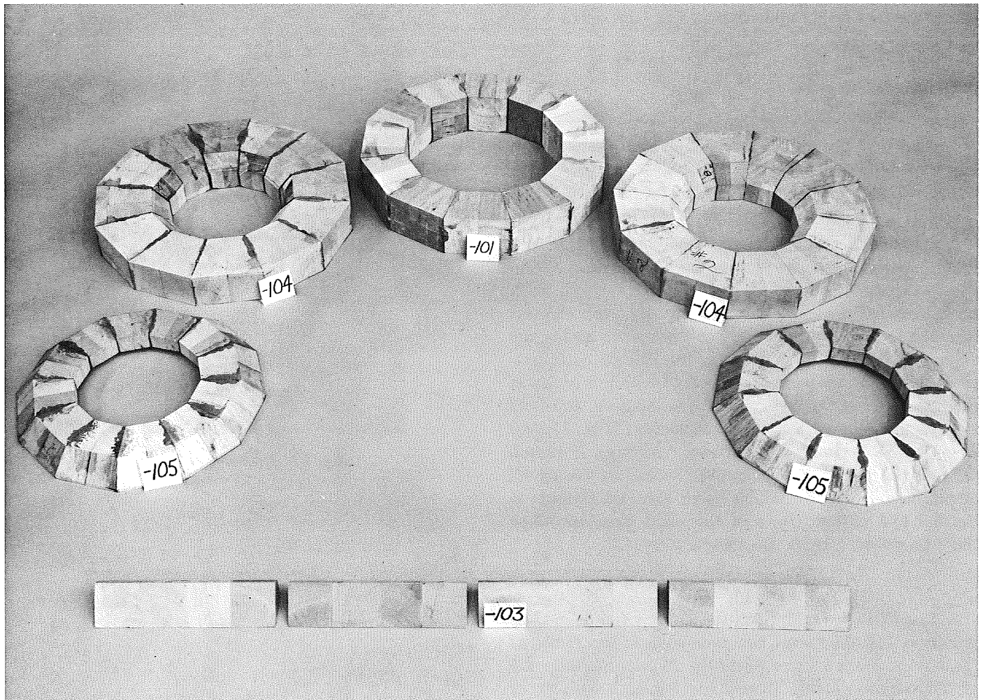
Fig. 19. Balsa impact limiter before assembly
