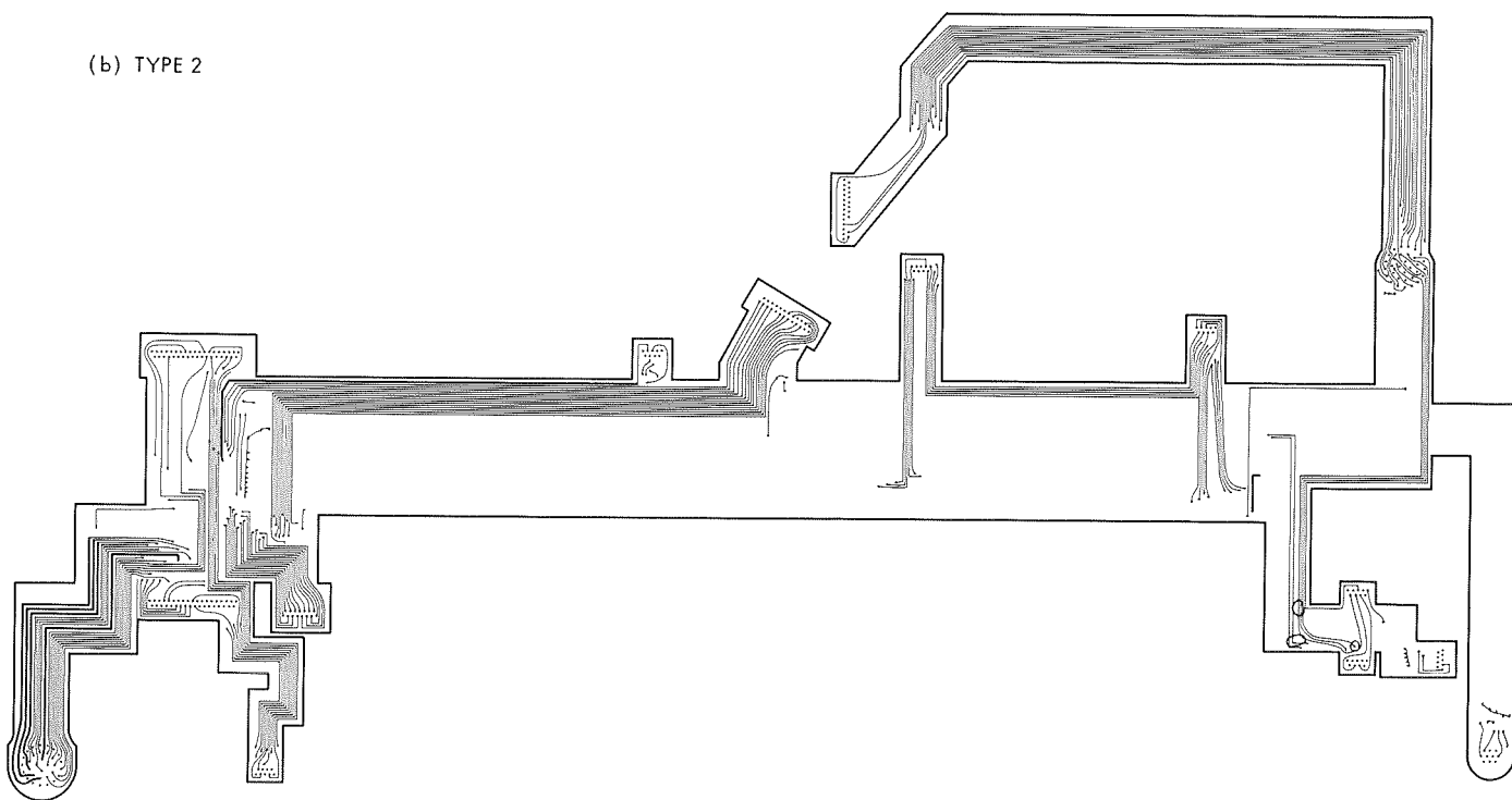
Fig. 10. Flexible harness
