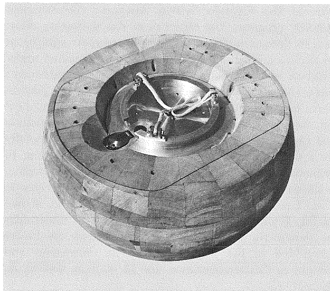
Fig. 3. Lander assembled in balsa impact limiter
