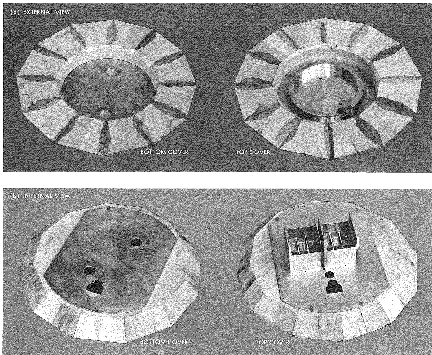
Fig. 21. Balsa cover assembly
