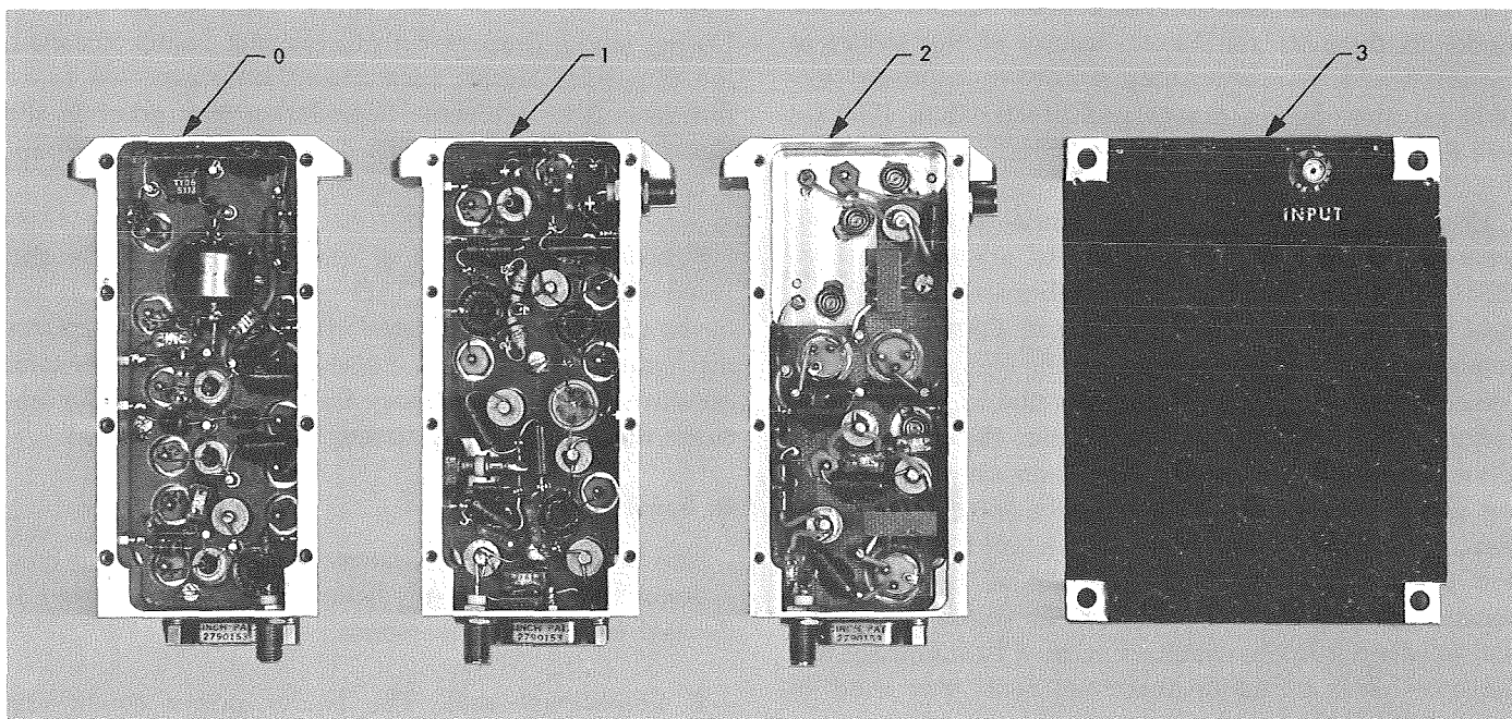
Fig. 11. Lander 5-W transmitter (modules 0-3)
