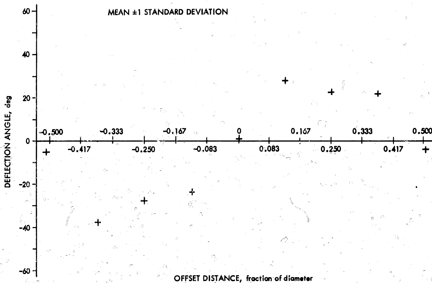
Figure 21. Crater Deflection Data, 47-ft Diameter, d/D Ratio 1:4.3
