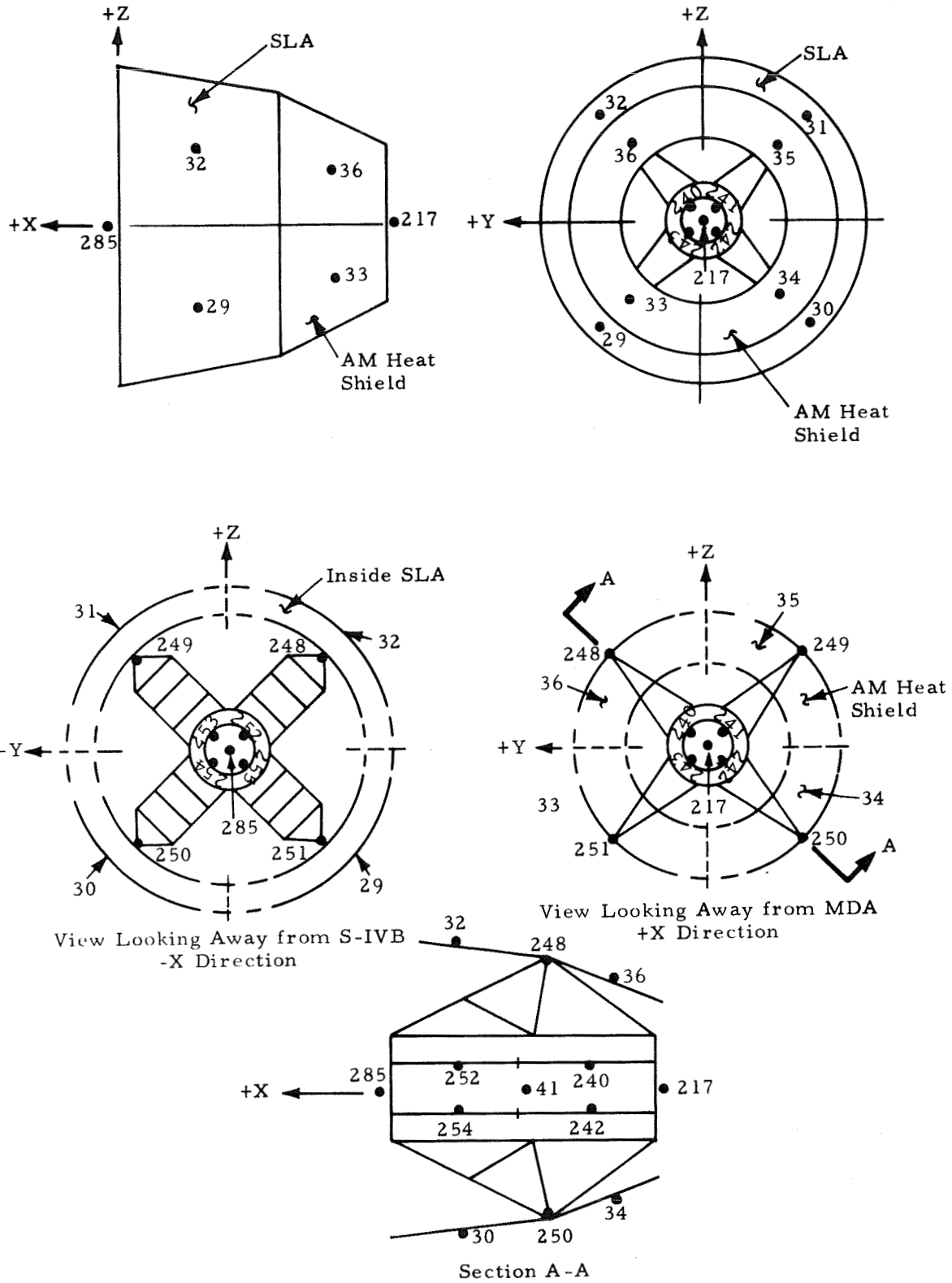
Figure 24 - AAP Cluster SLA and AM Nodal Network
