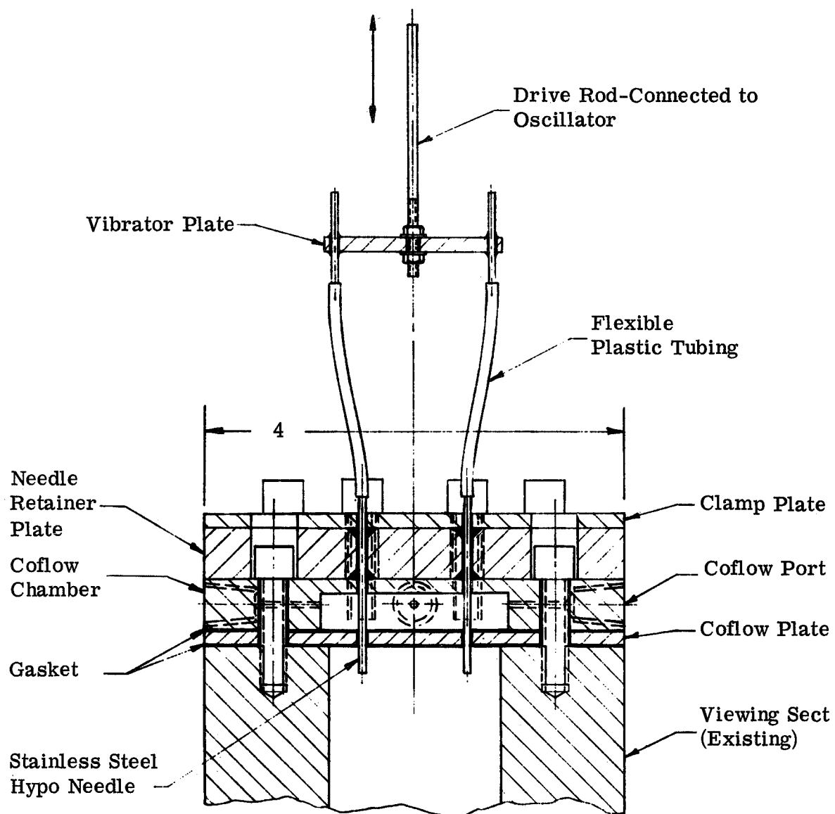
Figure 6. Drop Generator Head Detail.
