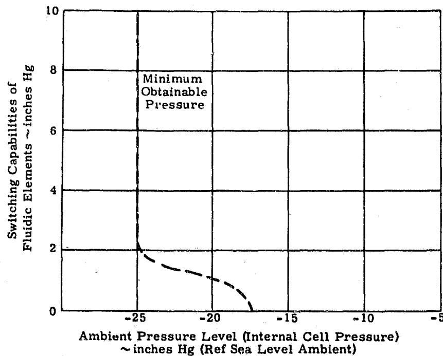
Figure 5. Maximum Switching Capabilities versus Internal Cell Pressure
