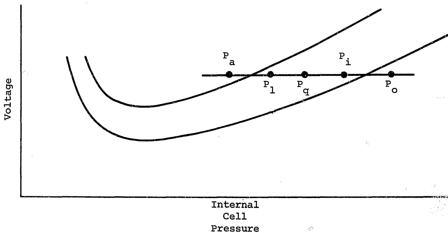
Figure 8. Pressure Levels versus Voltage
