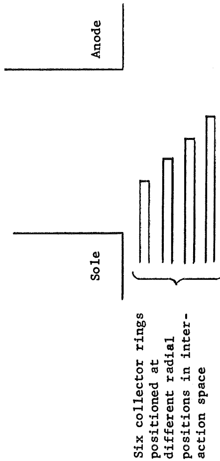
b. End view of interaction space showing positioning of collectors
