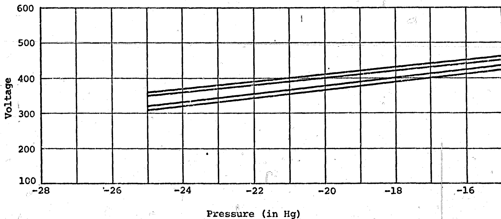
Figure 25. Cell Voltage-Pressure Relationship
