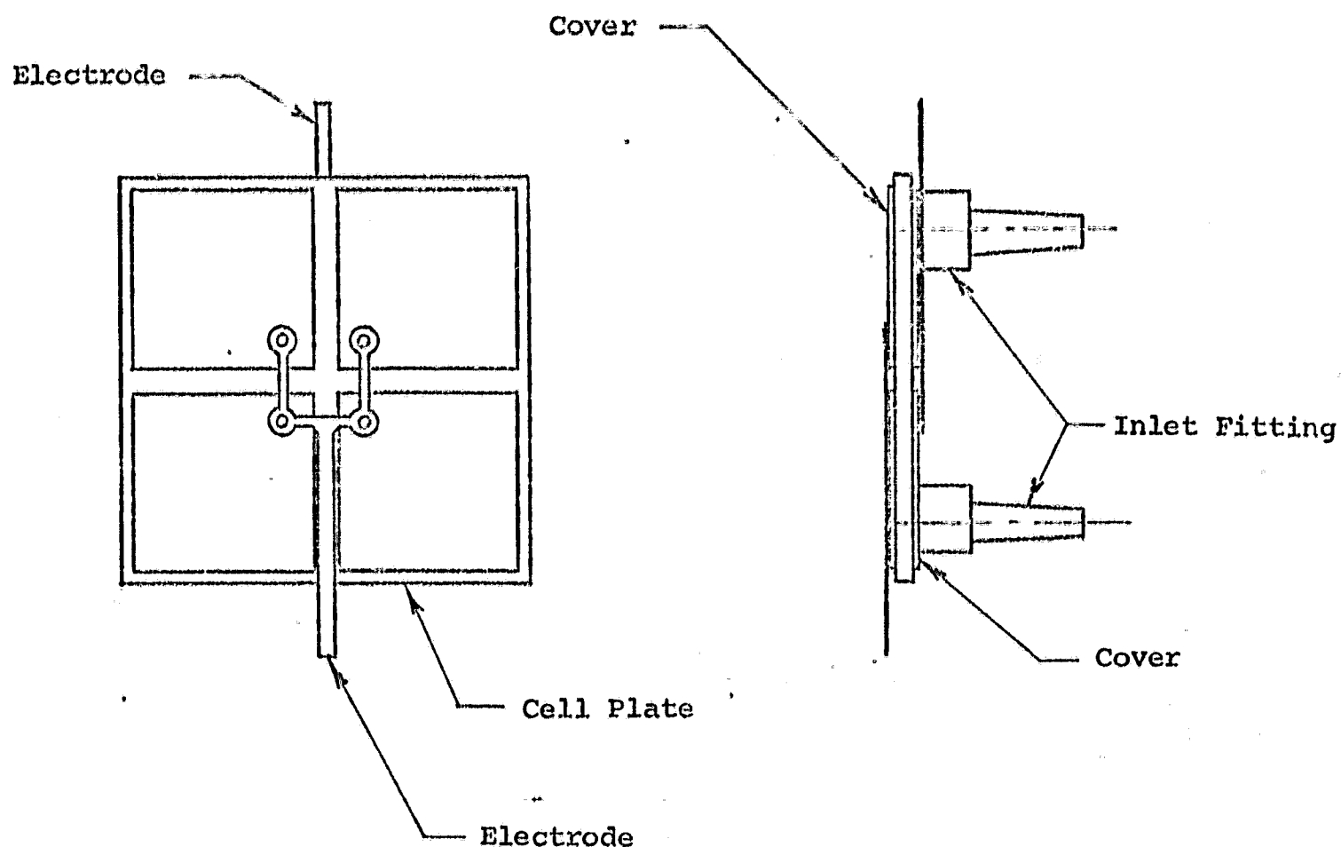
Figure 31. Plasma Cell Matrix
