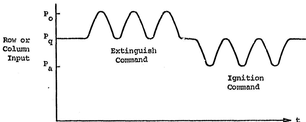
Figure 13. Oscillatory Control
