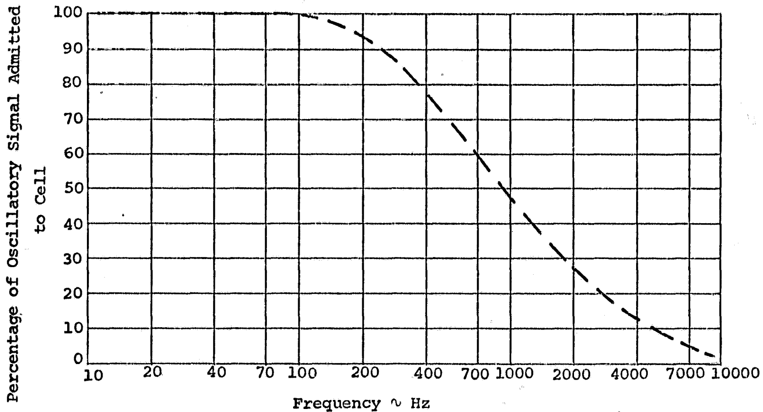
Figure 18. Control Signal Levels
