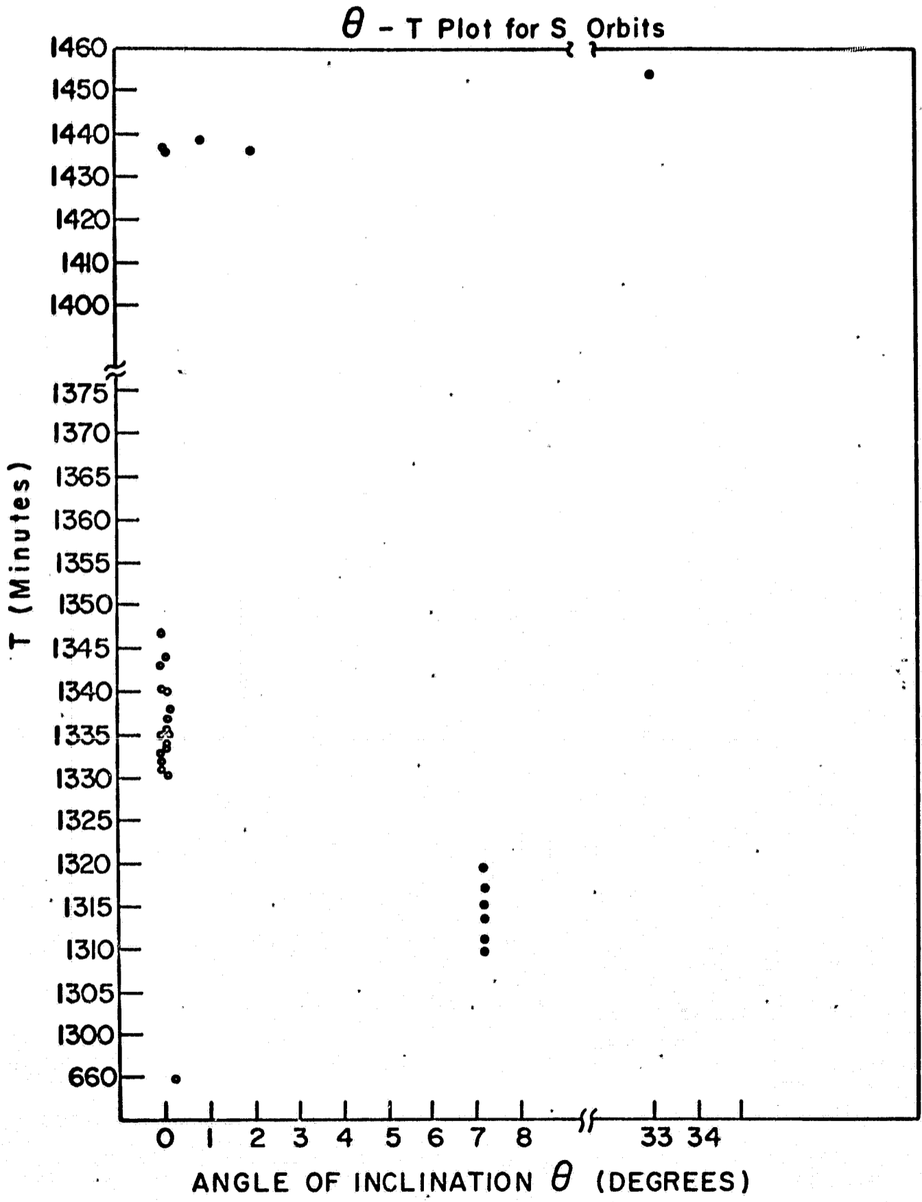
Fig. 5. Angle of Inclination vs. Period for S Flights
