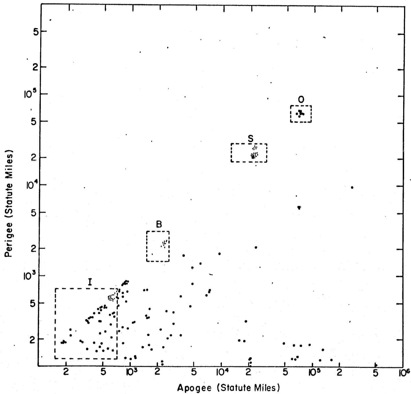
Fig. 1. Perigee vs. Apogee for Class # 1 Flights
