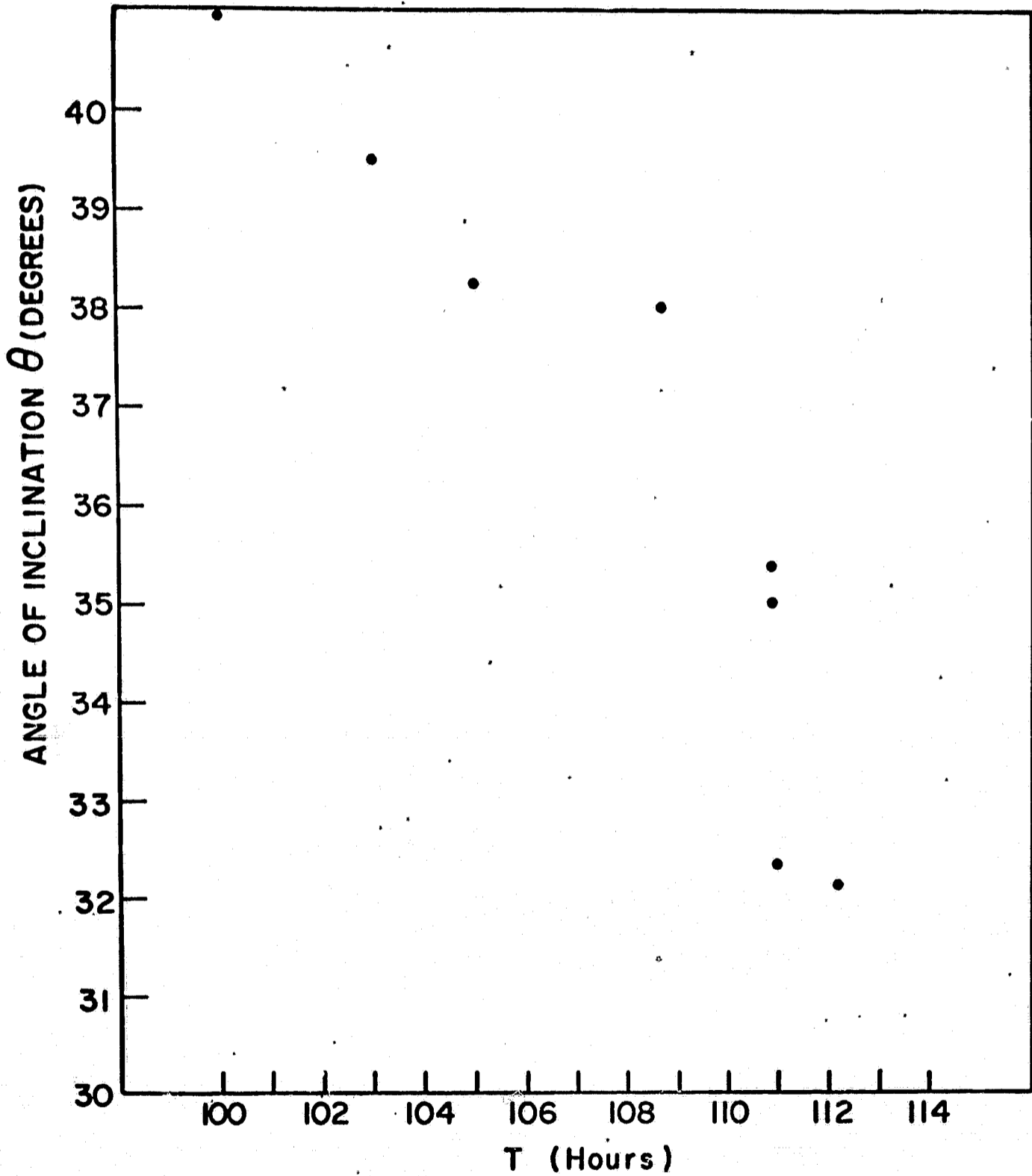
\theta - T Plot for O Orbits
