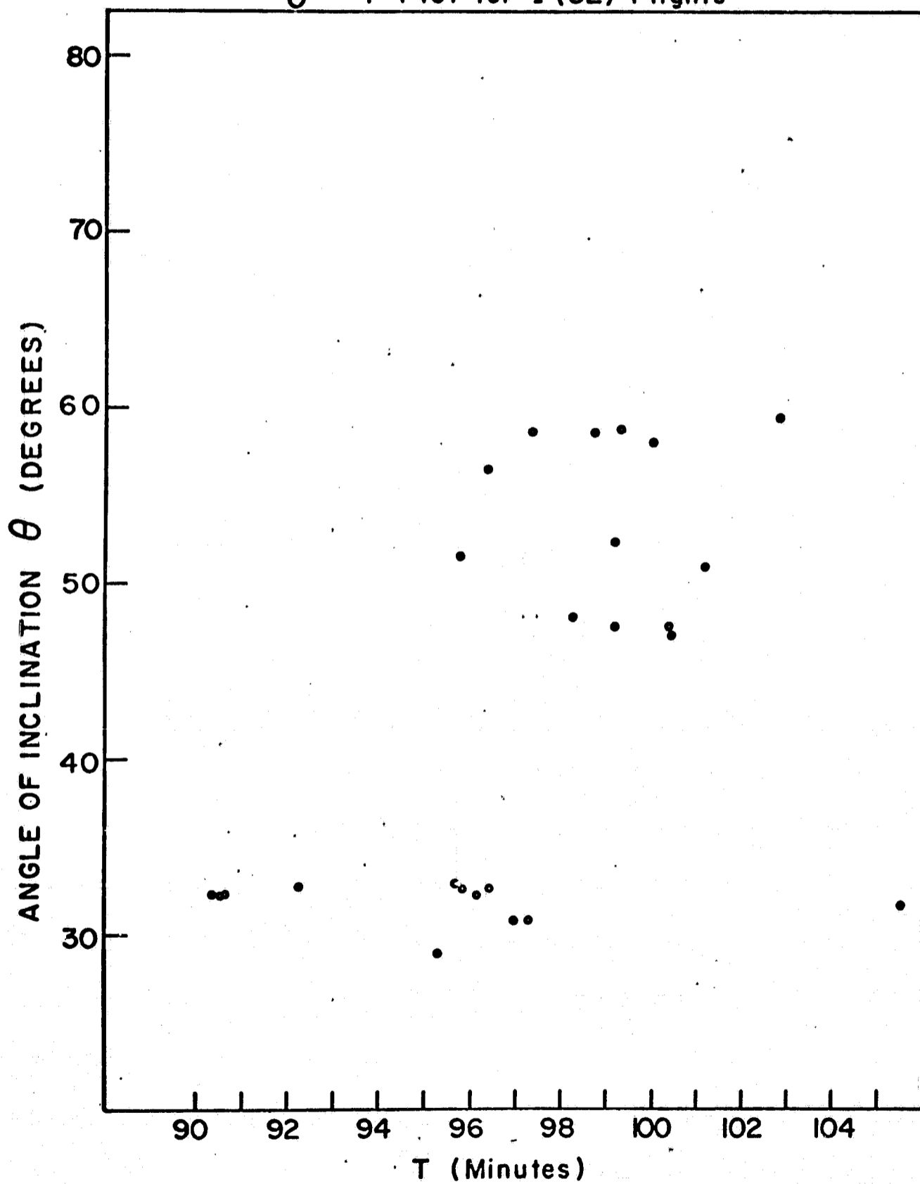
Fig. 2. Angle of Inclination vs. Period for I(55) and I(32) Flights
