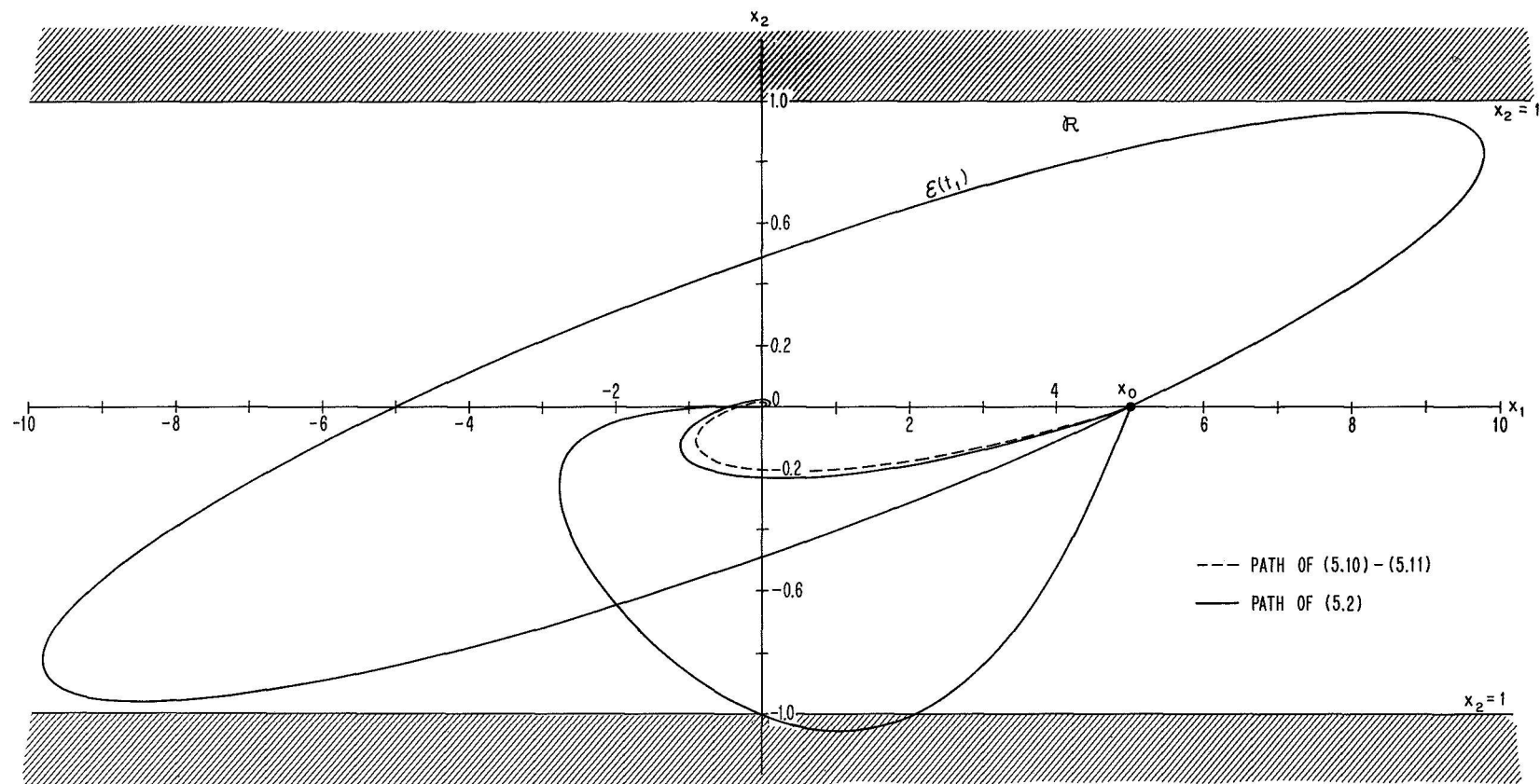
FIG. 7 REGION R , ELLIPSE E(t_1) , CONSTRAINED TRAJECTORIES OF (5.2), (5.10) - (5.11), AND AN UNCONSTRAINED TRAJECTORY OF (5.2).
