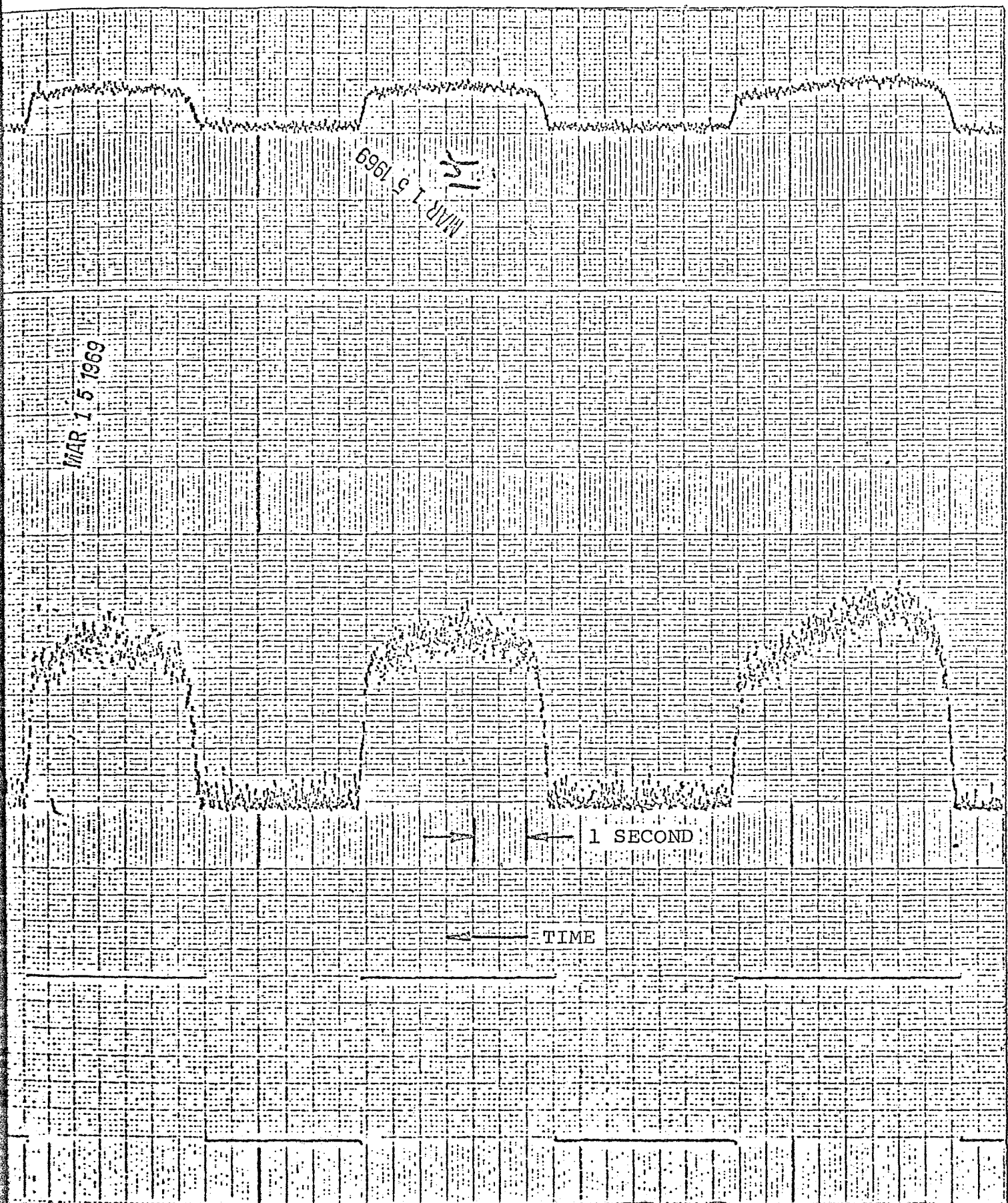
Figure 15. System Response to \text{CO}_2 during Inhale and Exhale Cycling.
