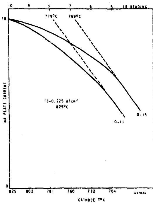
Figure 13 Diodes O-7/11/14/15 - Oxide-Coated Cathode Dip Test
