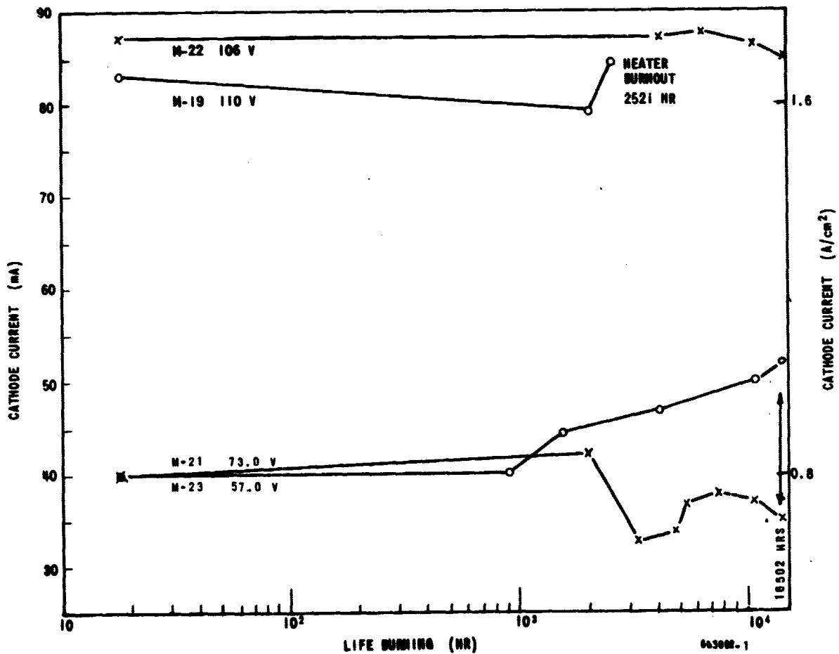
Figure 24. Pore-dispenser Cathode - T4 = 1100° C BR
