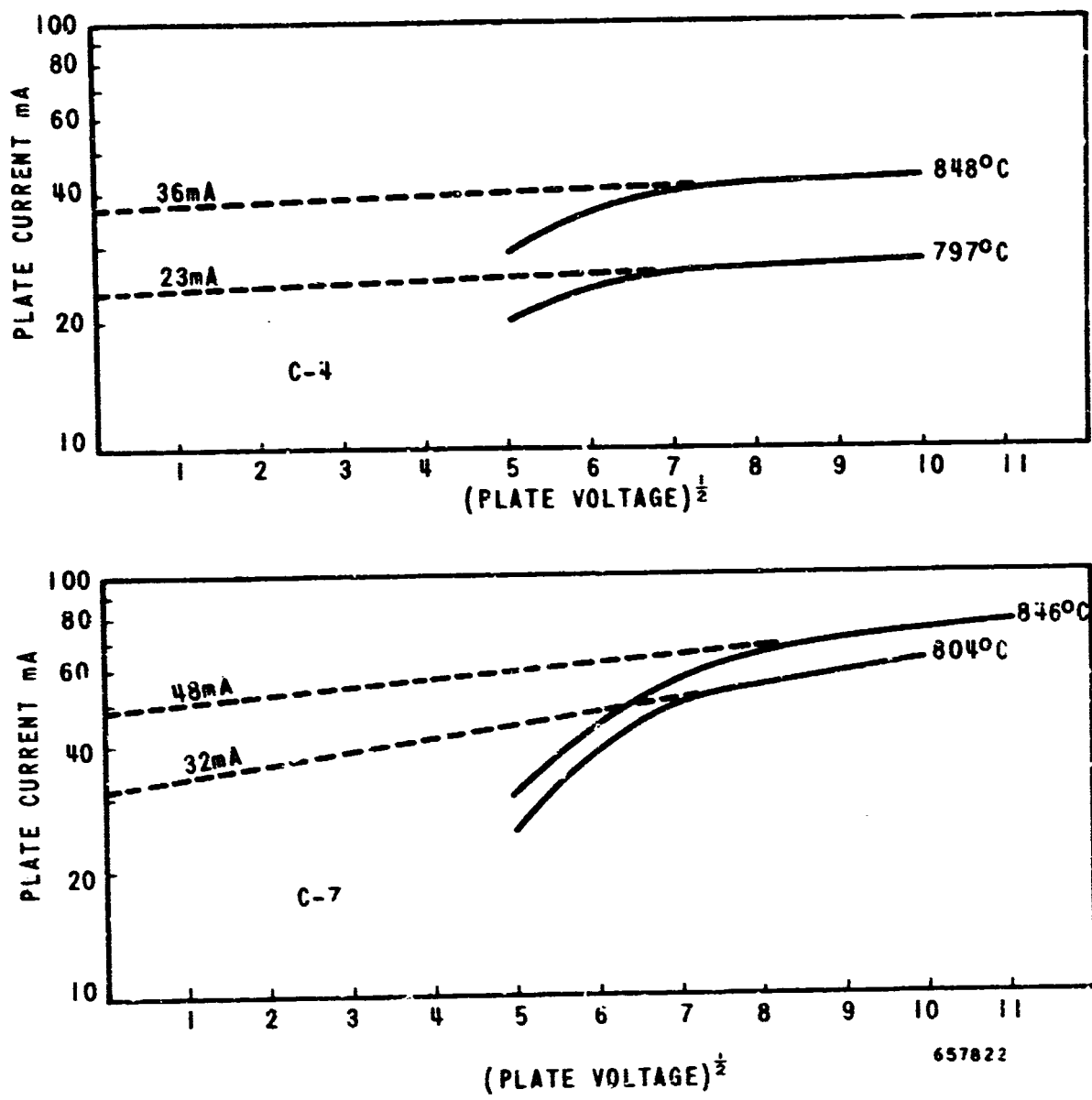
Figure 16 Diodes C-4/7 - Zero Field-Current Density Coated-Particle Cathodes
