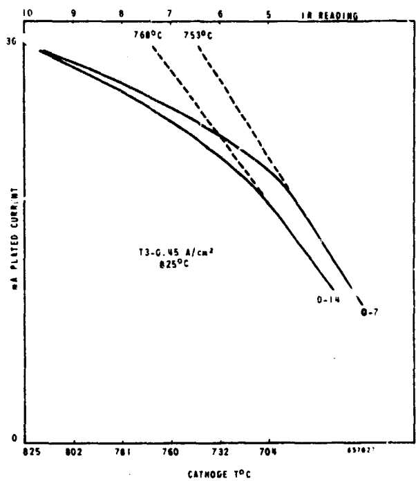
Figure 13 Diodes O-7/11/14/15 - Oxide-Coated Cathode Dip Test
