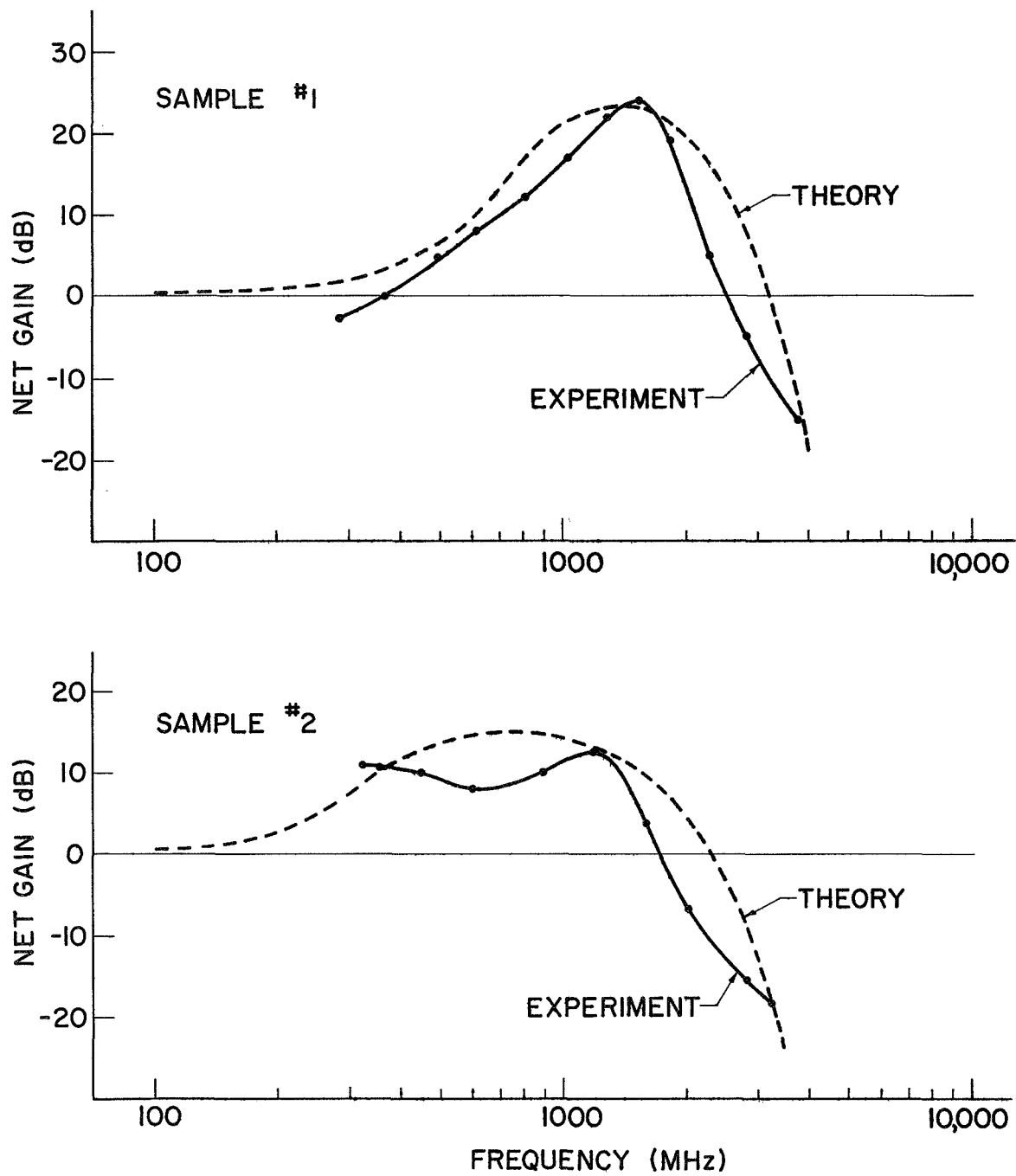
FIG. 4--Tuned terminal gain vs frequency.
