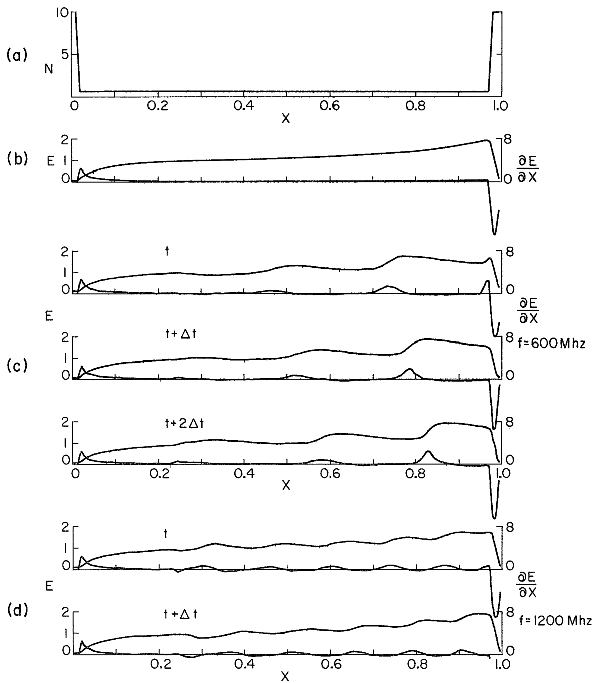
FIG. 5--Space charge wave field and charge distribution.
