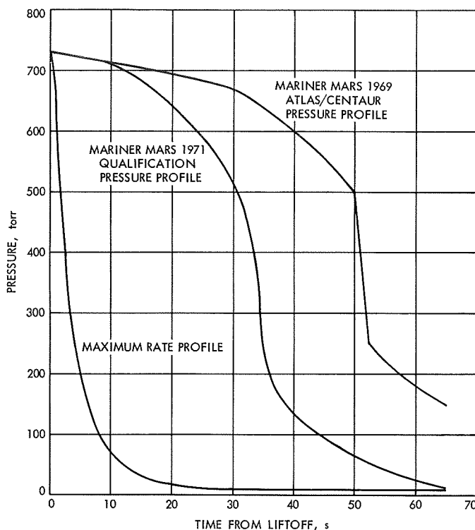
Fig. 8. Upper thermal blanket ballooning test pressure profiles
