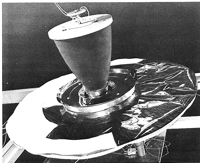
Fig. 9. Test fixture for rocket engine thermal blanket and shield
