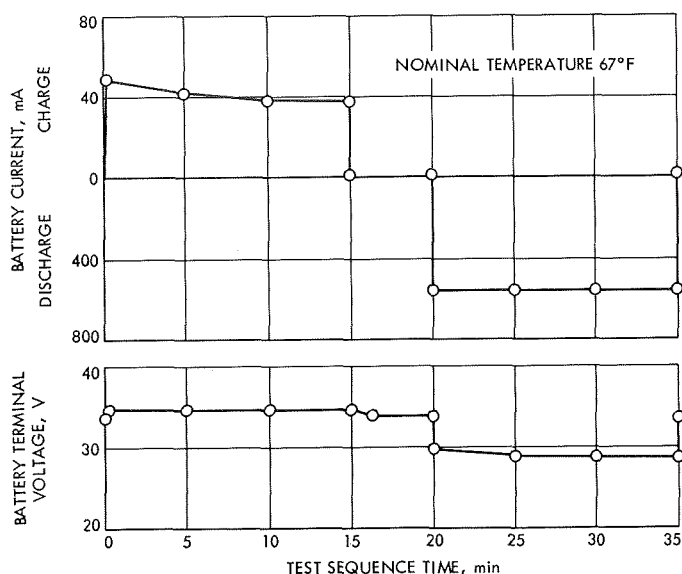
Fig. 1. Mariner VI battery current and voltage versus time test sequence
