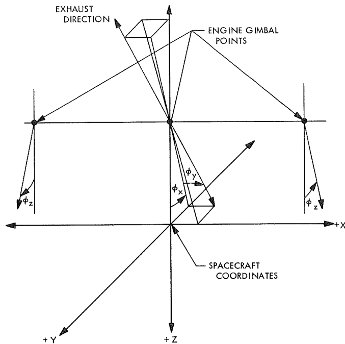
Fig. 7. Gimbal angle definition
