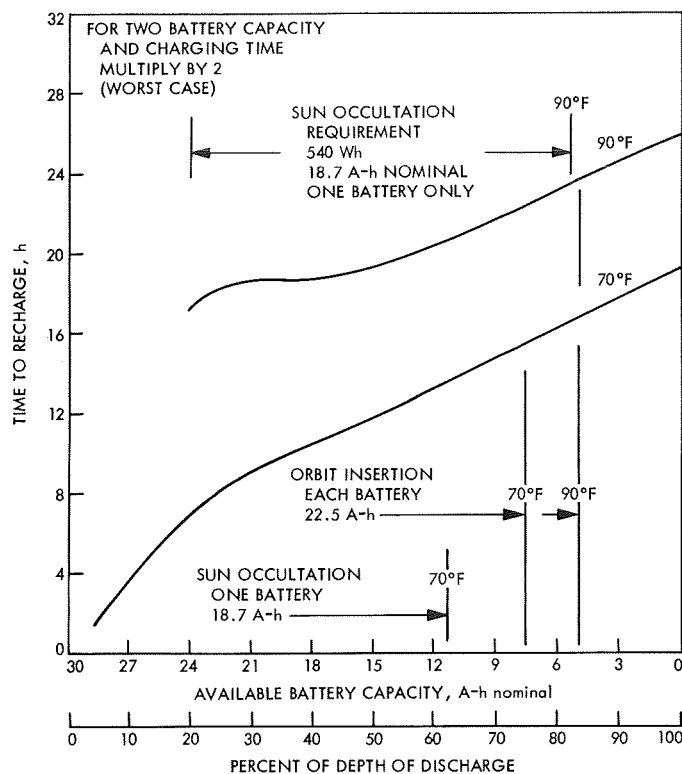
Fig. 6. Battery charging time at 70 and 90°F with C/15 charge rate
