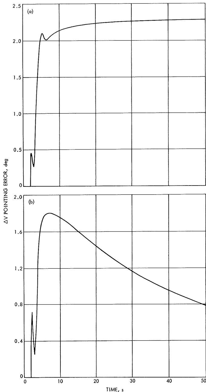
Fig. 9. \Delta V pointing error versus time: (a) no path guidance compensation, (b) with path guidance compensation
